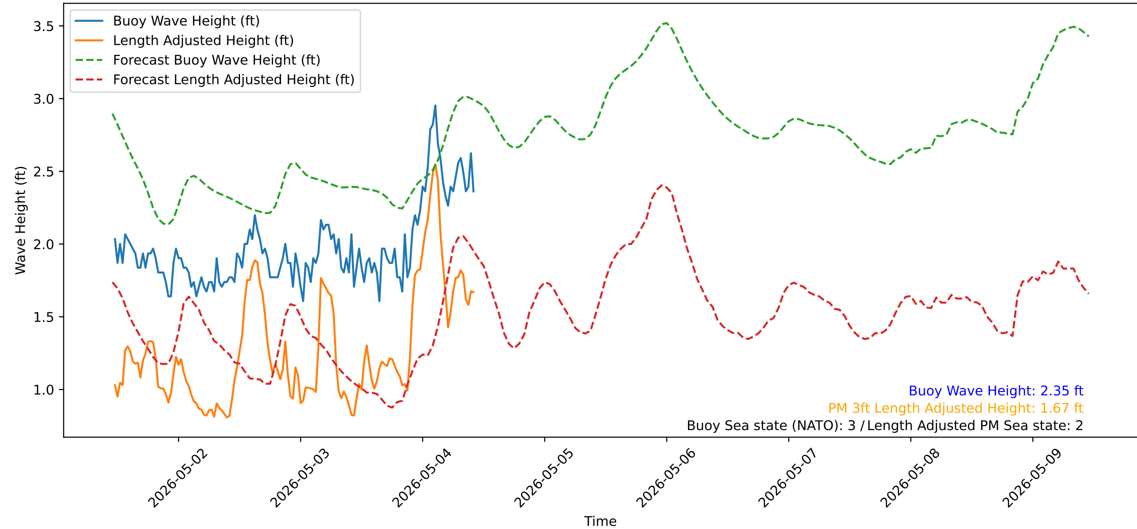
Wave Heights over Time for Red Beach at 2026-05-04 11:00:50
