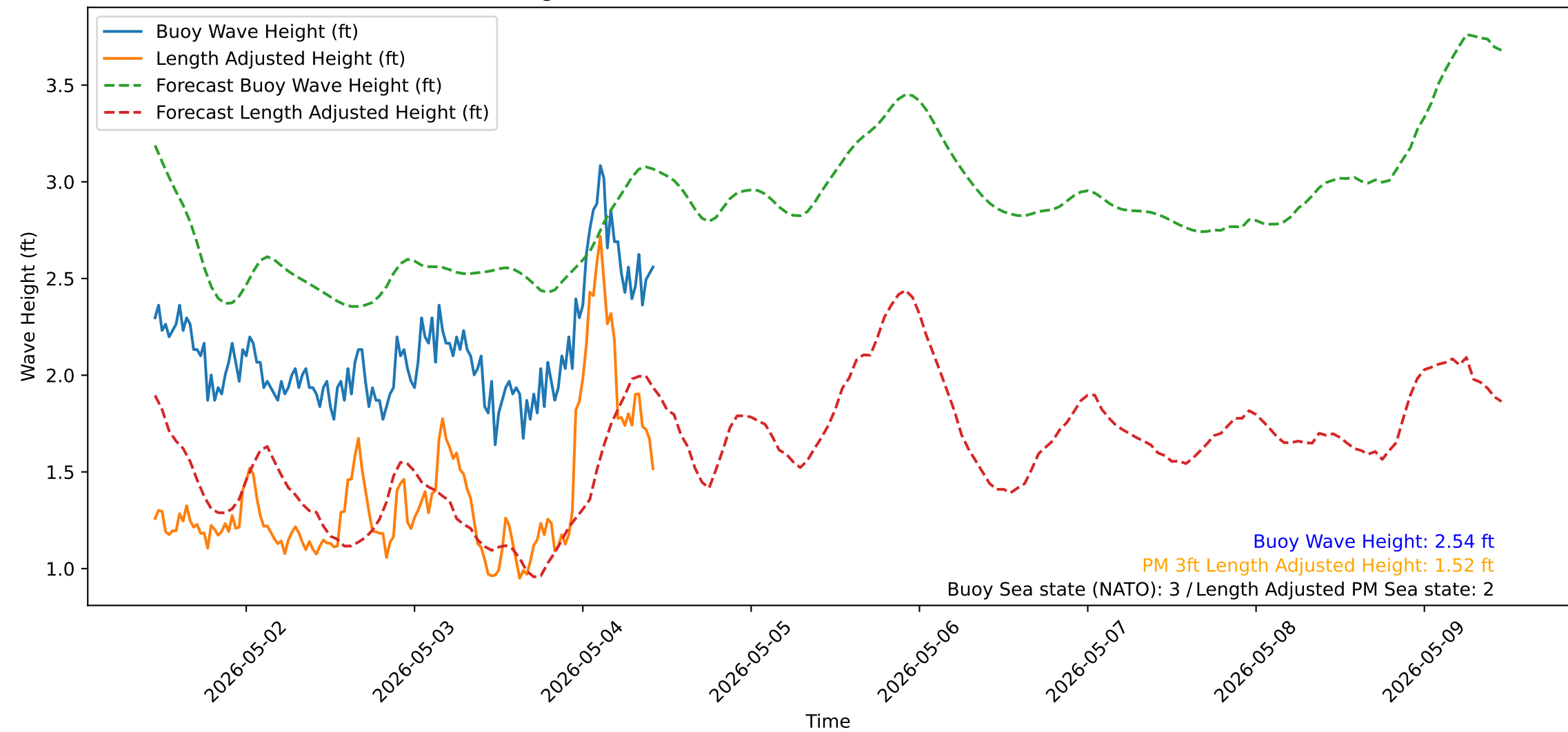
Wave Heights over Time for Oceanside Harbor at 2026-05-04 11:00:31
