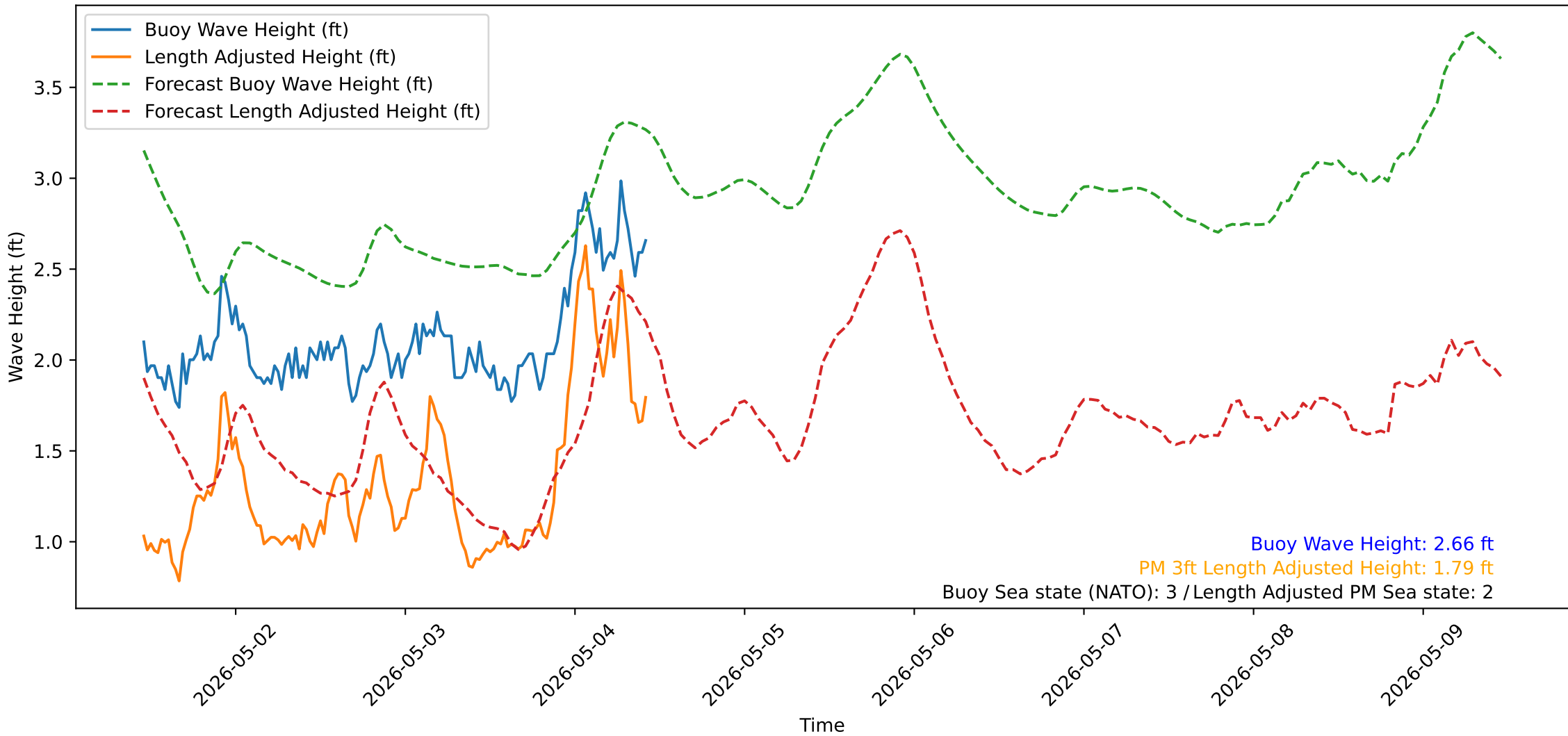
Wave Heights over Time for Green Beach at 2026-05-04 11:01:12
