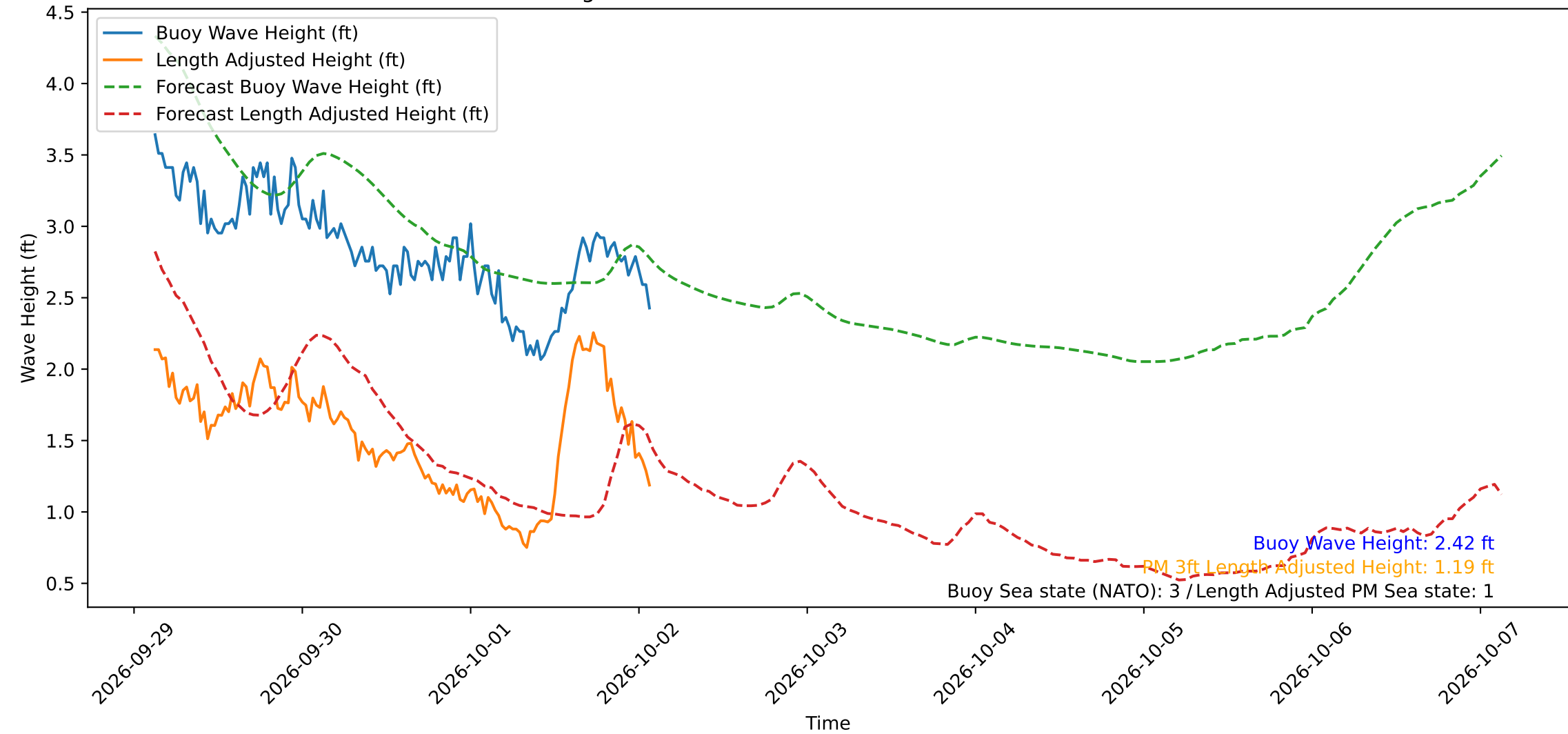
Wave Heights over Time for Red Beach at 2026-10-02 02:30:49
