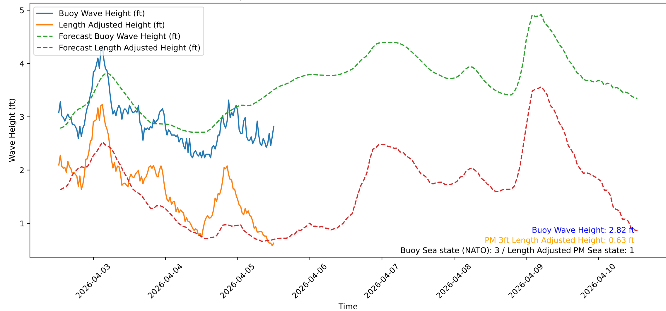
Wave Heights over Time for Green Beach at 2026-04-05 12:41:10
