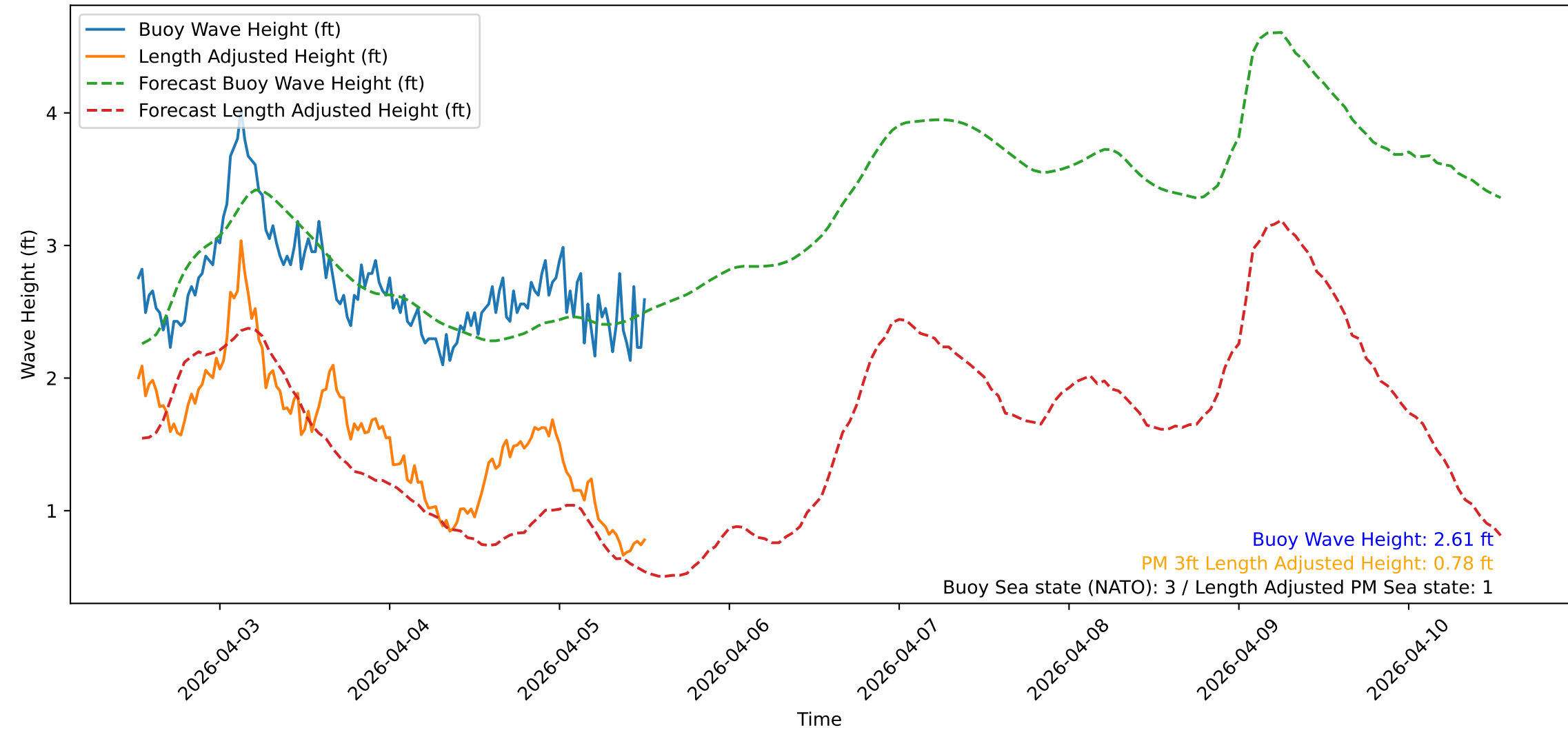
Wave Heights over Time for Oceanside Harbor at 2026-04-05 12:40:31
