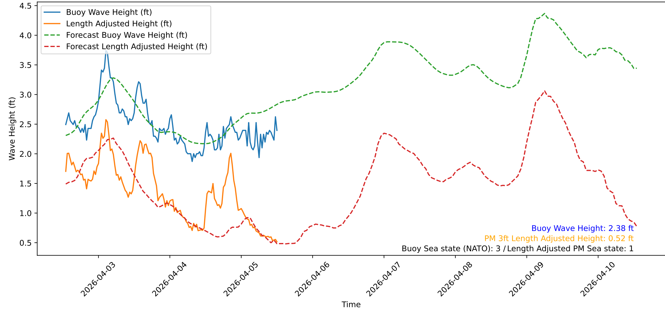
Wave Heights over Time for Red Beach at 2026-04-05 12:40:48
