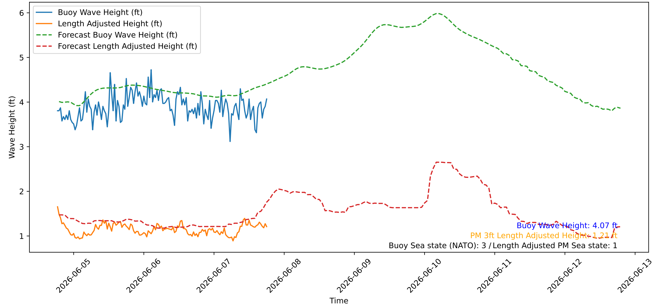
Wave Heights over Time for Green Beach at 2026-06-07 18:41:07
