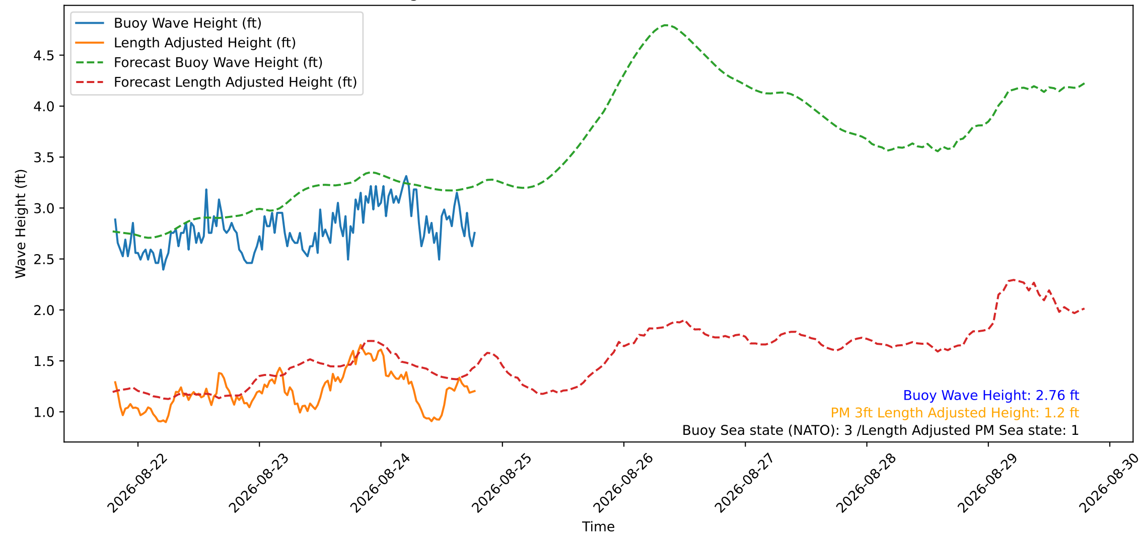
Wave Heights over Time for Green Beach at 2026-08-24 19:11:11
