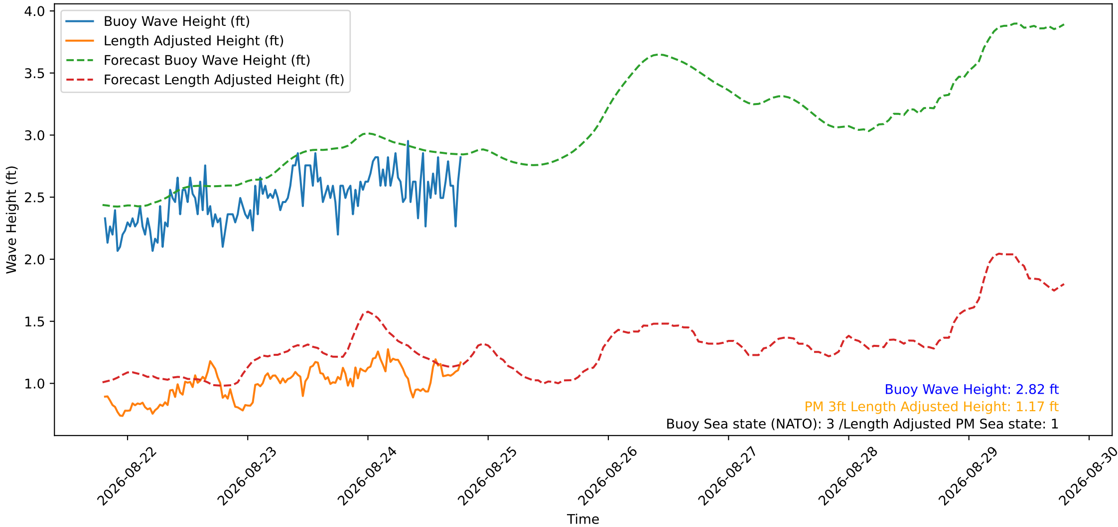
Wave Heights over Time for Red Beach at 2026-08-24 19:10:49
