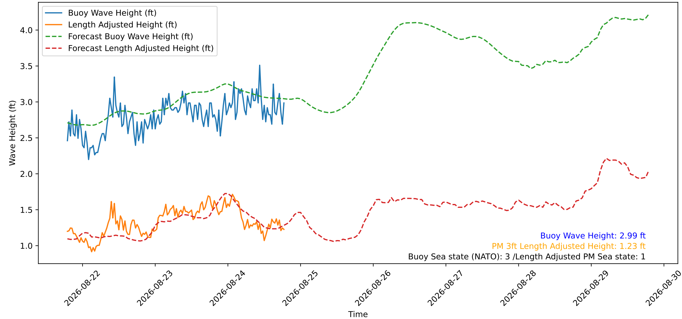
Wave Heights over Time for Oceanside Harbor at 2026-08-24 19:10:29
