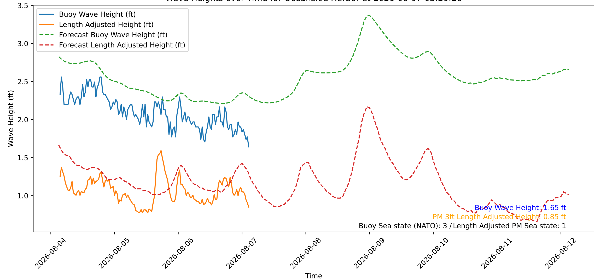
Wave Heights over Time for Oceanside Harbor at 2026-08-07 03:20:26
