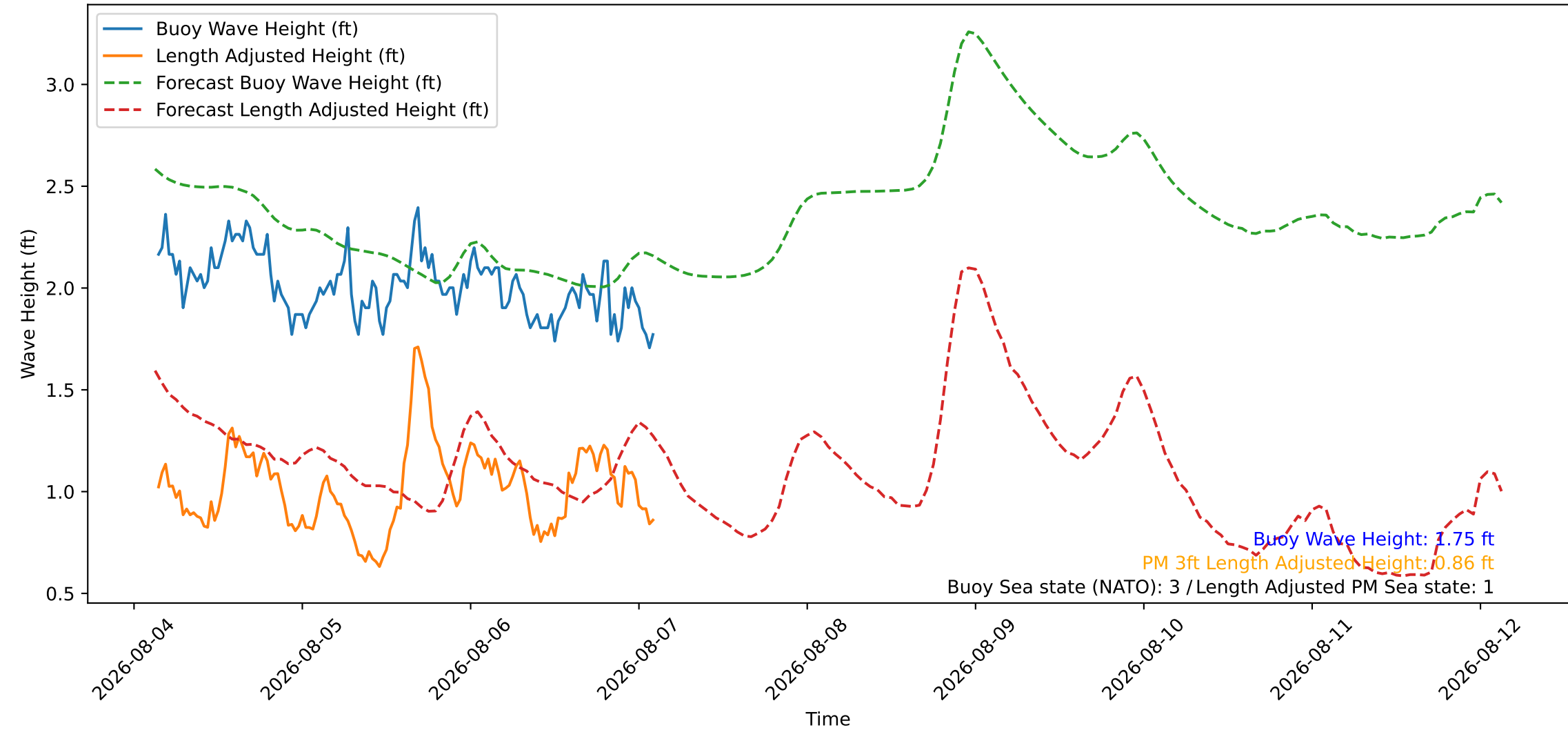
Wave Heights over Time for Red Beach at 2026-08-07 03:20:47
