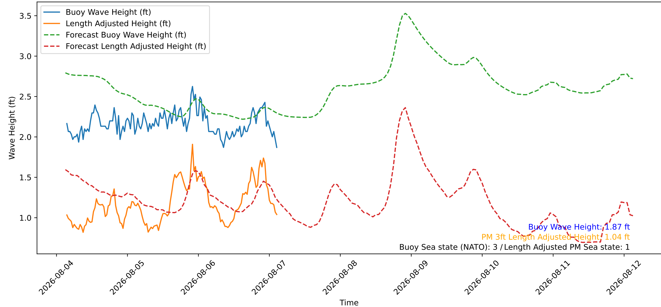
Wave Heights over Time for Green Beach at 2026-08-07 03:21:09
