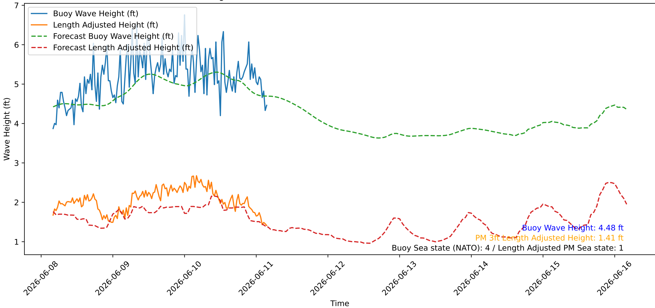
Wave Heights over Time for Oceanside Harbor at 2026-06-11 04:00:26
