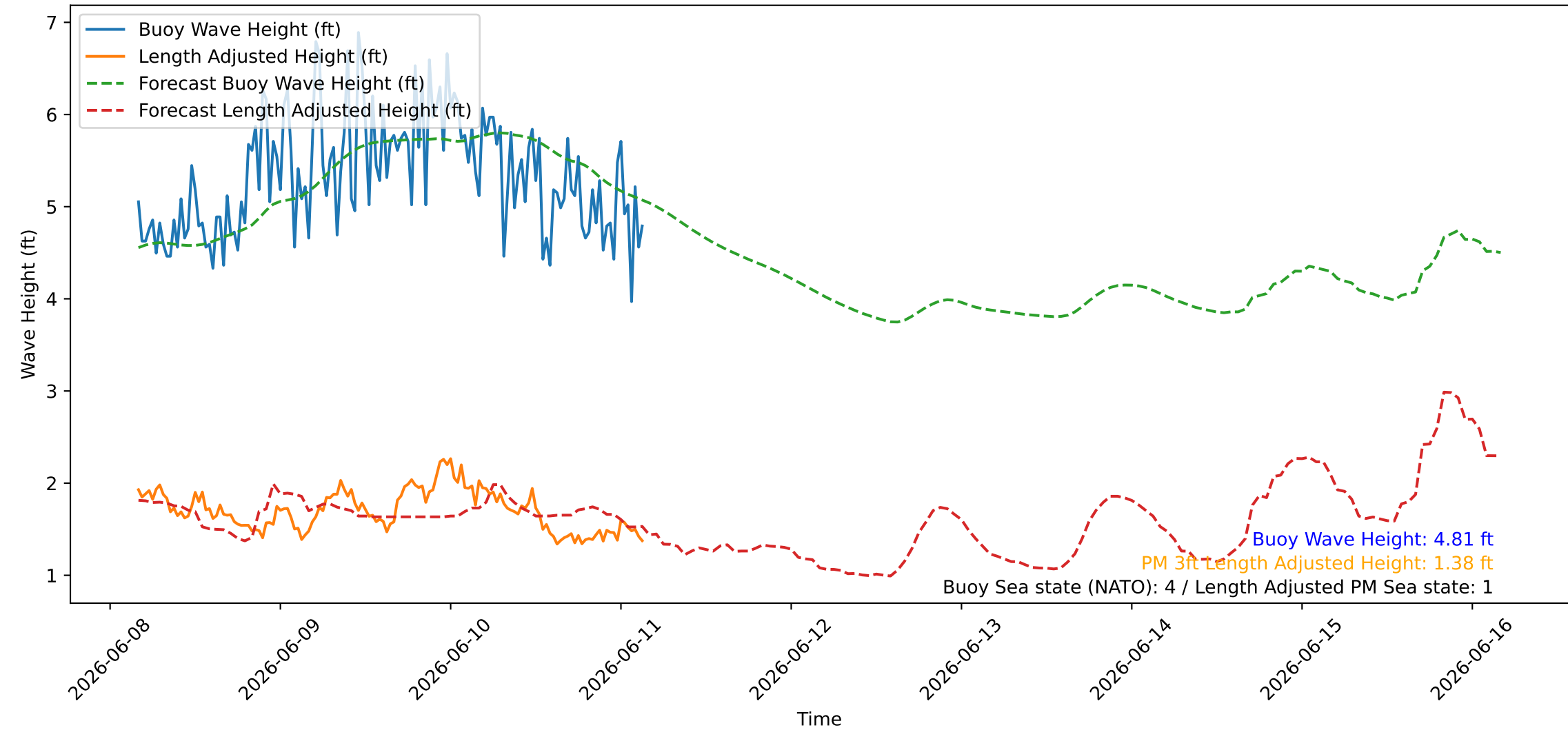
Wave Heights over Time for Green Beach at 2026-06-11 04:01:10
