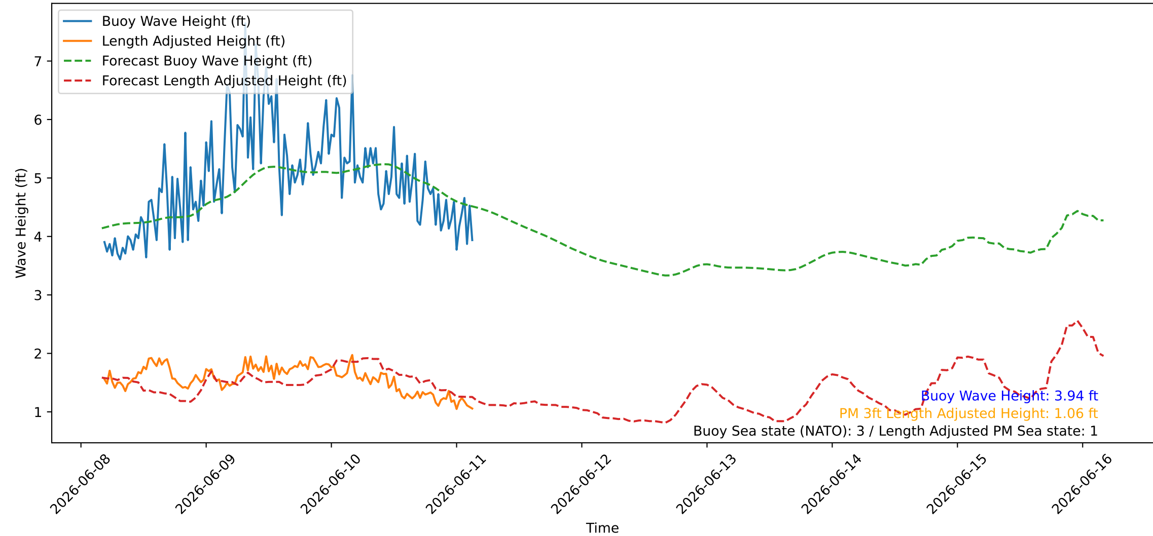
Wave Heights over Time for Red Beach at 2026-06-11 04:00:47
