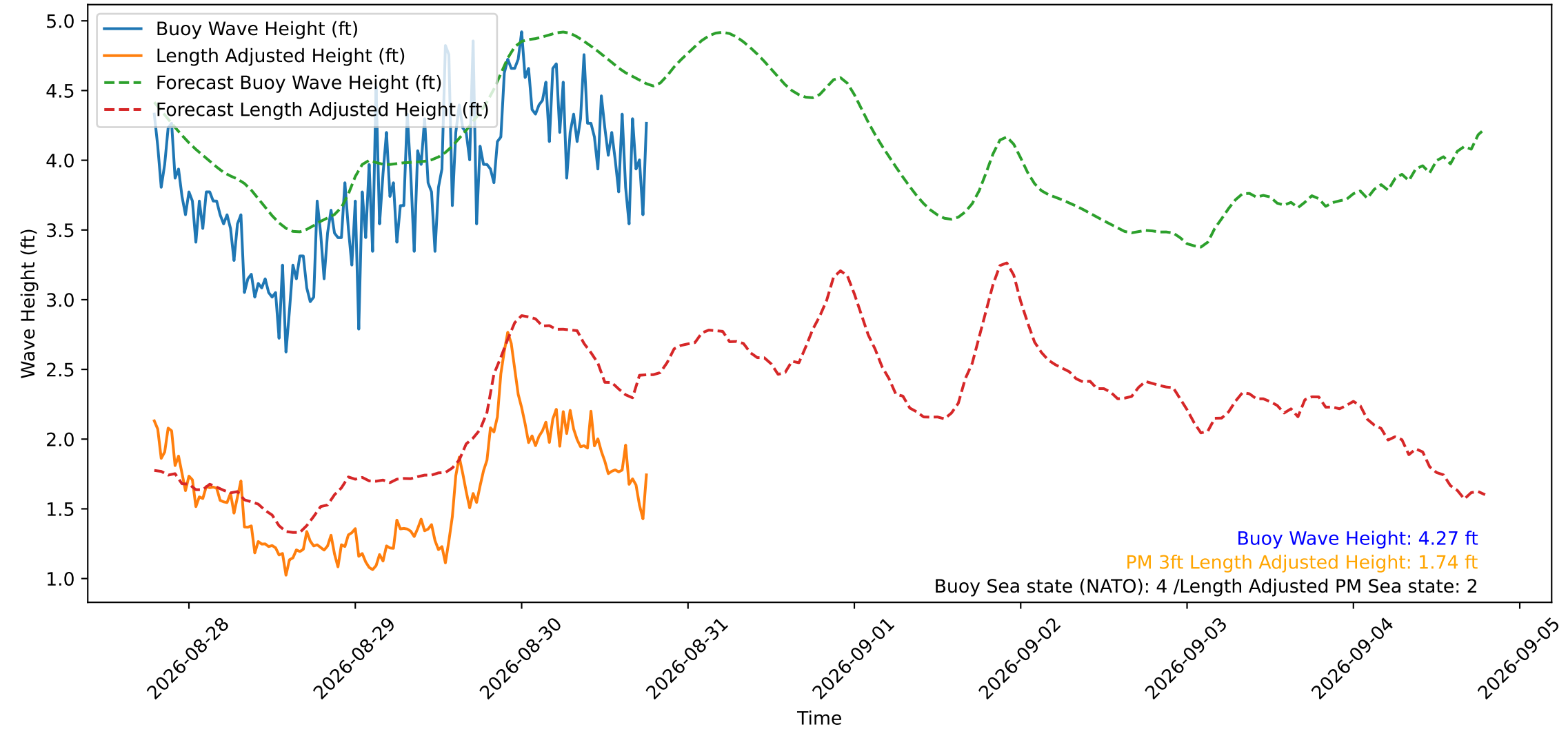
Wave Heights over Time for Green Beach at 2026-08-30 18:51:14
