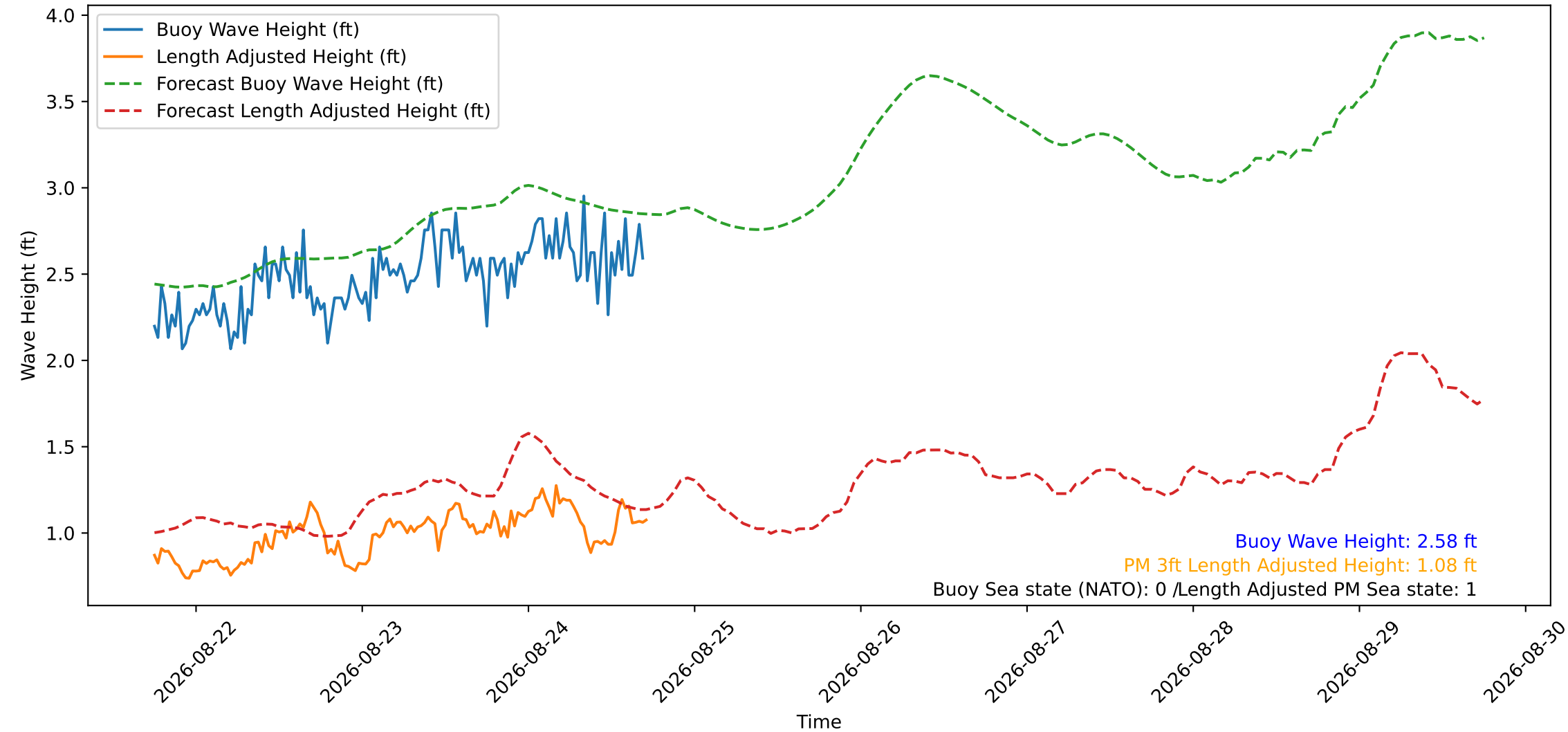
Wave Heights over Time for Red Beach at 2026-08-24 17:50:50
