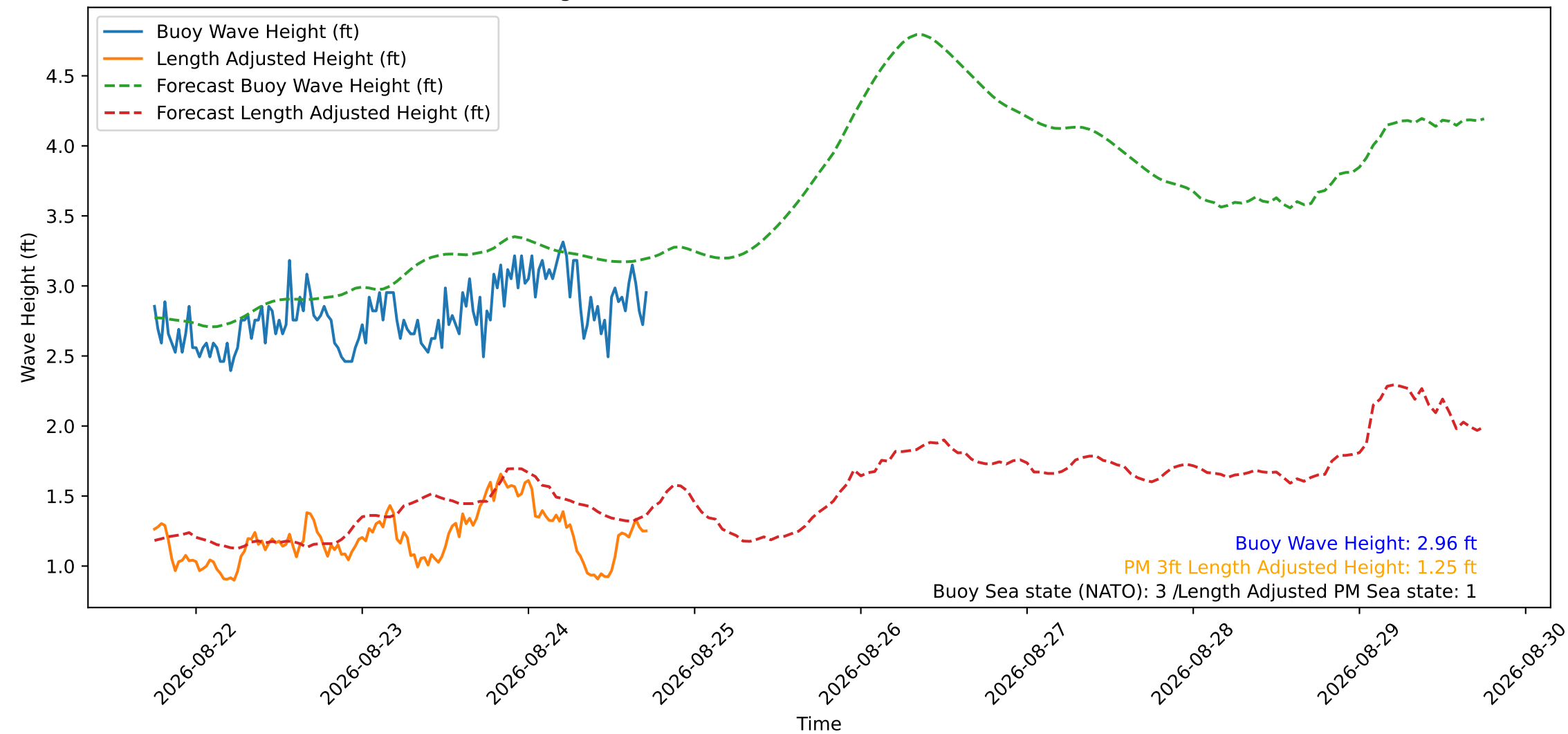
Wave Heights over Time for Green Beach at 2026-08-24 17:51:14
