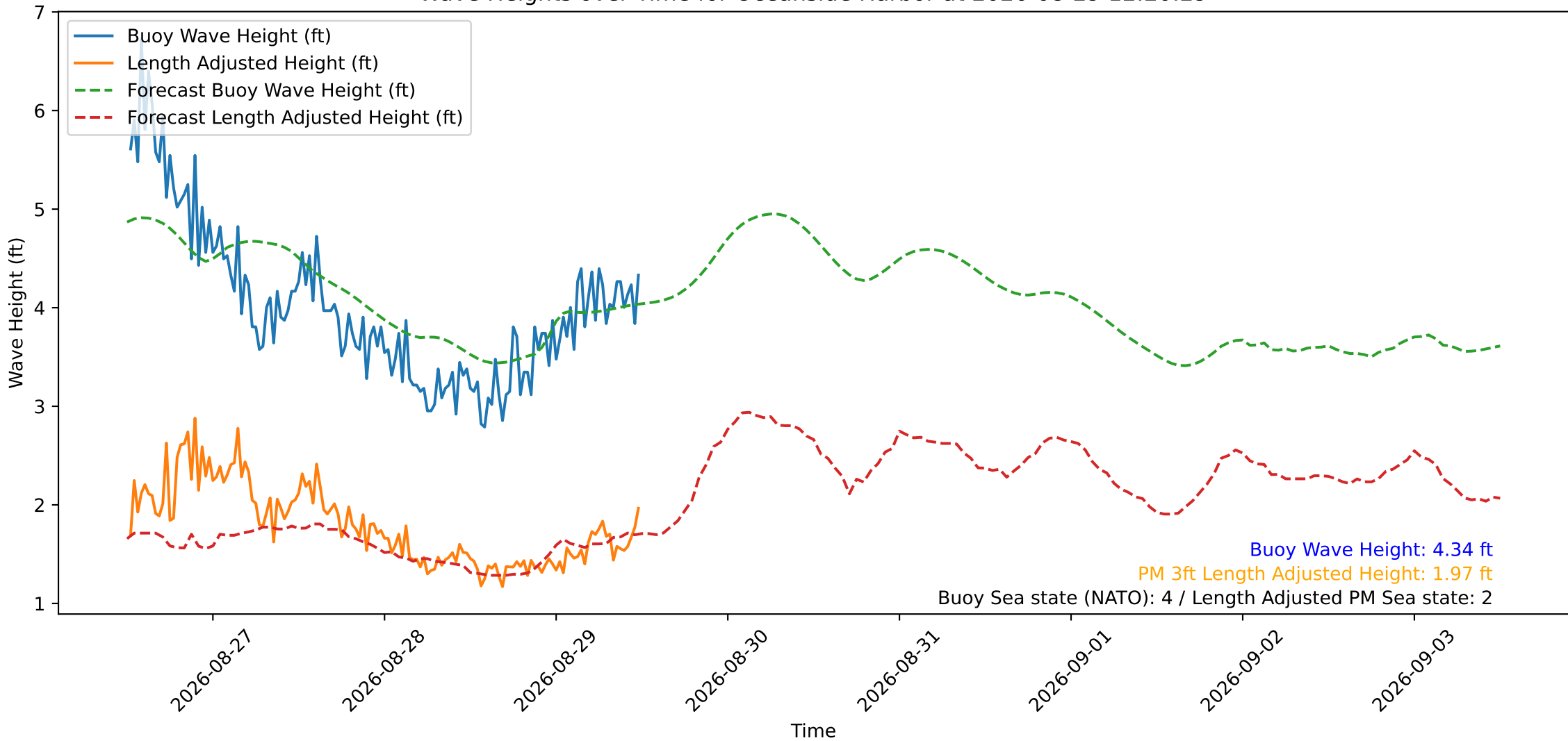
Wave Heights over Time for Oceanside Harbor at 2026-08-29 12:20:29
