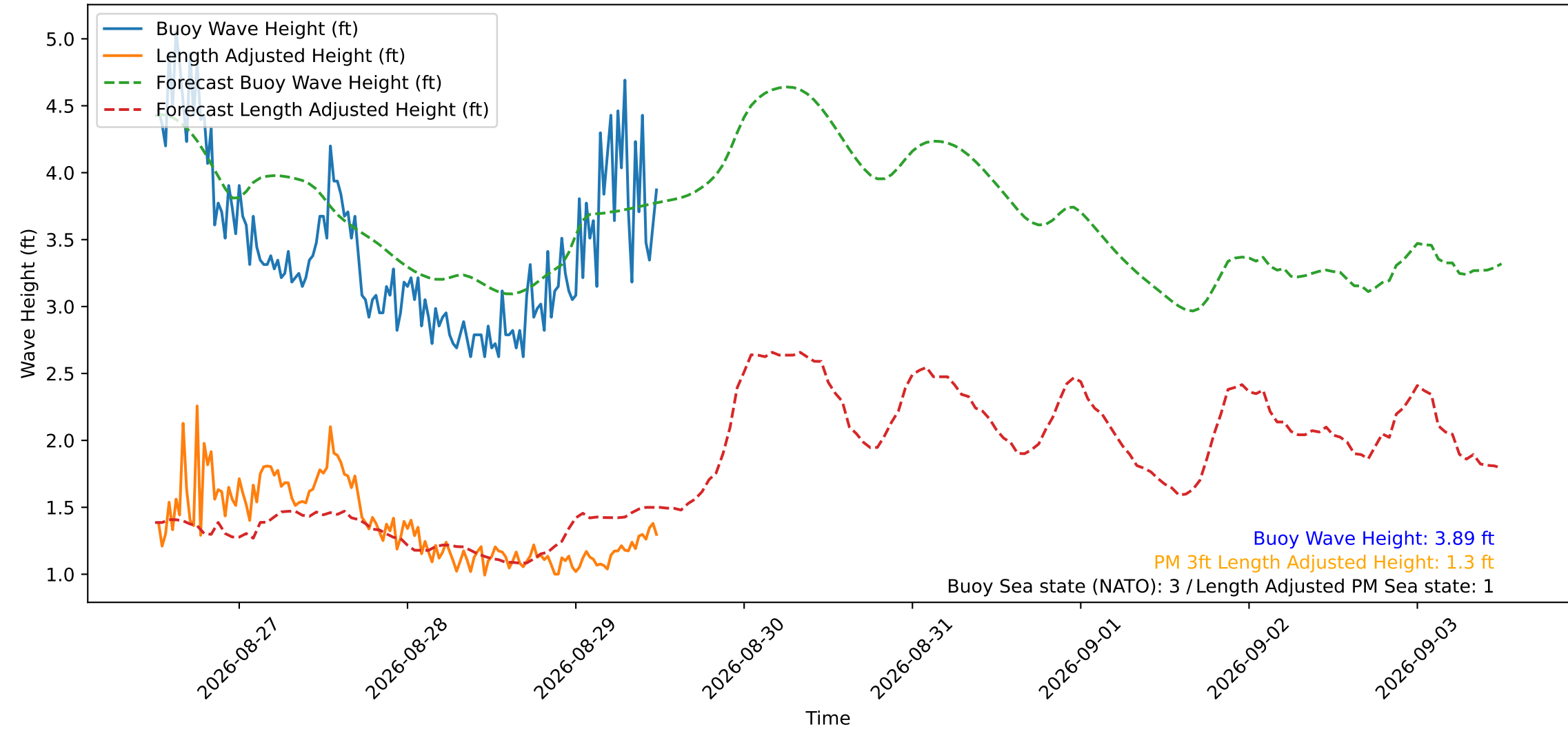
Wave Heights over Time for Red Beach at 2026-08-29 12:20:50
