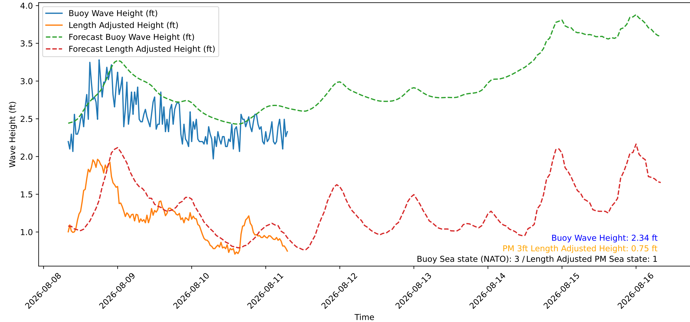
Wave Heights over Time for Oceanside Harbor at 2026-08-11 07:50:26
