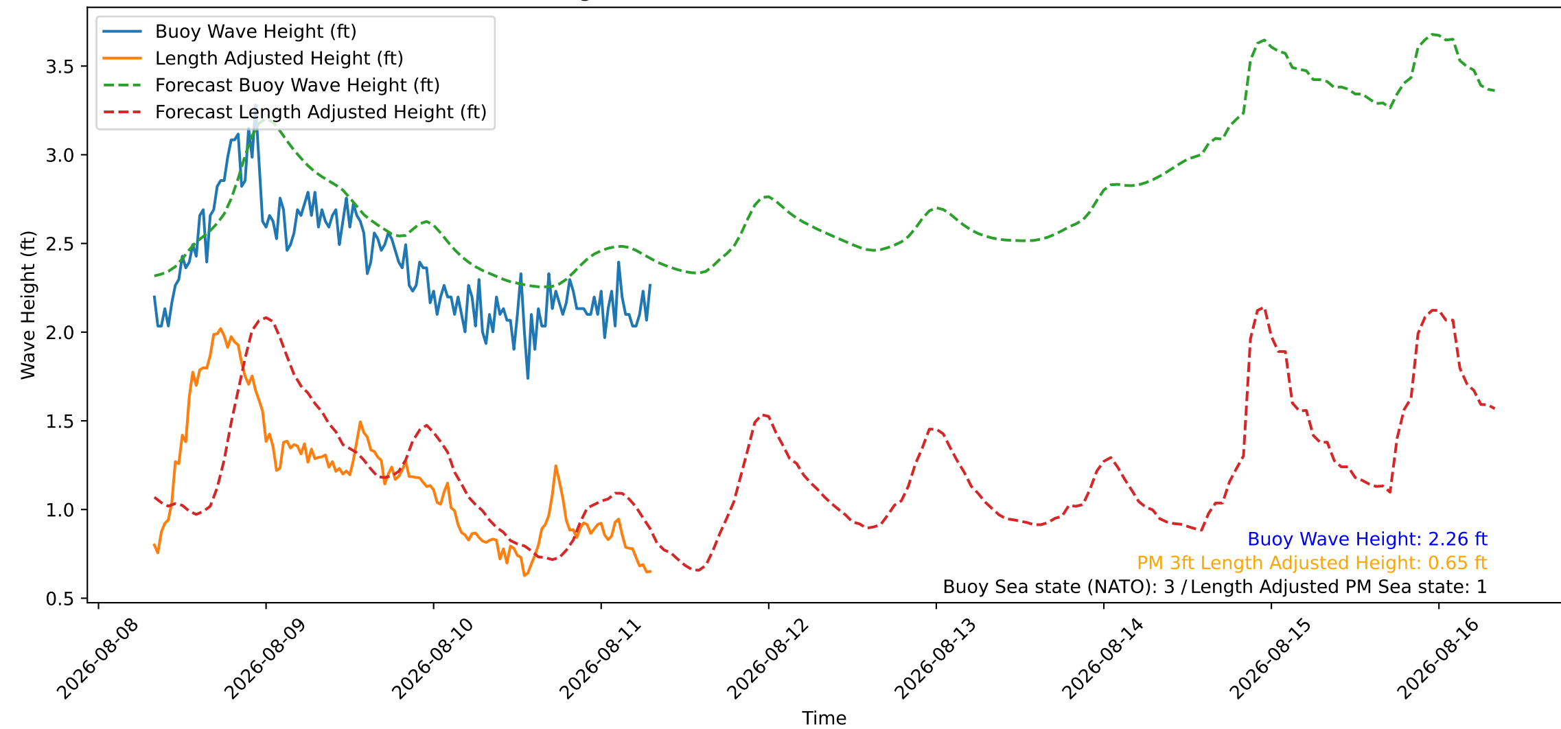
Wave Heights over Time for Red Beach at 2026-08-11 07:50:47
