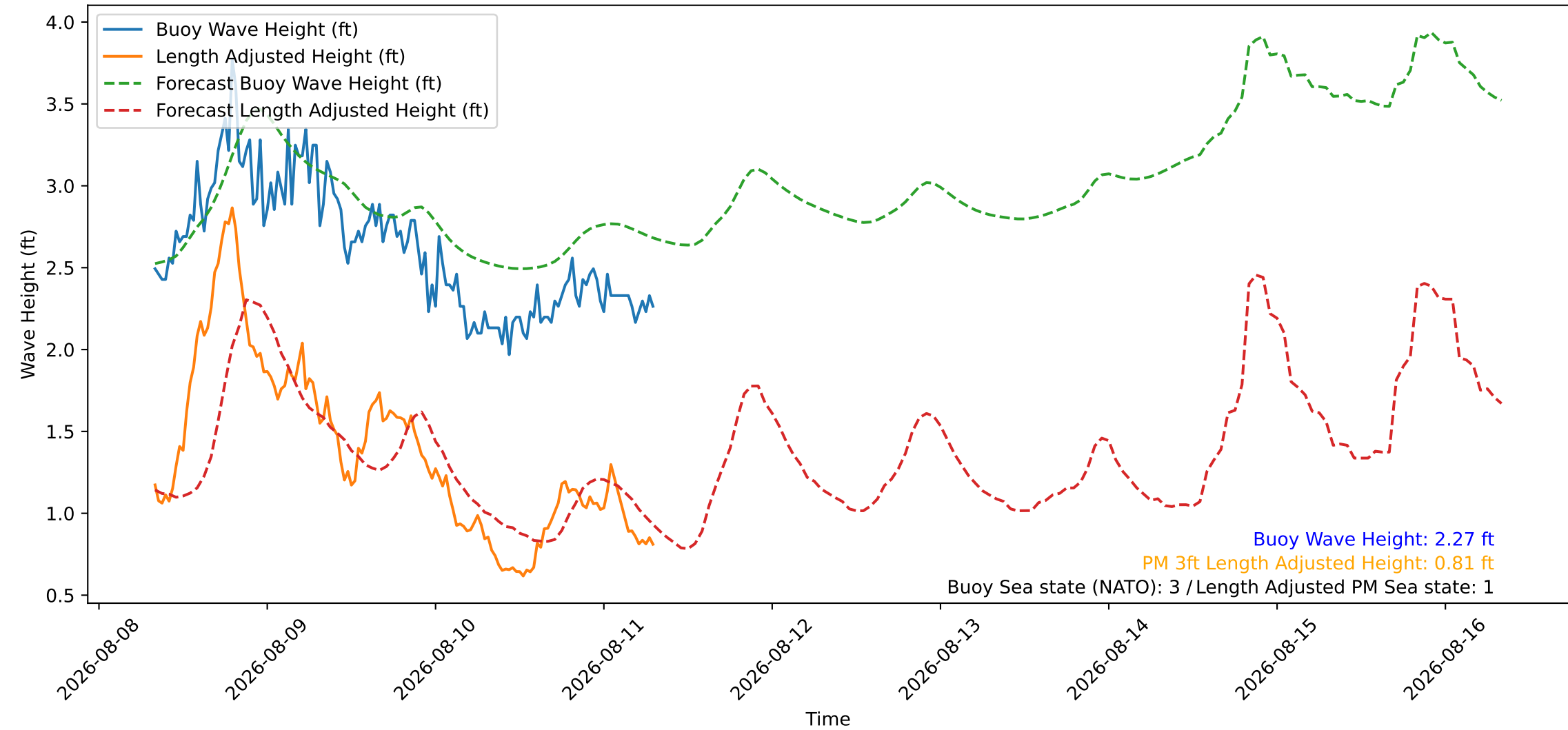
Wave Heights over Time for Green Beach at 2026-08-11 07:51:10
