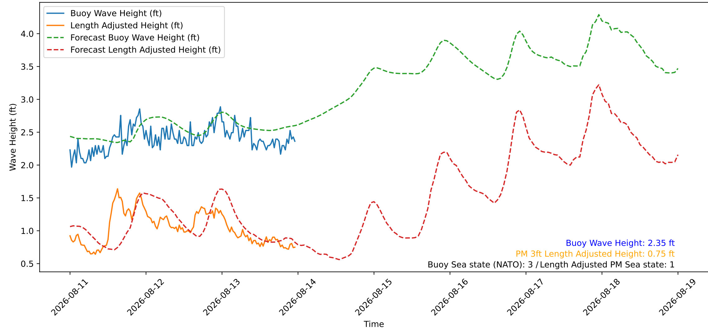
Wave Heights over Time for Red Beach at 2026-08-13 23:50:46
