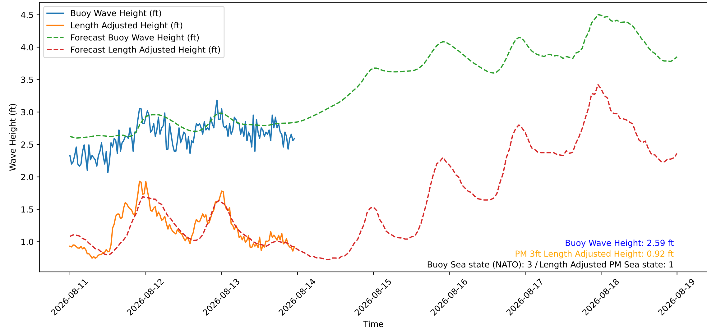
Wave Heights over Time for Oceanside Harbor at 2026-08-13 23:50:26
