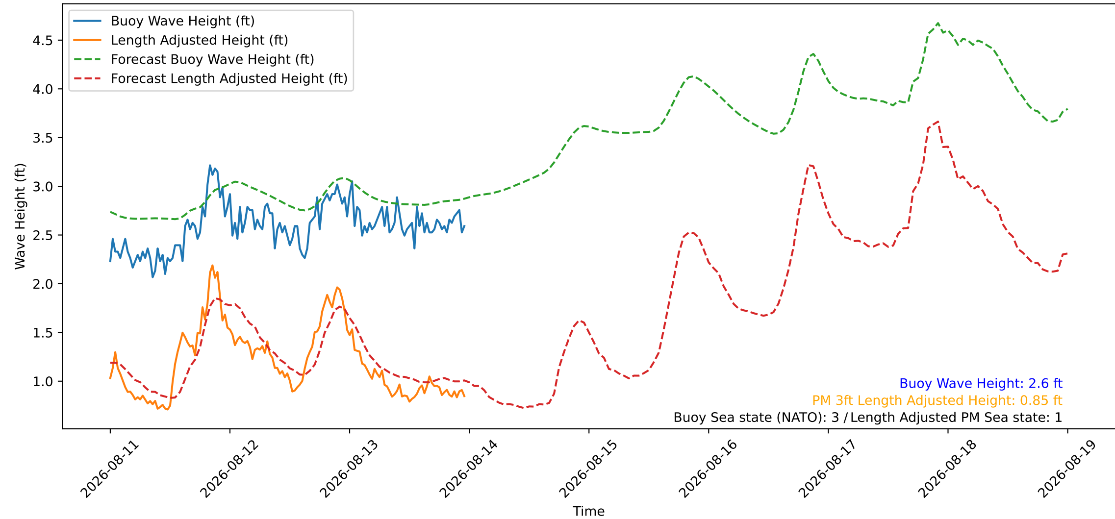
Wave Heights over Time for Green Beach at 2026-08-13 23:51:09
