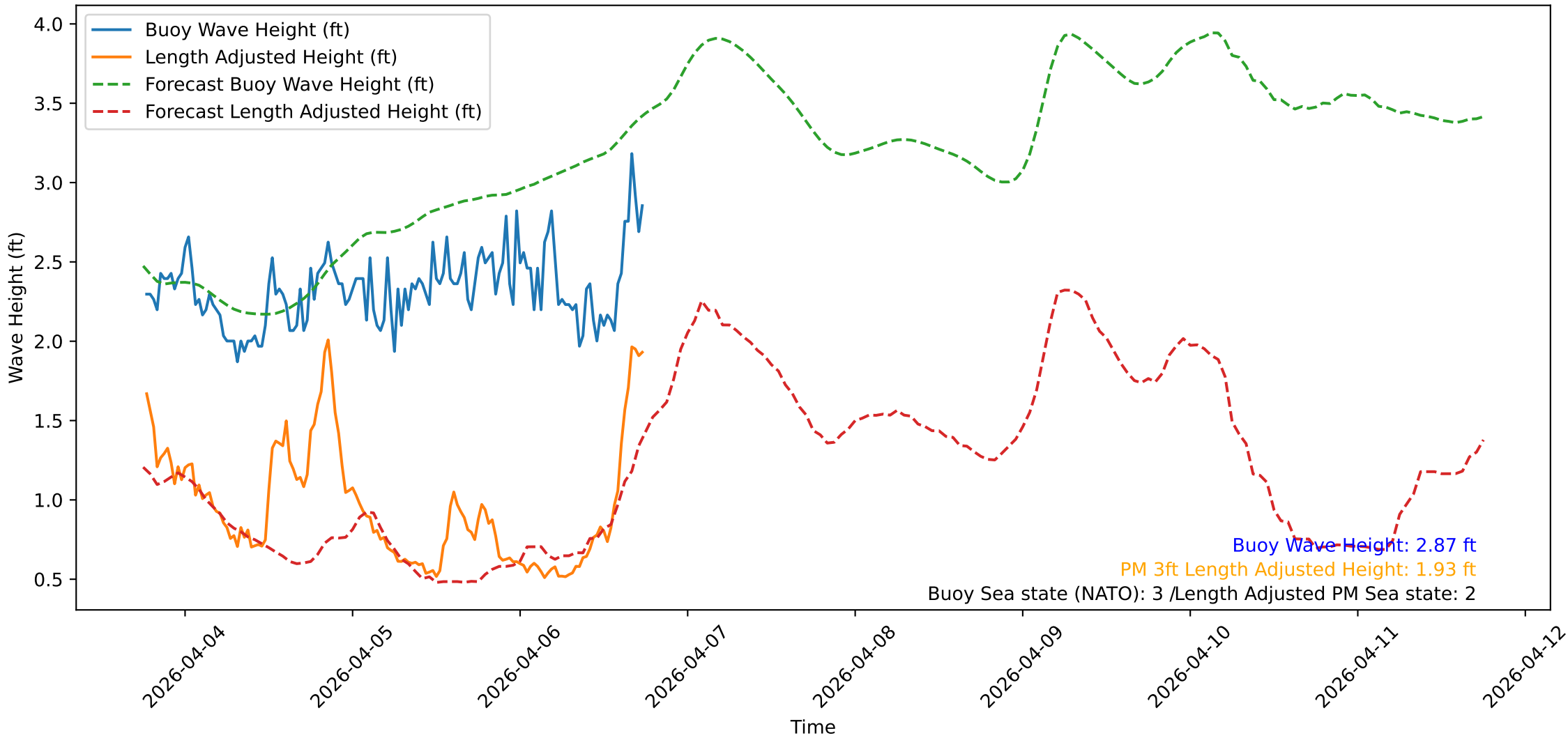
Wave Heights over Time for Red Beach at 2026-04-06 18:10:47
