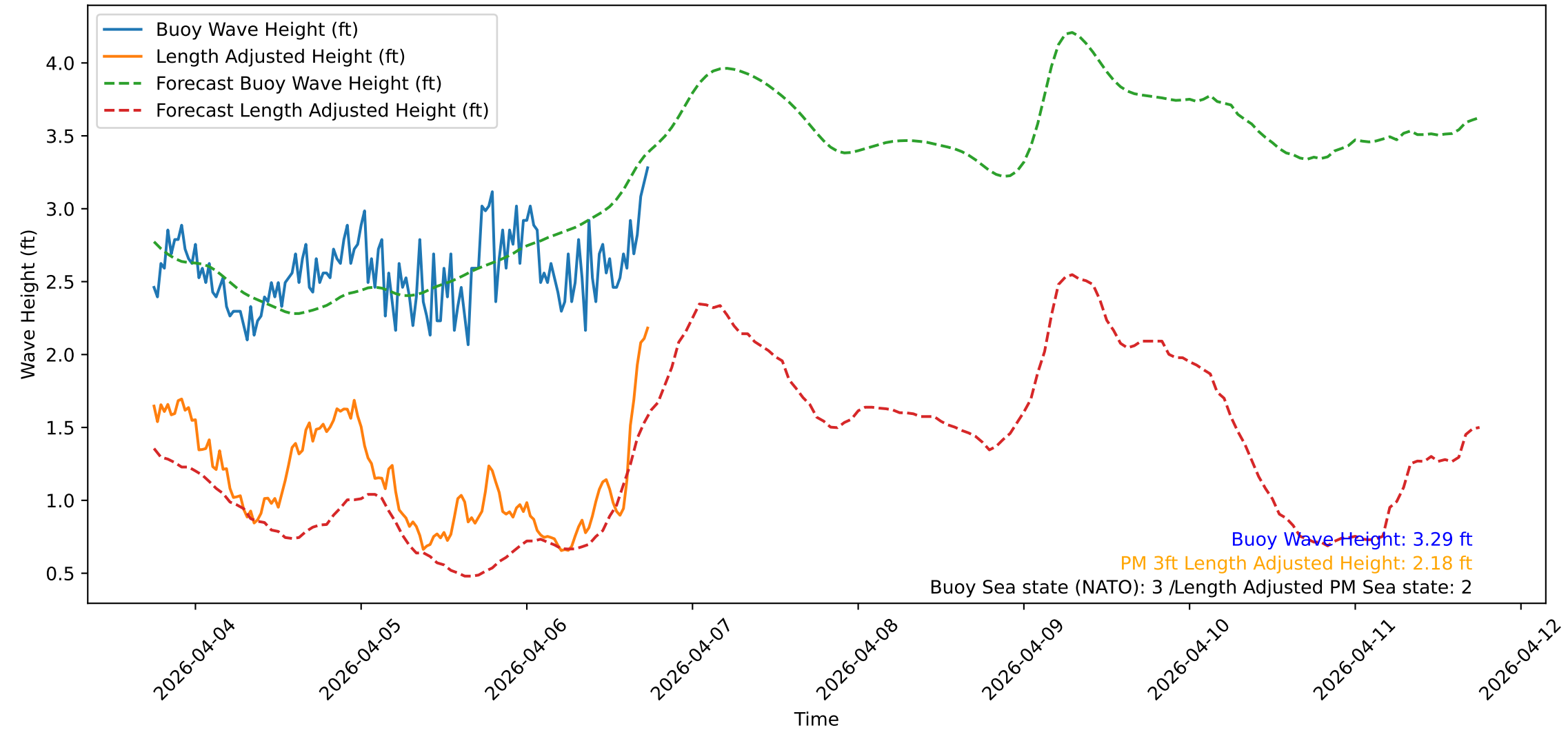
Wave Heights over Time for Oceanside Harbor at 2026-04-06 18:10:31
