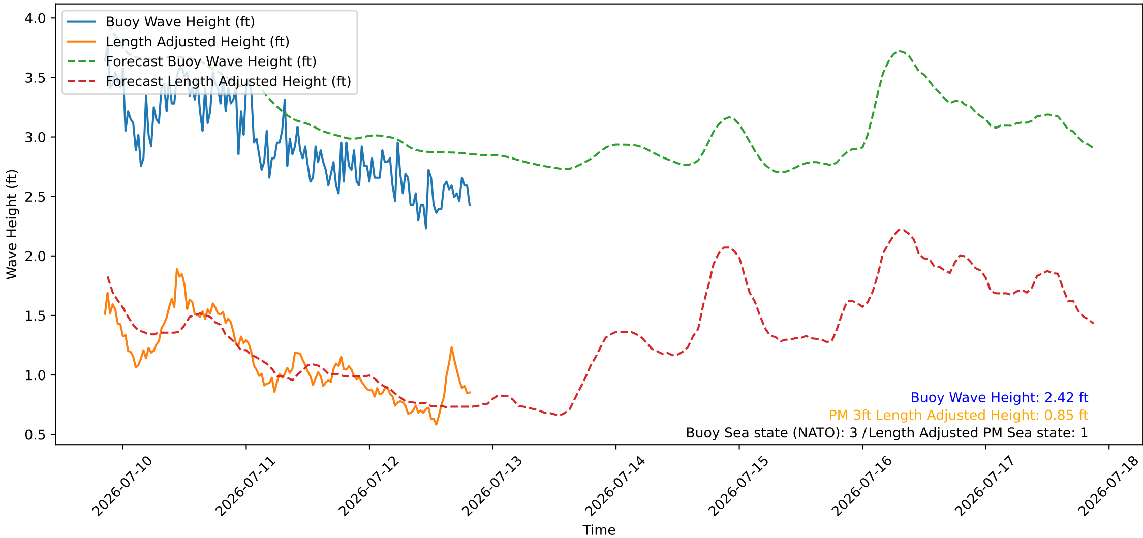
Wave Heights over Time for Green Beach at 2026-07-12 20:31:08
