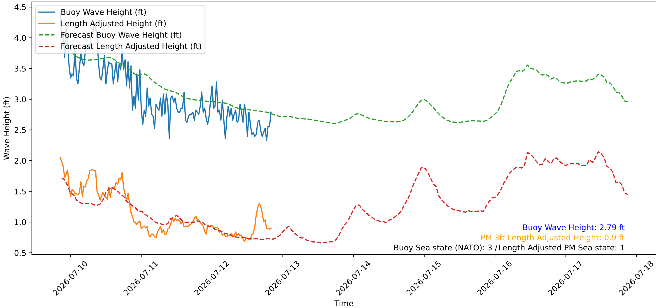
Wave Heights over Time for Oceanside Harbor at 2026-07-12 20:30:27
