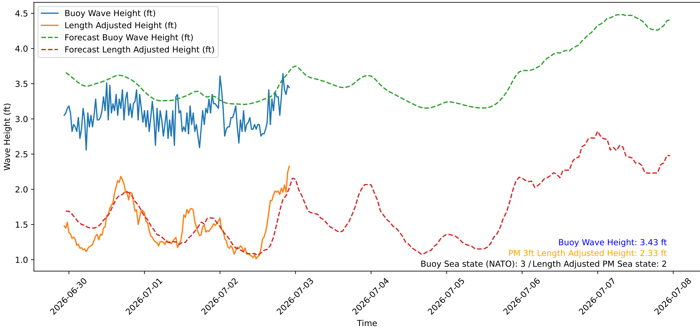
Wave Heights over Time for Oceanside Harbor at 2026-07-02 22:40:26
