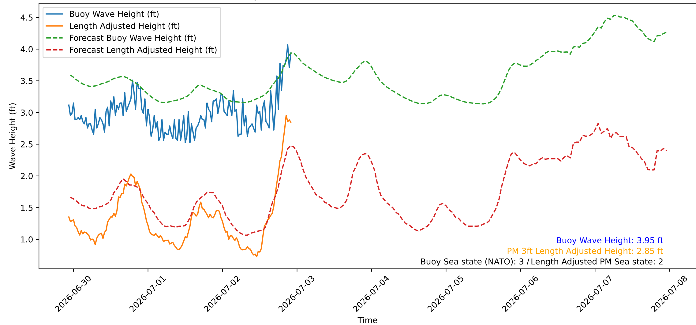
Wave Heights over Time for Green Beach at 2026-07-02 22:41:08
