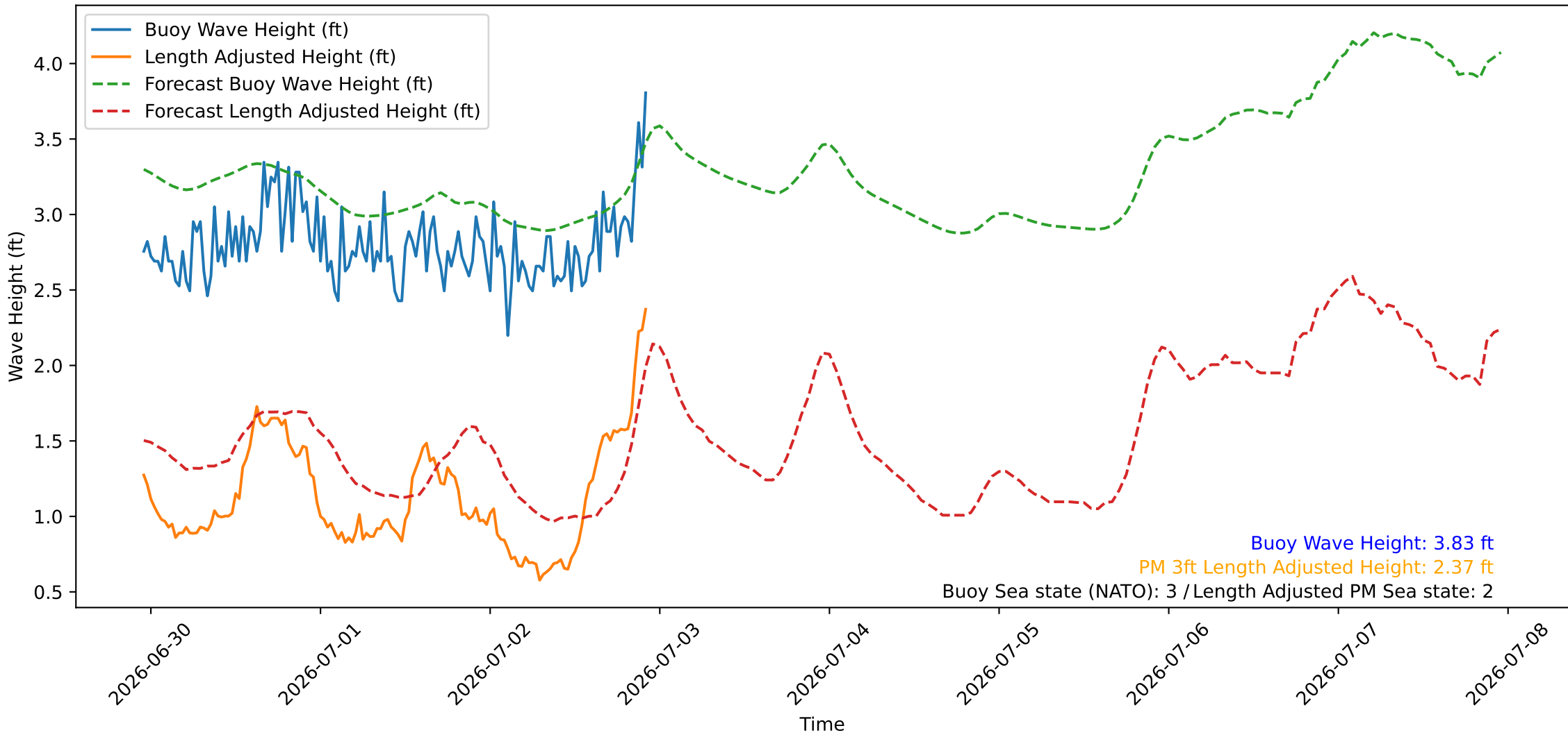
Wave Heights over Time for Red Beach at 2026-07-02 22:40:46
