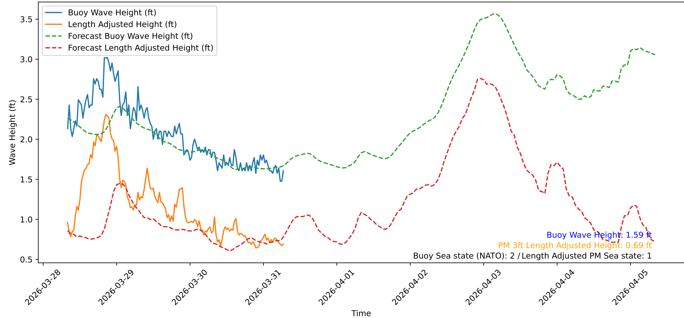
Wave Heights over Time for Red Beach at 2026-03-31 07:30:46
