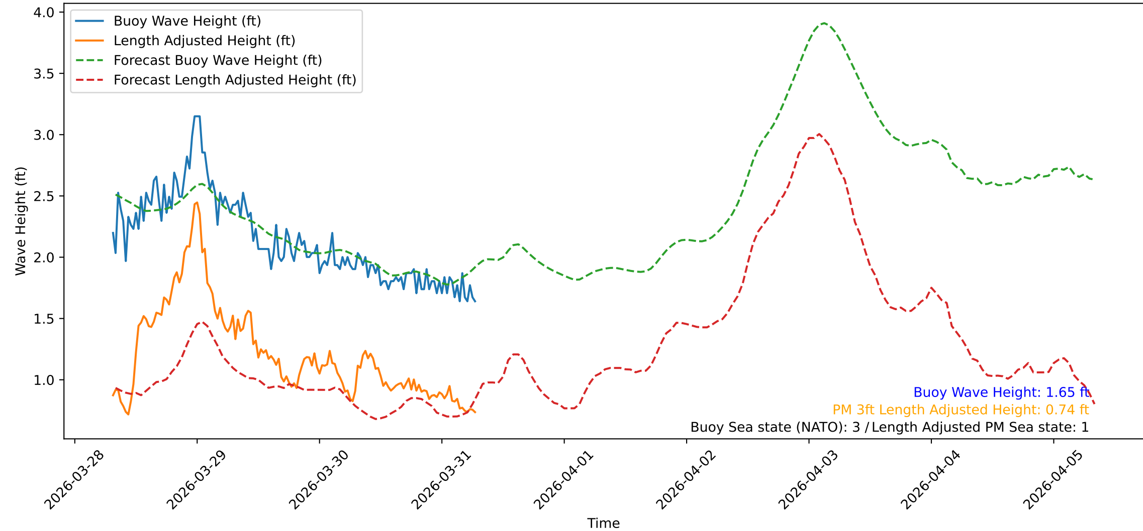
Wave Heights over Time for Oceanside Harbor at 2026-03-31 07:30:30
