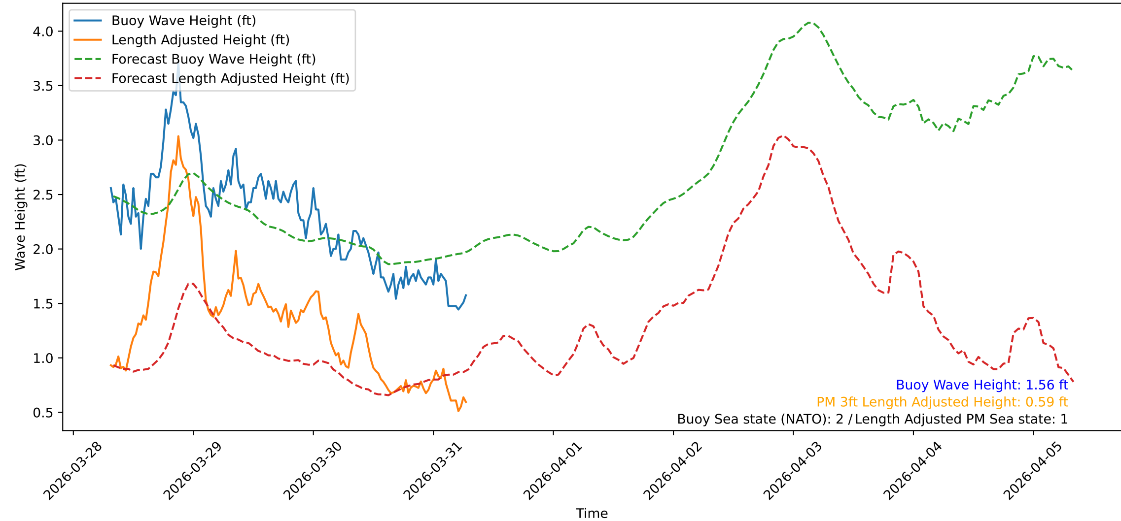
Wave Heights over Time for Green Beach at 2026-03-31 07:31:09
