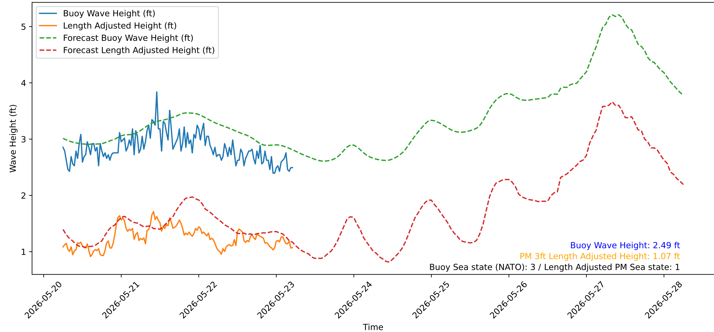
Wave Heights over Time for Oceanside Harbor at 2026-05-23 06:00:31
