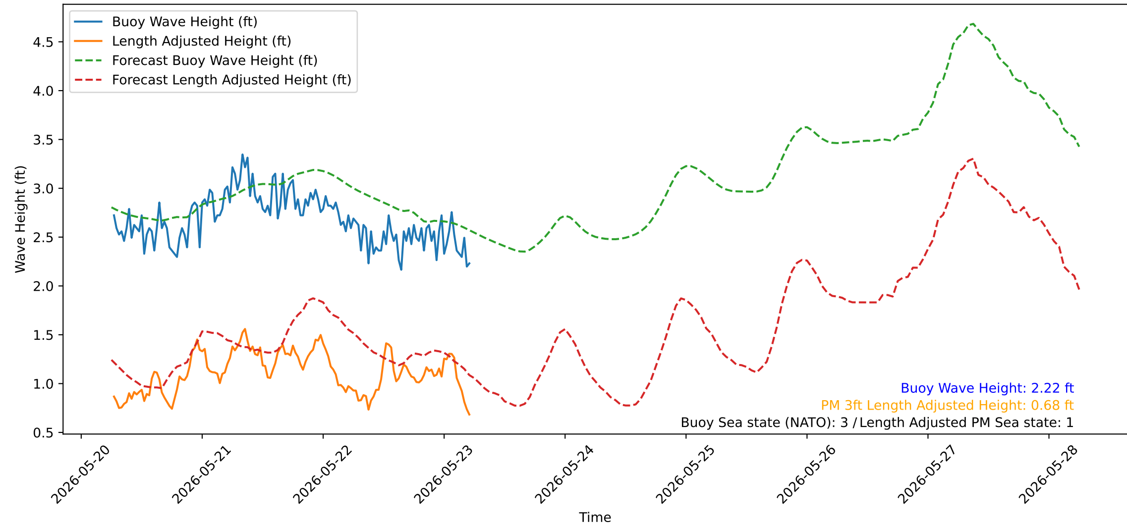
Wave Heights over Time for Red Beach at 2026-05-23 06:00:51
