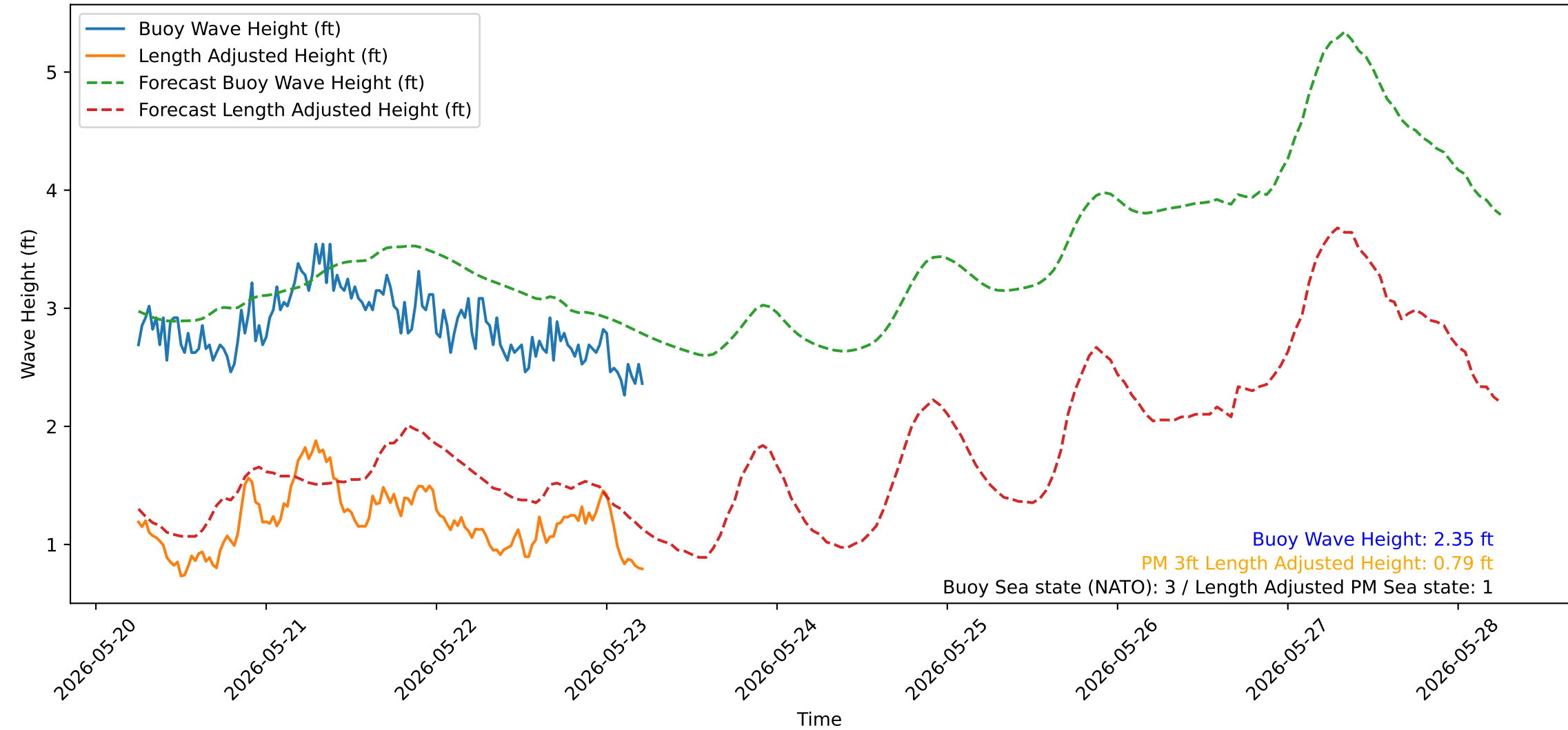
Wave Heights over Time for Green Beach at 2026-05-23 06:01:14
