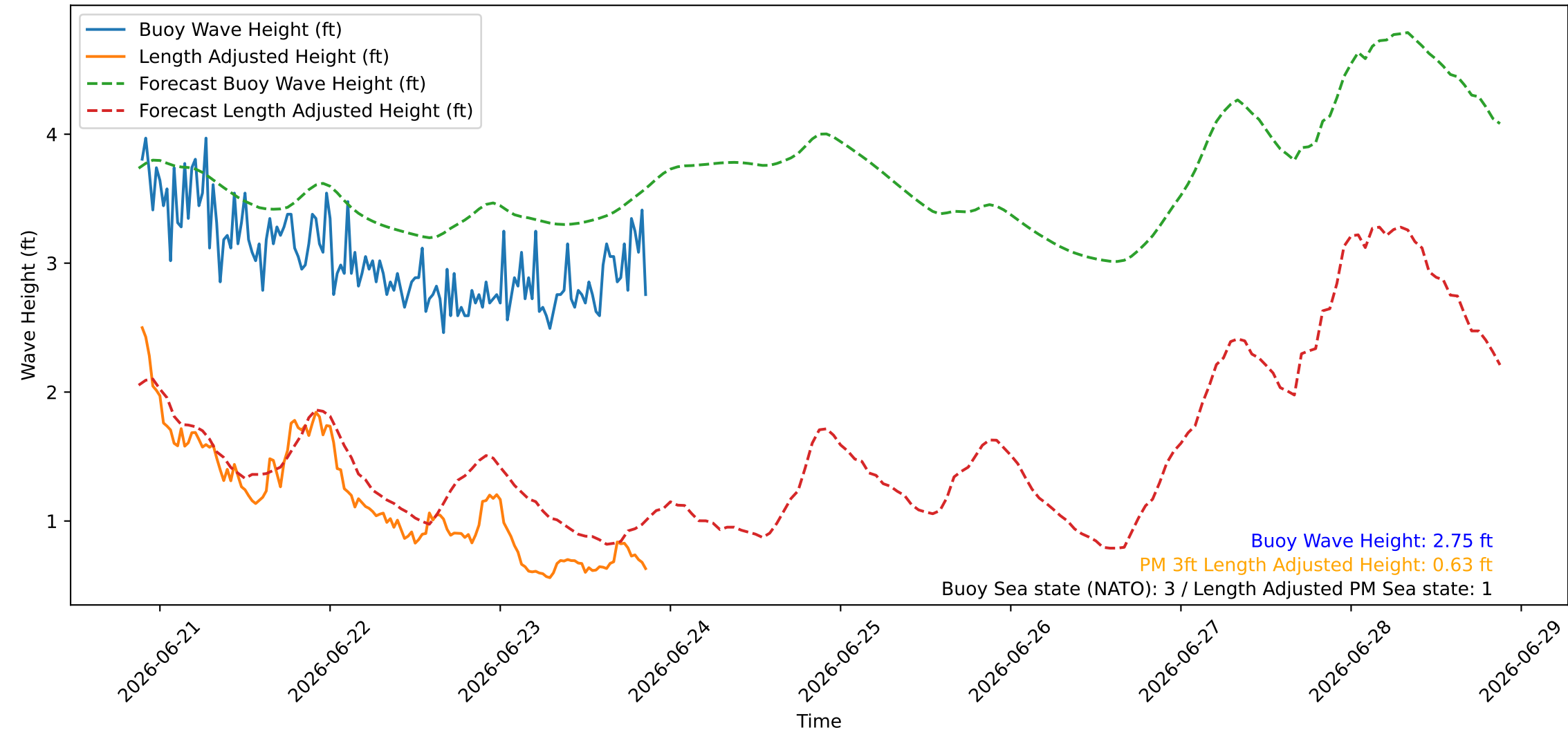
Wave Heights over Time for Green Beach at 2026-06-23 21:21:09
