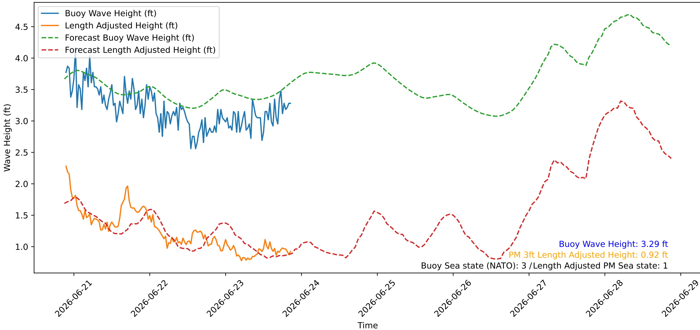
Wave Heights over Time for Oceanside Harbor at 2026-06-23 21:20:26
