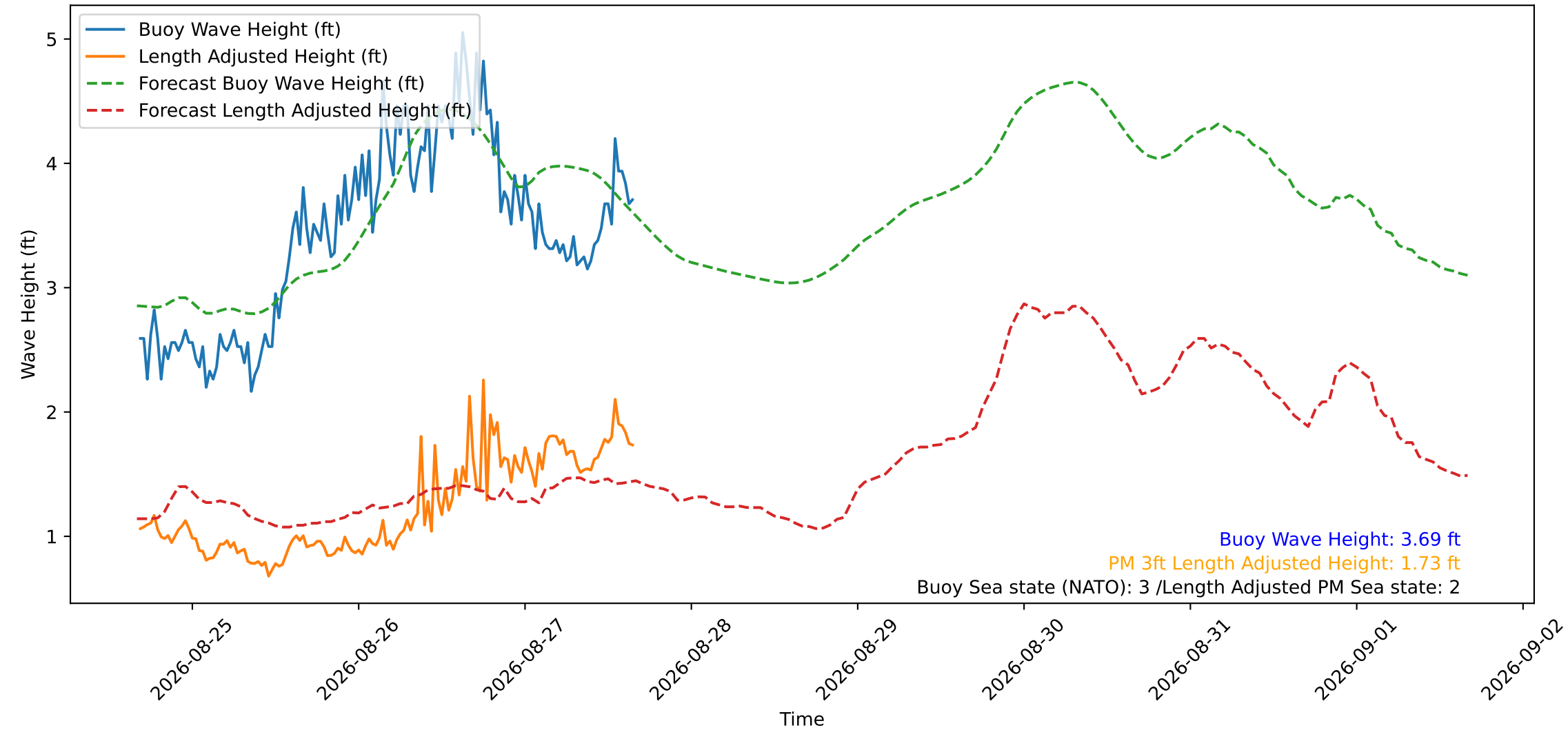
Wave Heights over Time for Red Beach at 2026-08-27 16:20:51
