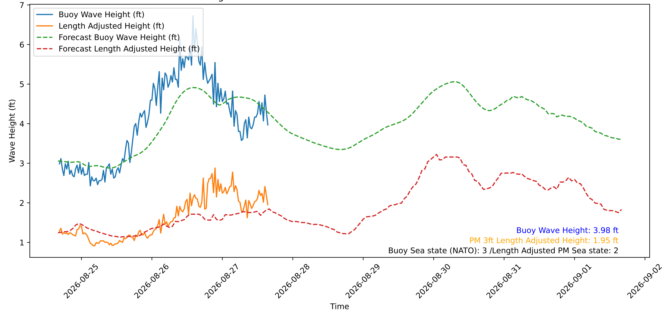
Wave Heights over Time for Oceanside Harbor at 2026-08-27 16:20:30
