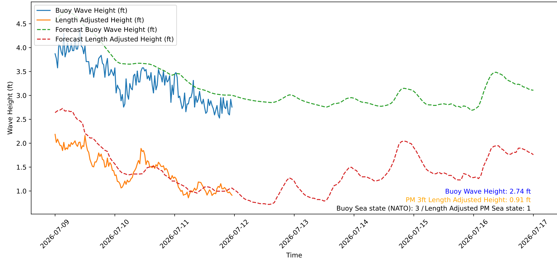
Wave Heights over Time for Green Beach at 2026-07-12 00:01:07
