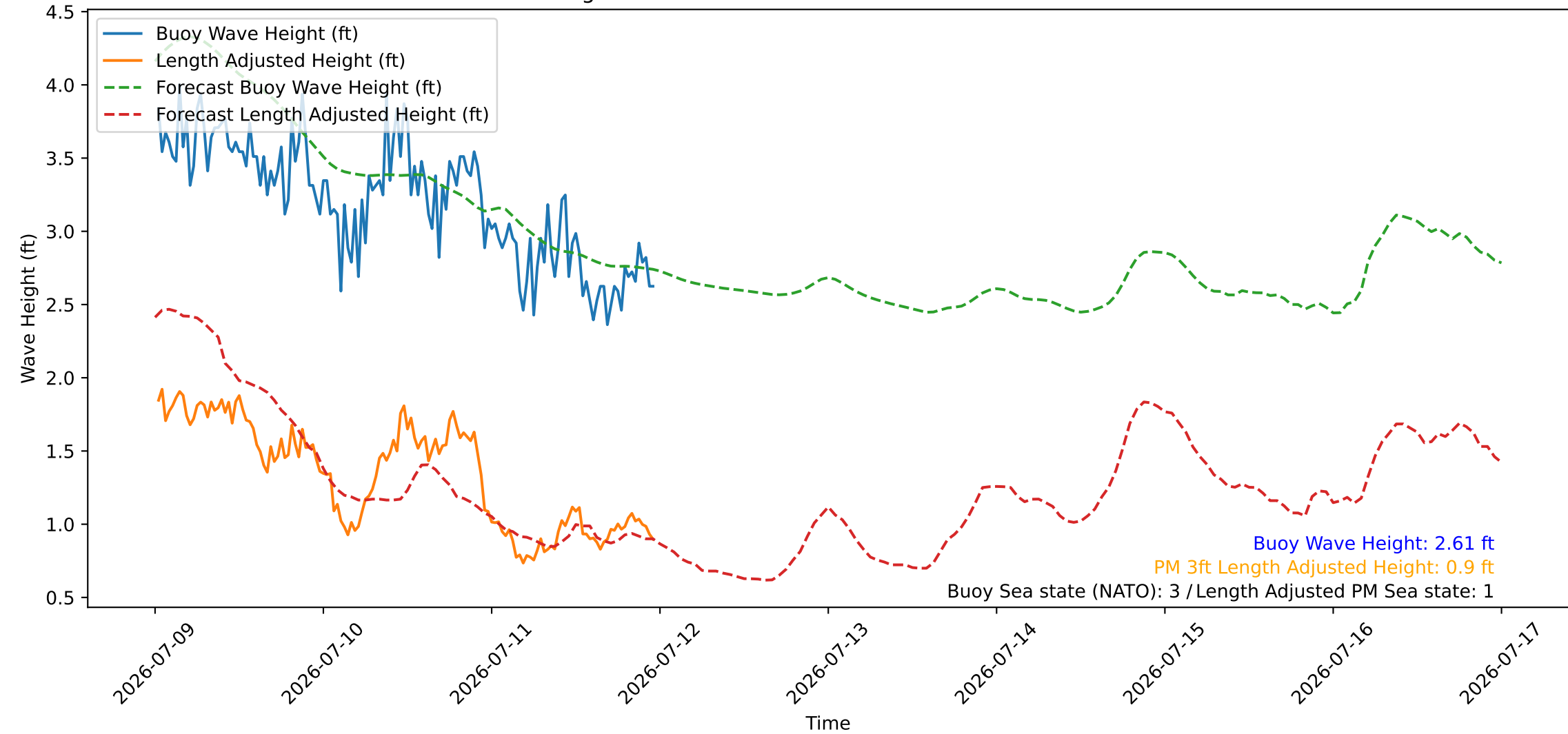
Wave Heights over Time for Red Beach at 2026-07-12 00:00:45
