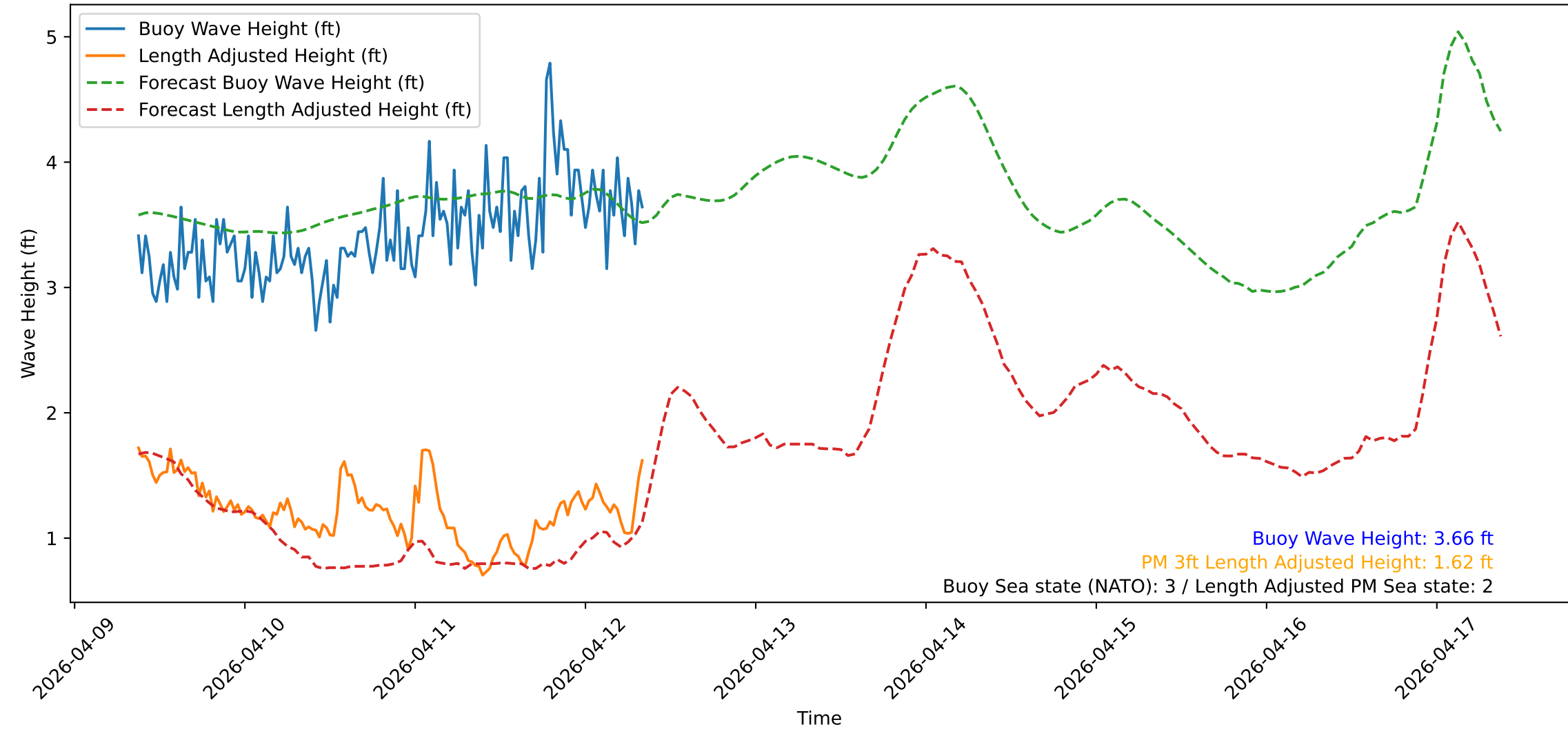
Wave Heights over Time for Oceanside Harbor at 2026-04-12 09:00:32
