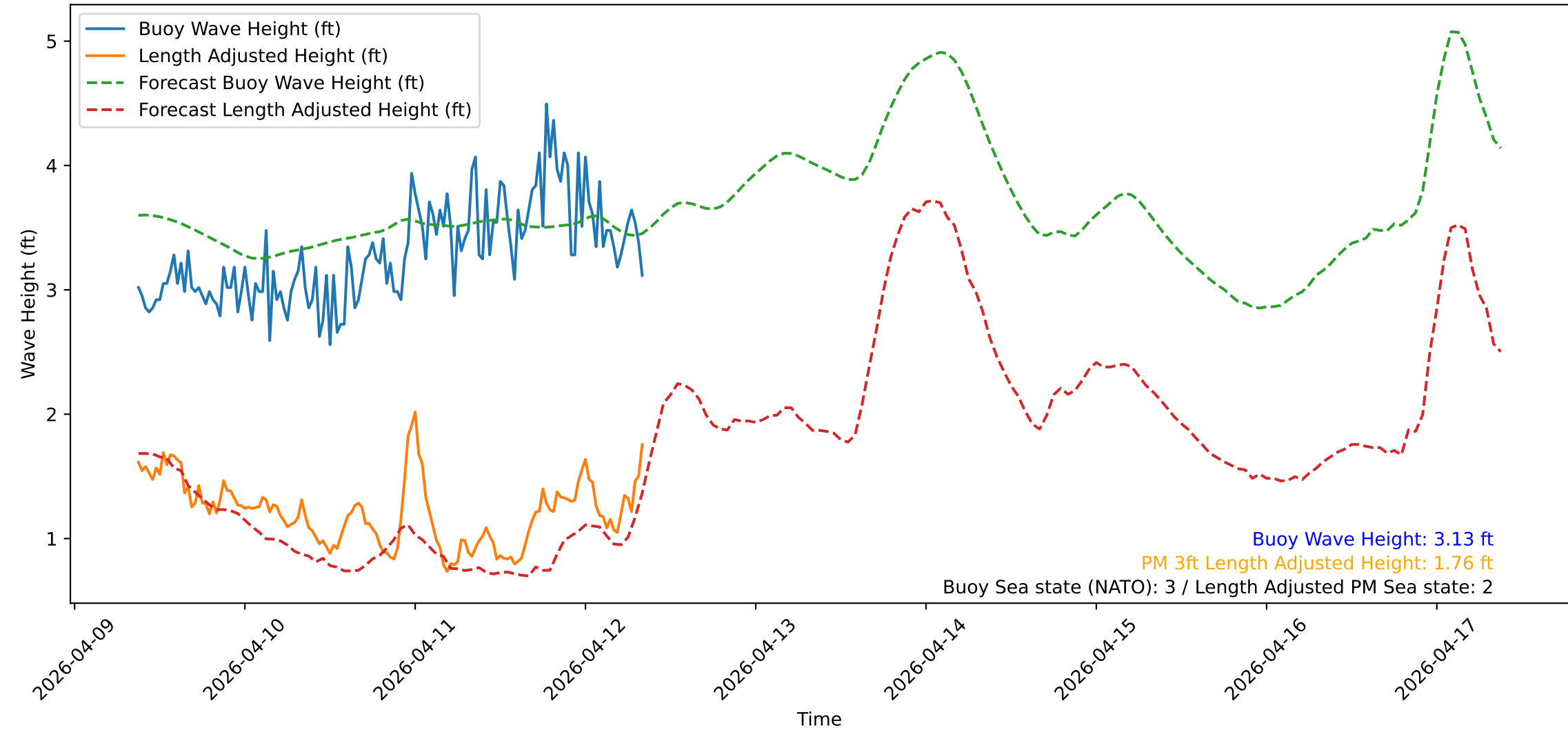
Wave Heights over Time for Green Beach at 2026-04-12 09:01:13
