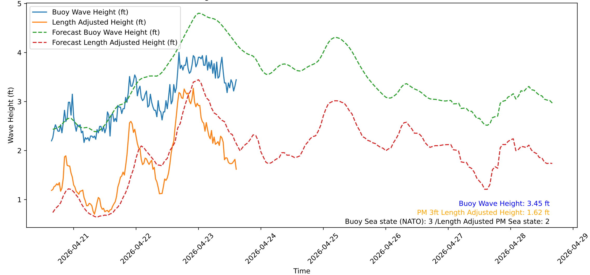
Wave Heights over Time for Green Beach at 2026-04-23 15:31:14
