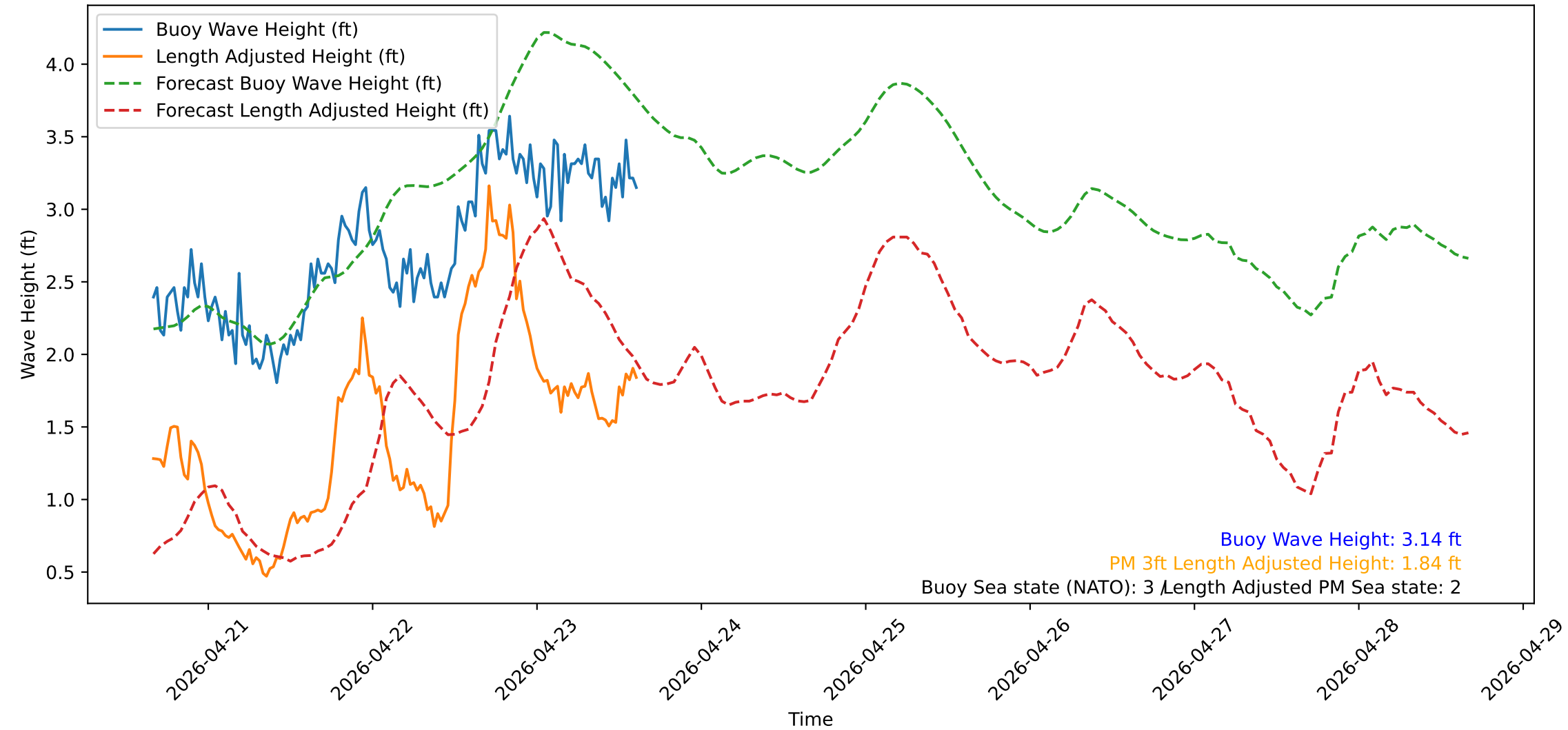
Wave Heights over Time for Red Beach at 2026-04-23 15:30:51
