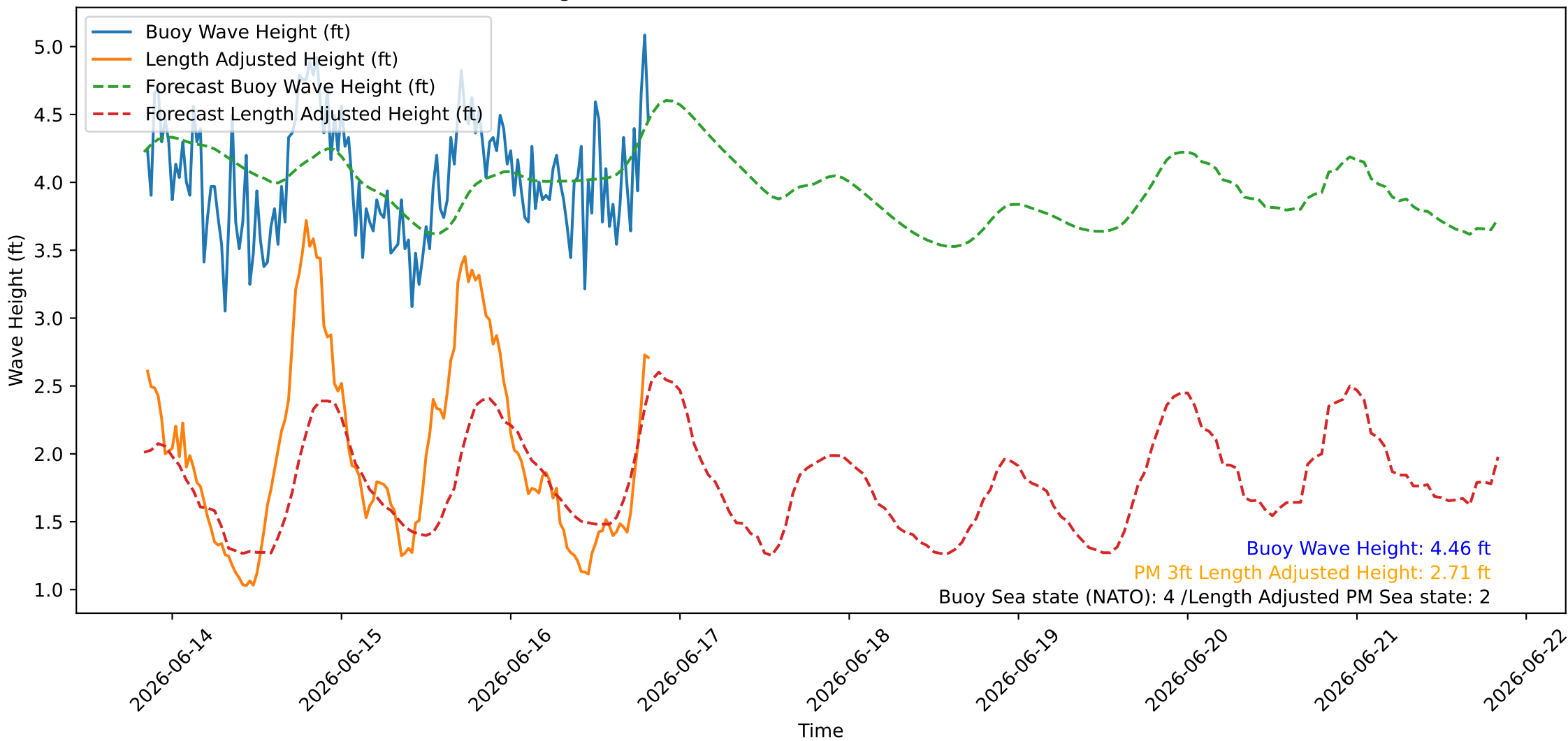
Wave Heights over Time for Green Beach at 2026-06-16 20:21:14
