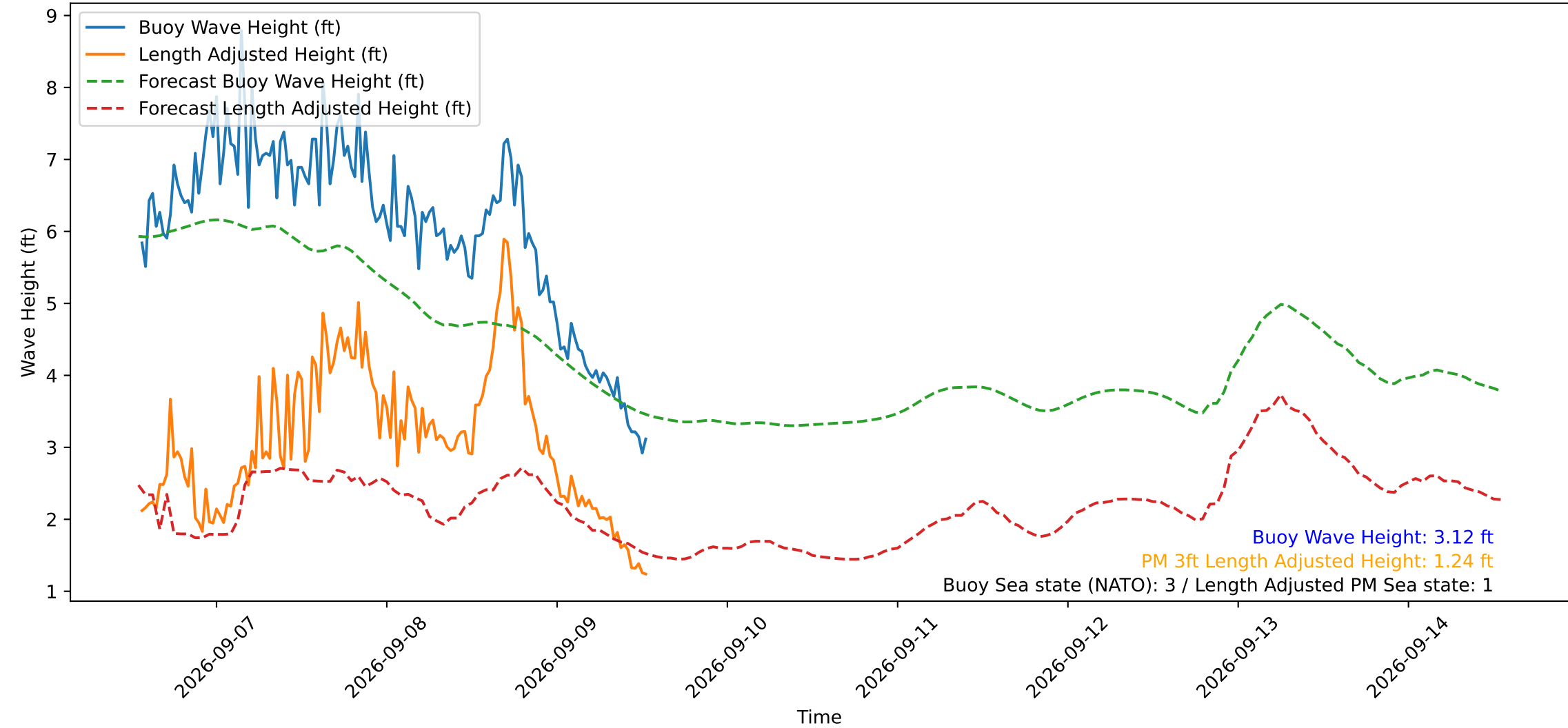
Wave Heights over Time for Green Beach at 2026-09-09 13:11:11
