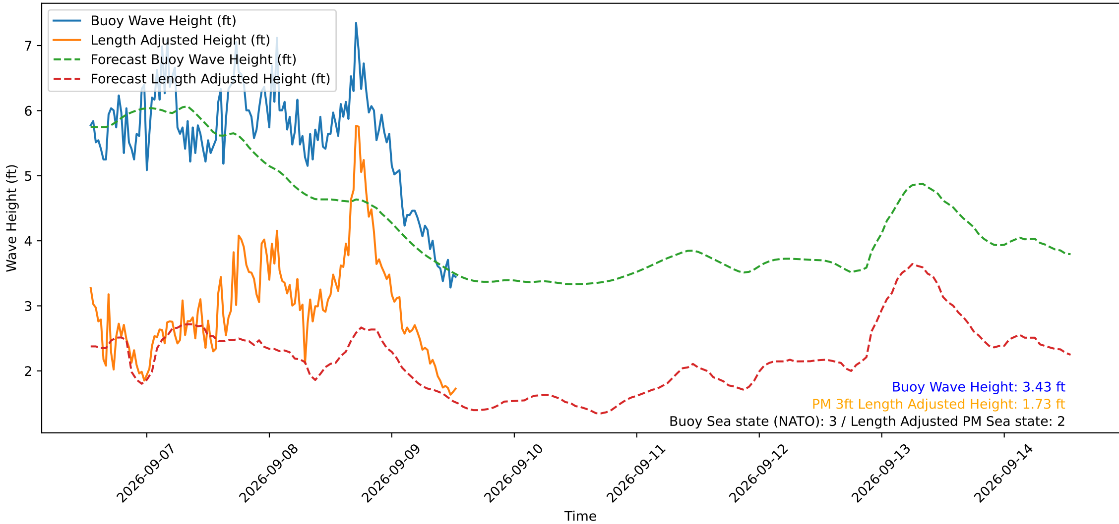
Wave Heights over Time for Oceanside Harbor at 2026-09-09 13:10:29
