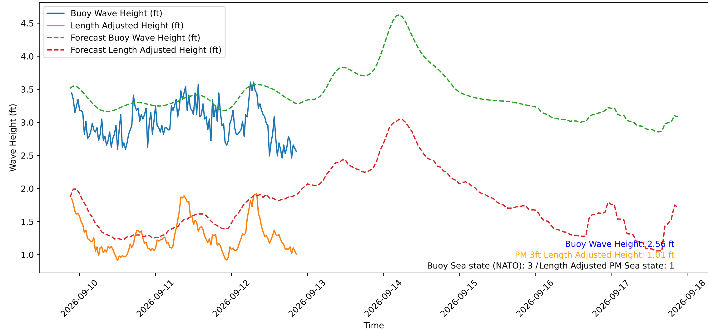
Wave Heights over Time for Green Beach at 2026-09-12 21:11:11
