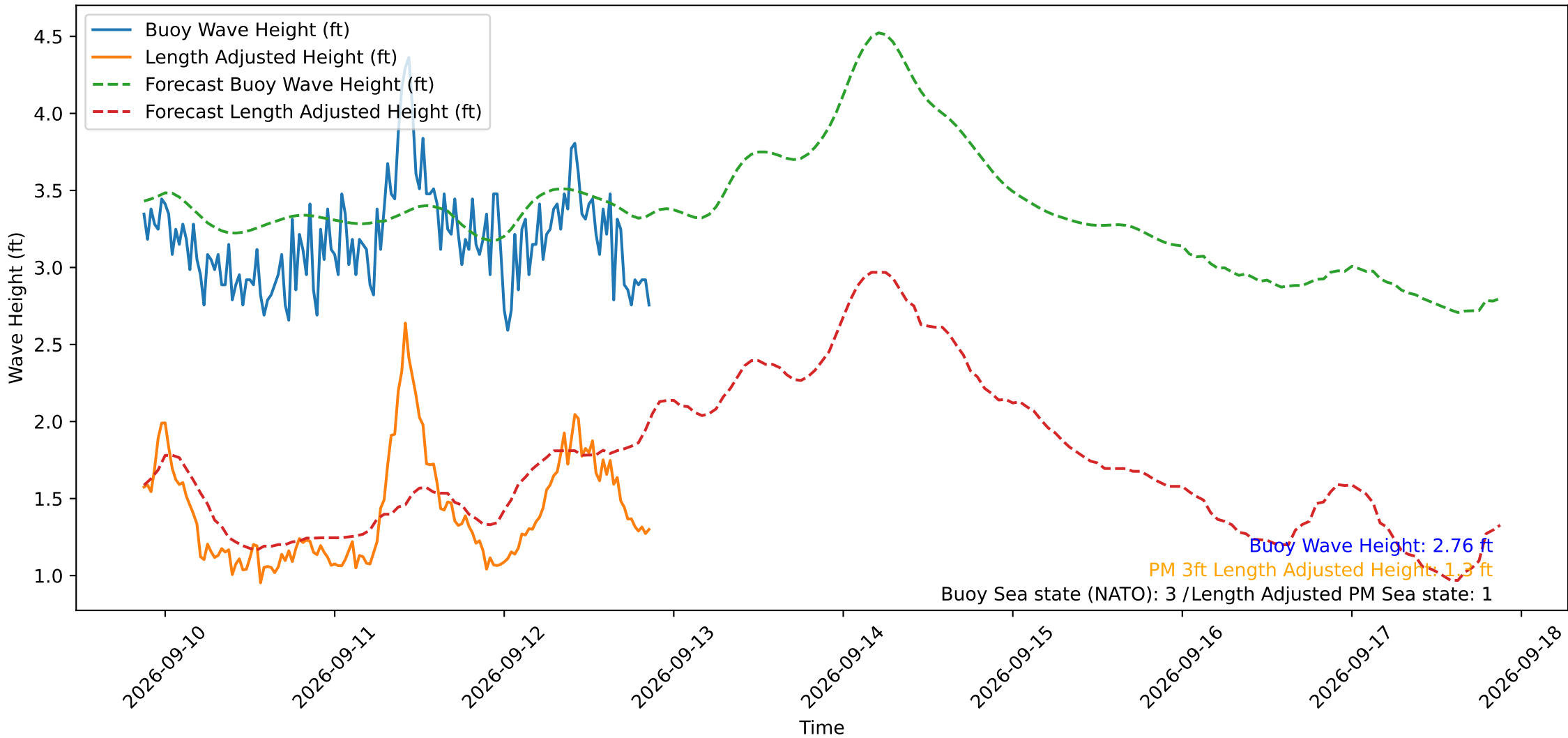
Wave Heights over Time for Oceanside Harbor at 2026-09-12 21:10:30
