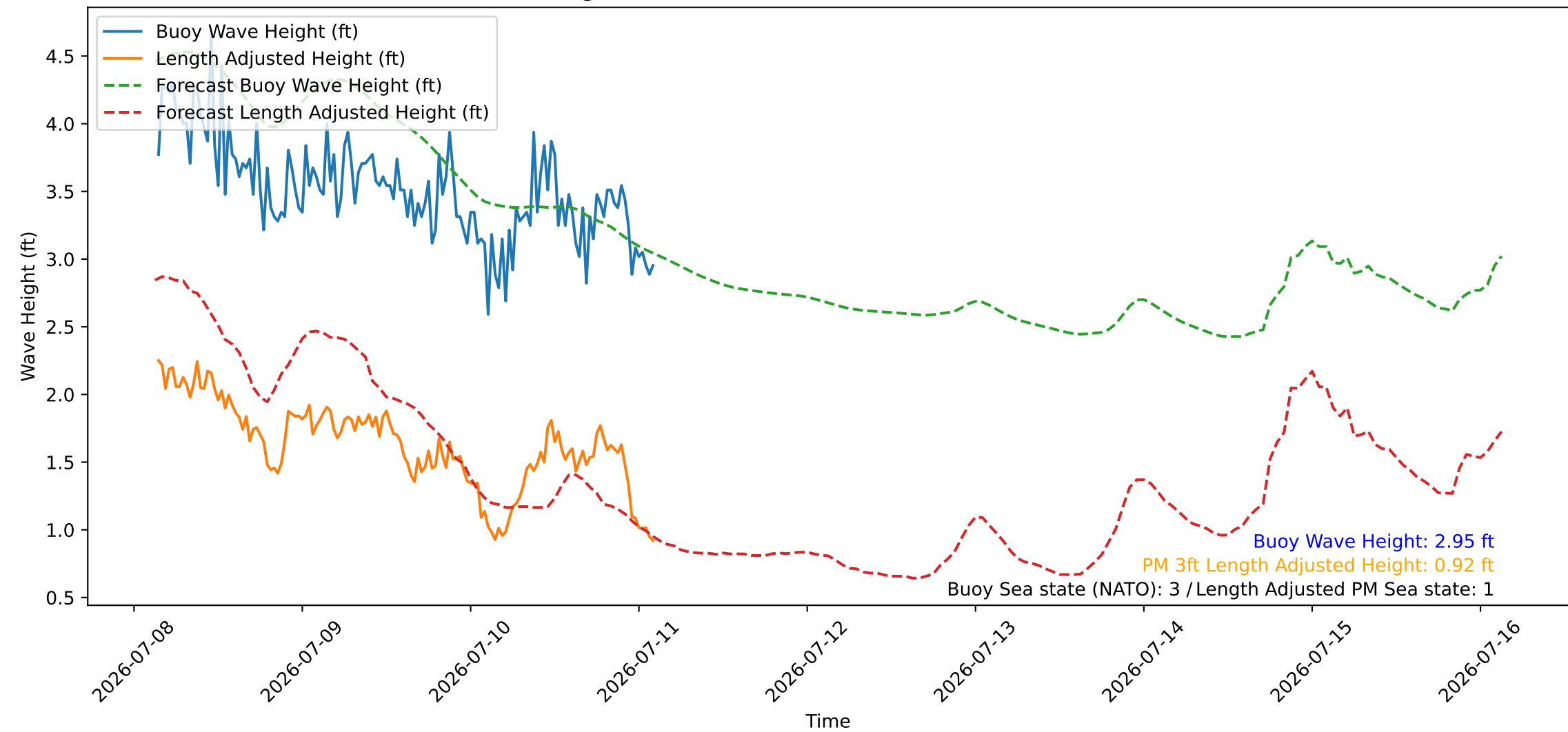
Wave Heights over Time for Red Beach at 2026-07-11 03:00:45
