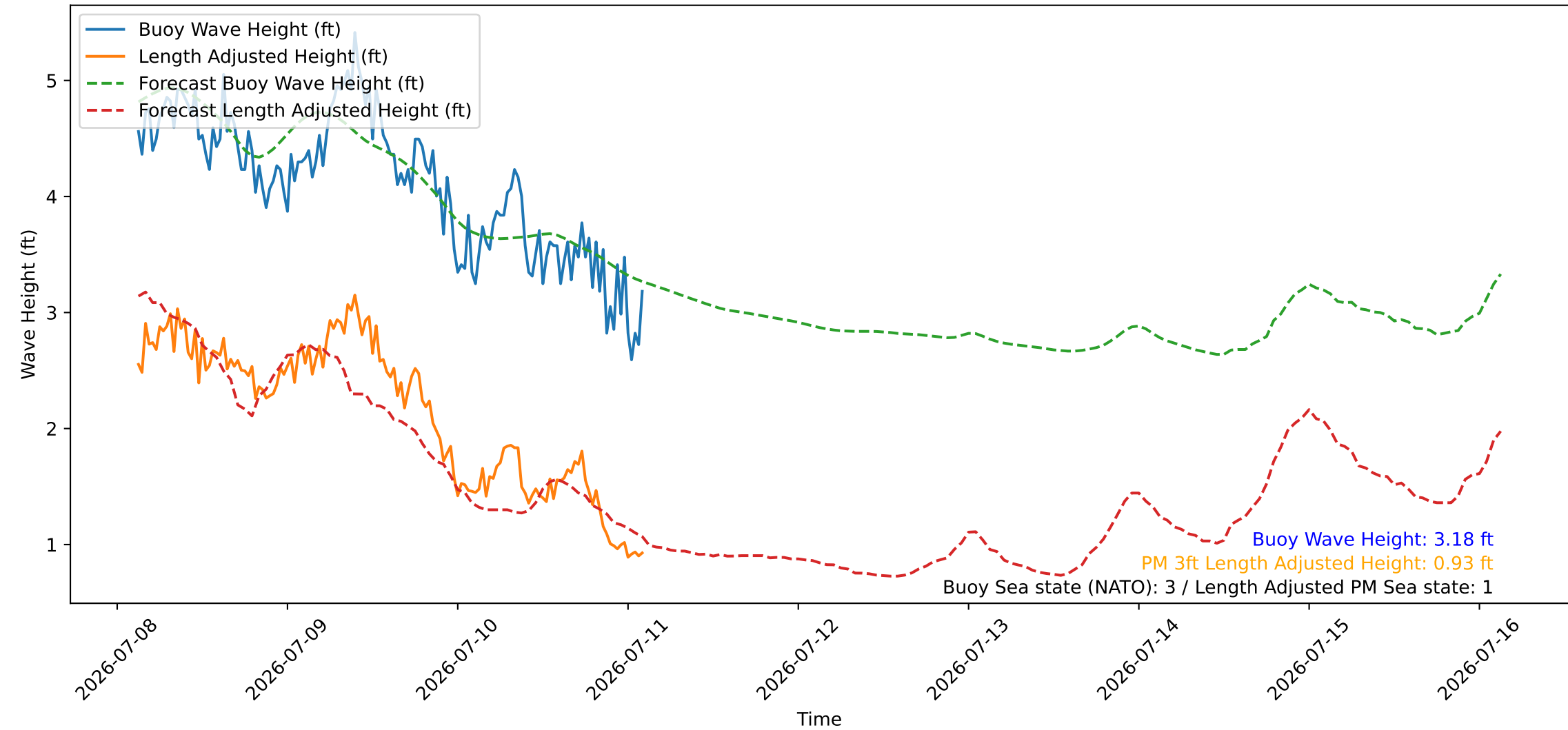
Wave Heights over Time for Oceanside Harbor at 2026-07-11 03:00:26
