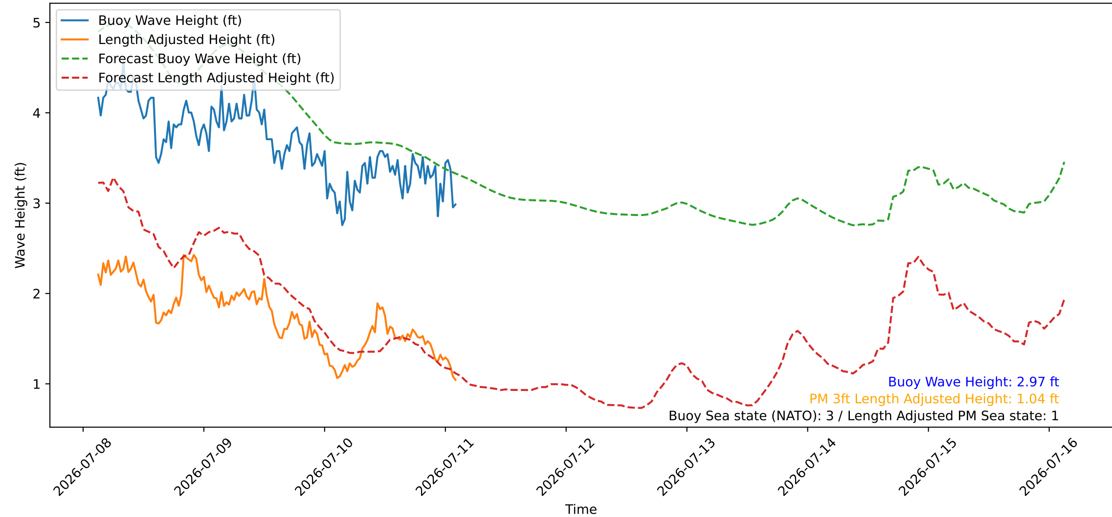
Wave Heights over Time for Green Beach at 2026-07-11 03:01:07
