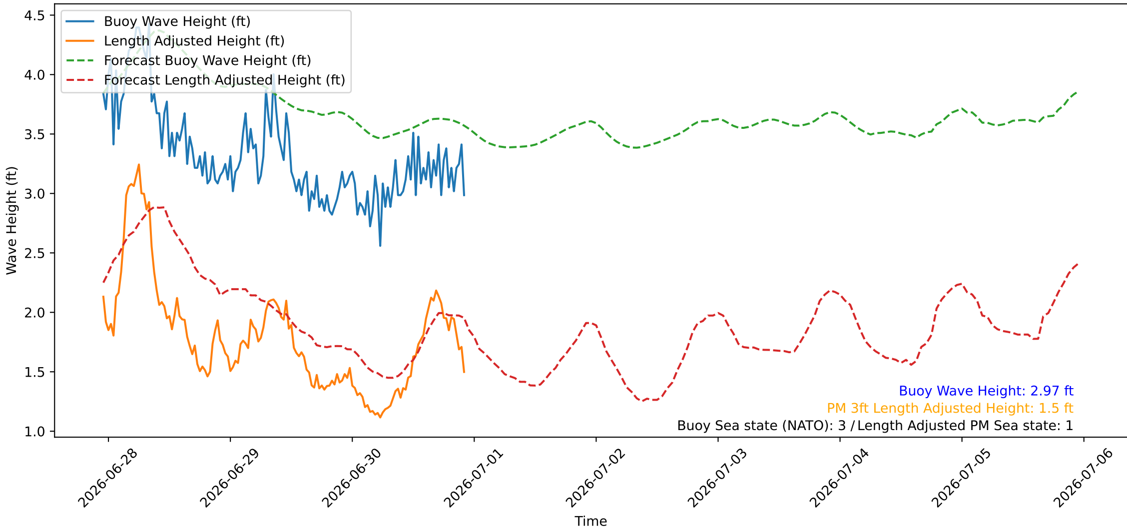
Wave Heights over Time for Oceanside Harbor at 2026-06-30 23:00:26
