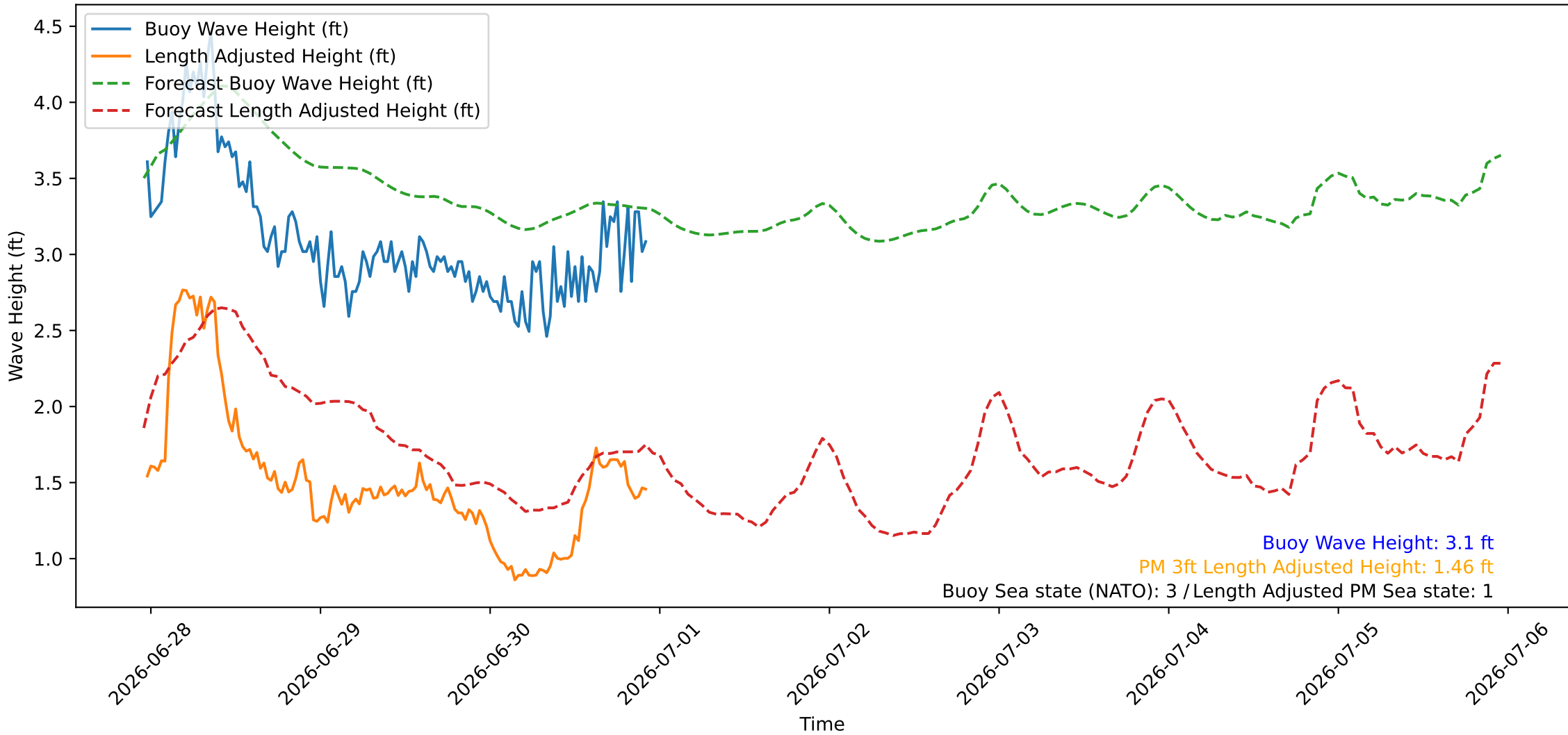
Wave Heights over Time for Red Beach at 2026-06-30 23:00:45
