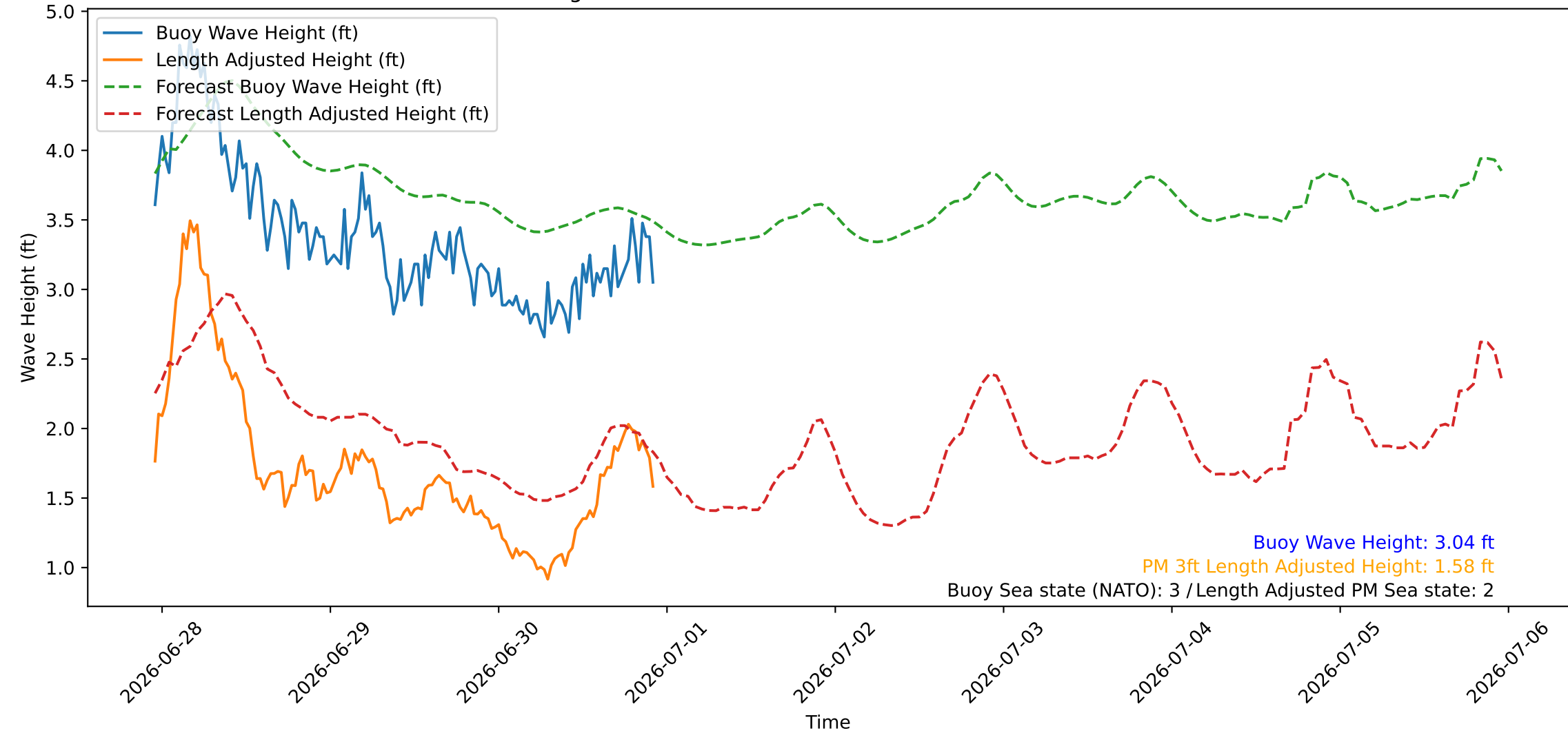
Wave Heights over Time for Green Beach at 2026-06-30 23:01:07
