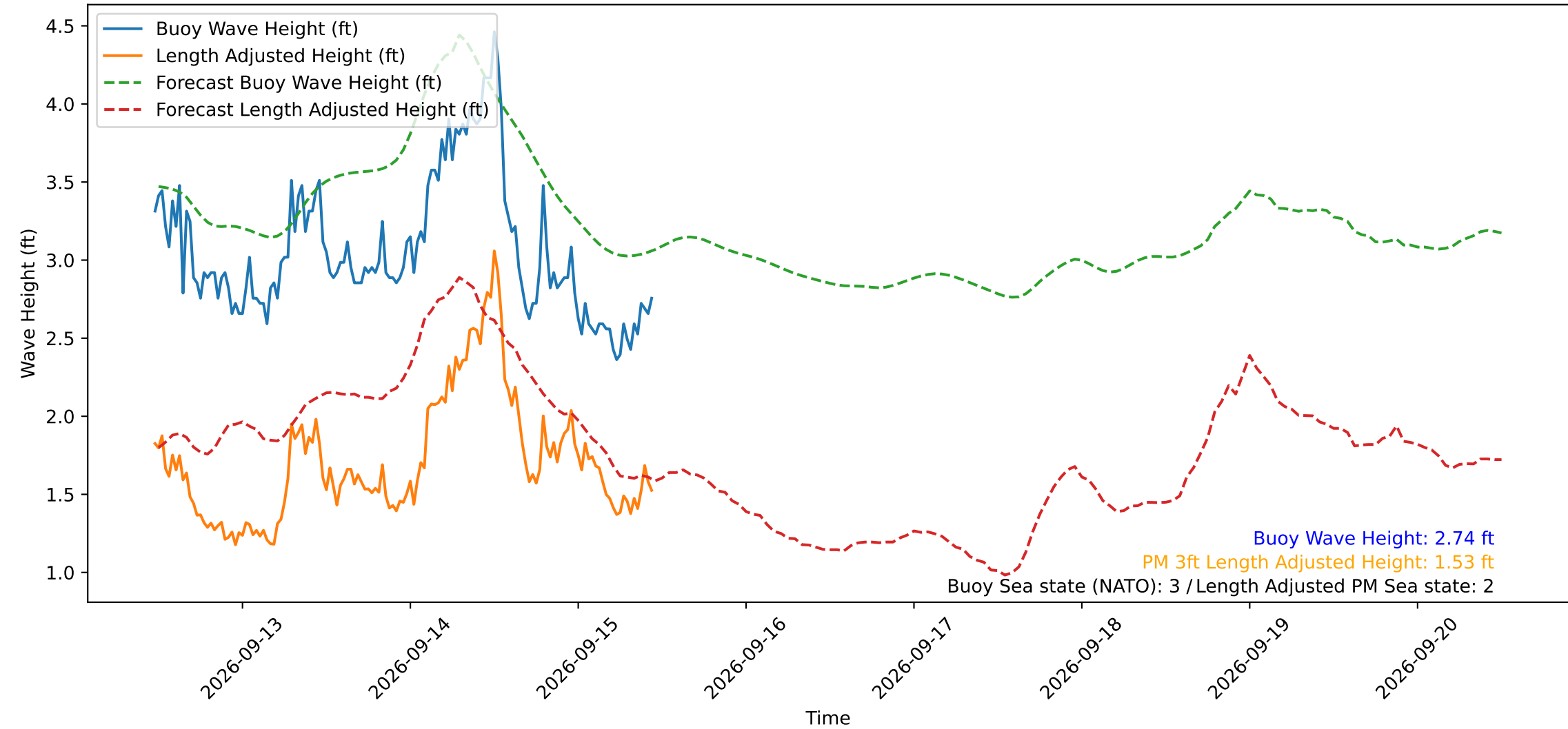
Wave Heights over Time for Oceanside Harbor at 2026-09-15 11:30:29
