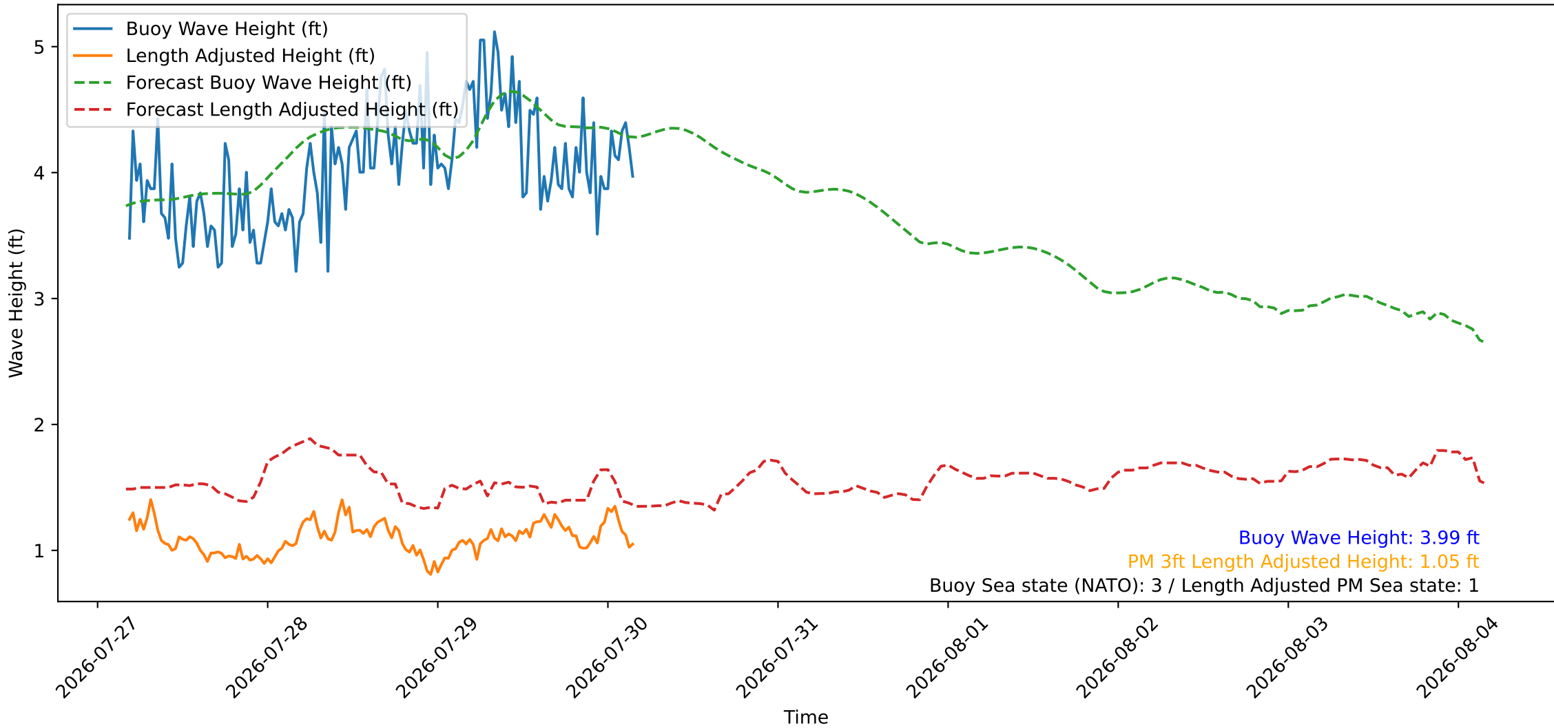
Wave Heights over Time for Red Beach at 2026-07-30 04:10:47
