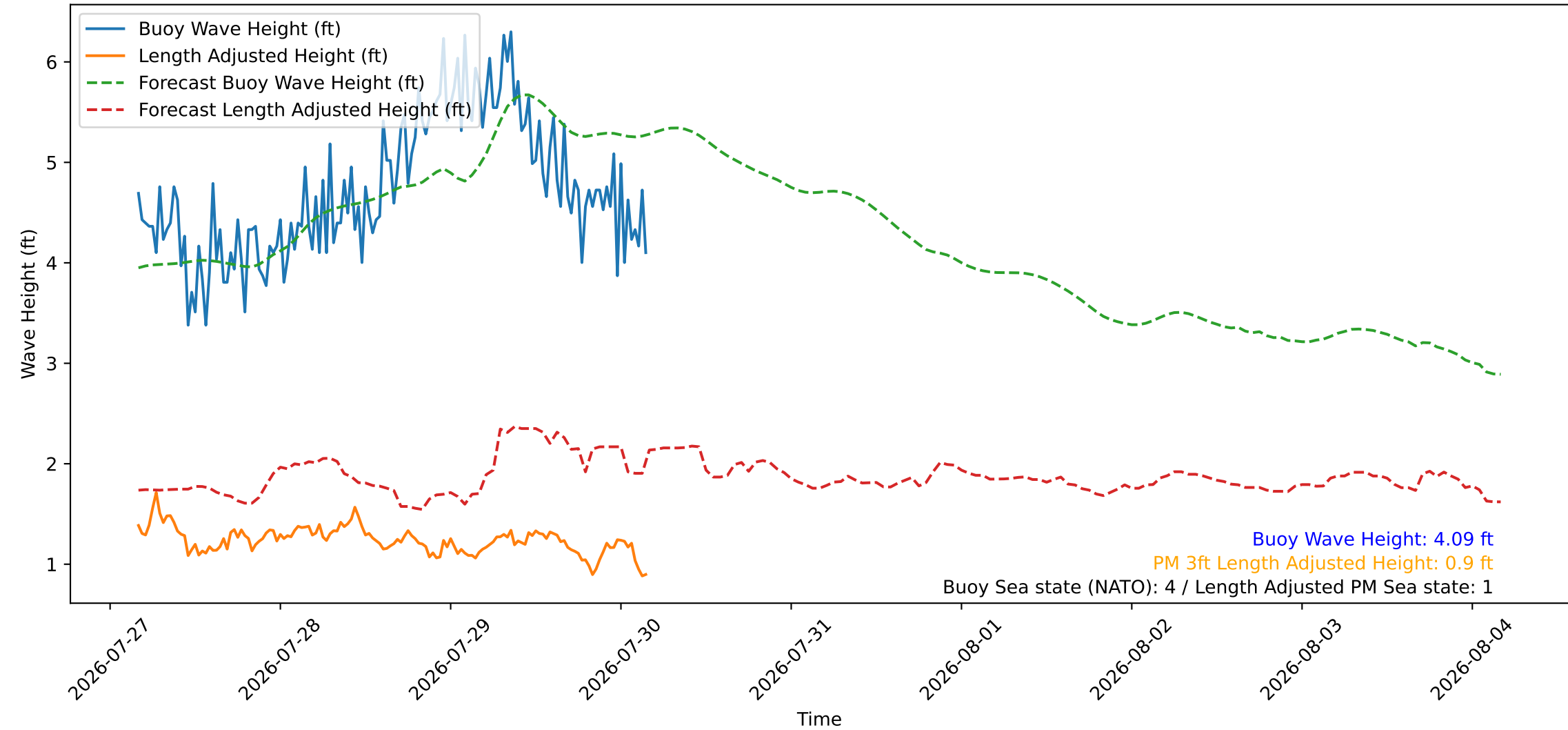
Wave Heights over Time for Green Beach at 2026-07-30 04:11:10
