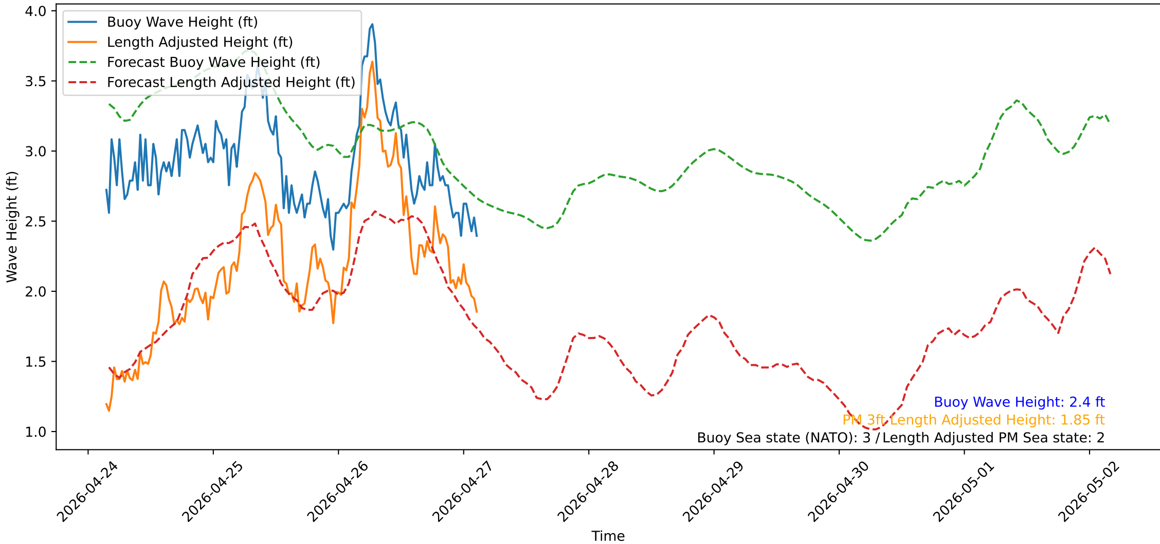
Wave Heights over Time for Oceanside Harbor at 2026-04-27 03:30:31
