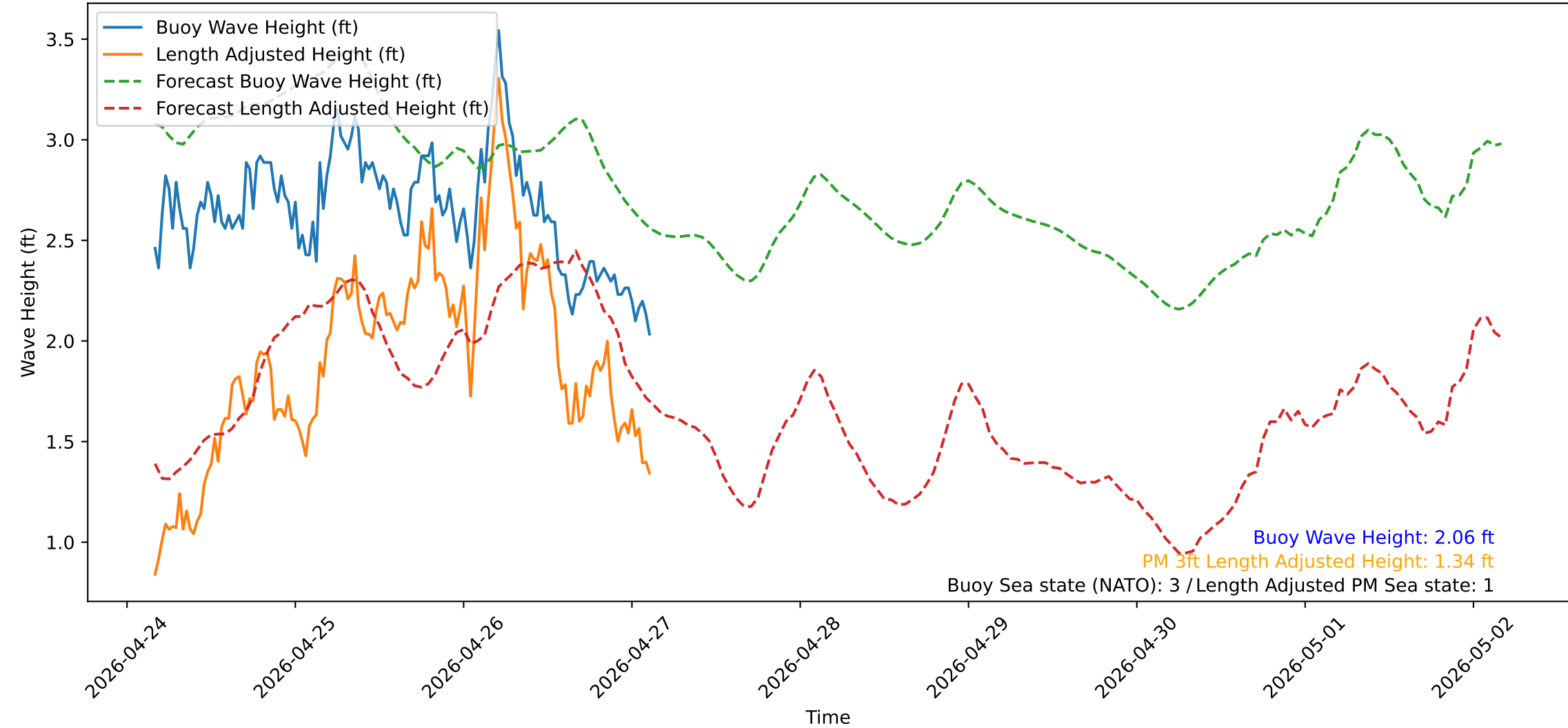
Wave Heights over Time for Red Beach at 2026-04-27 03:30:50
