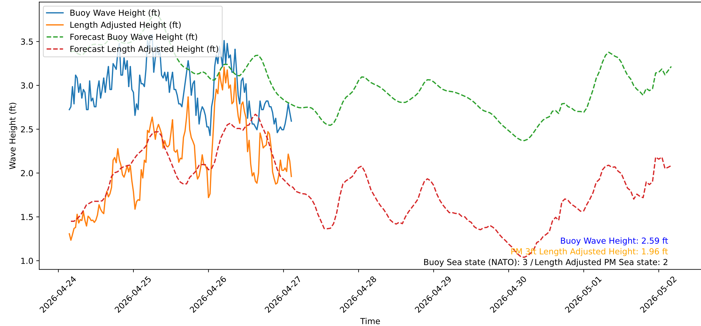
Wave Heights over Time for Green Beach at 2026-04-27 03:31:12
