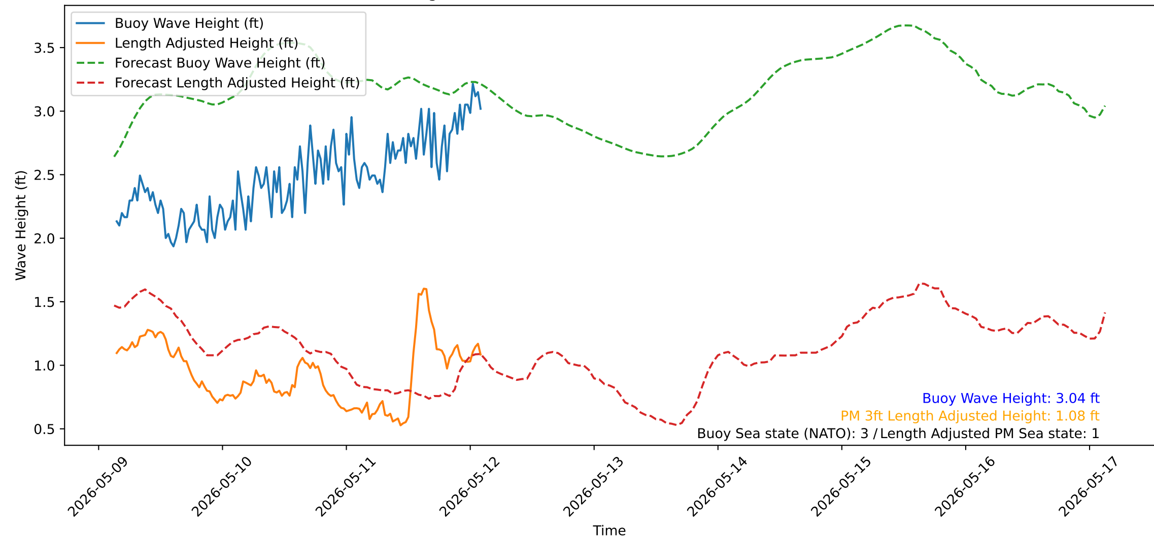
Wave Heights over Time for Red Beach at 2026-05-12 03:00:50
