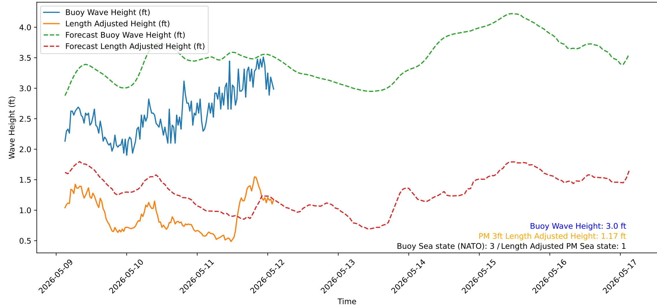
Wave Heights over Time for Green Beach at 2026-05-12 03:01:13
