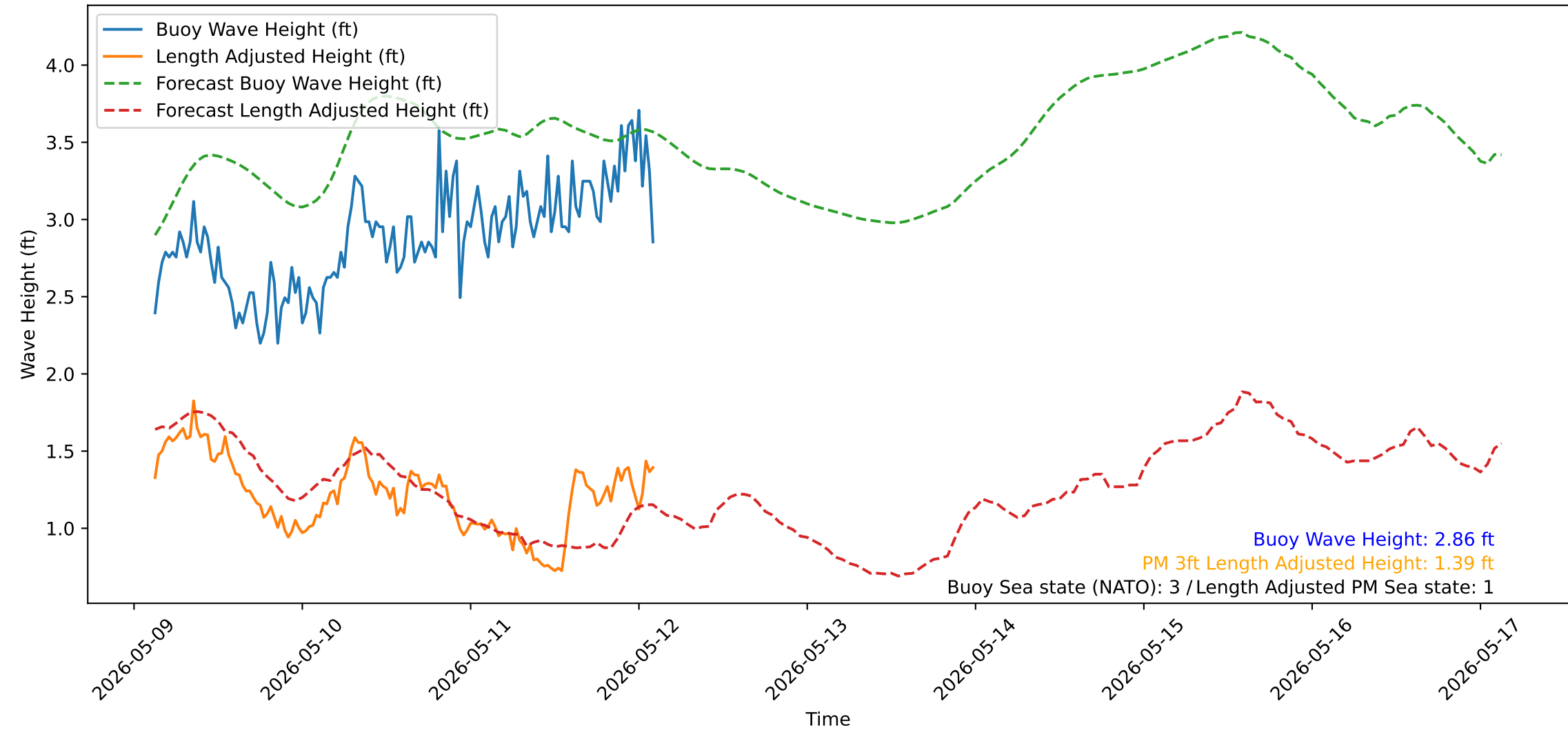
Wave Heights over Time for Oceanside Harbor at 2026-05-12 03:00:31
