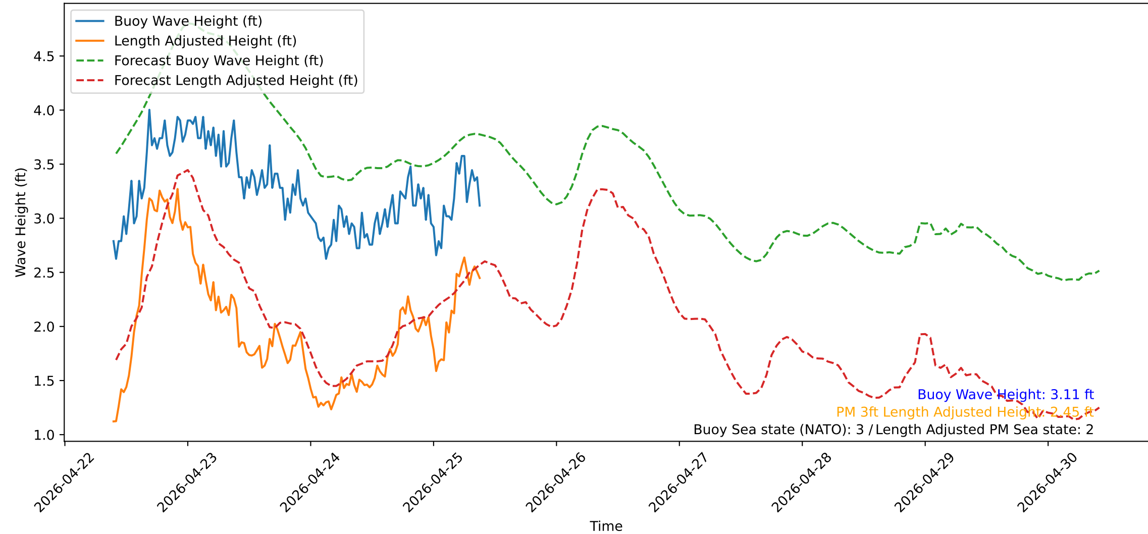
Wave Heights over Time for Green Beach at 2026-04-25 09:41:13
