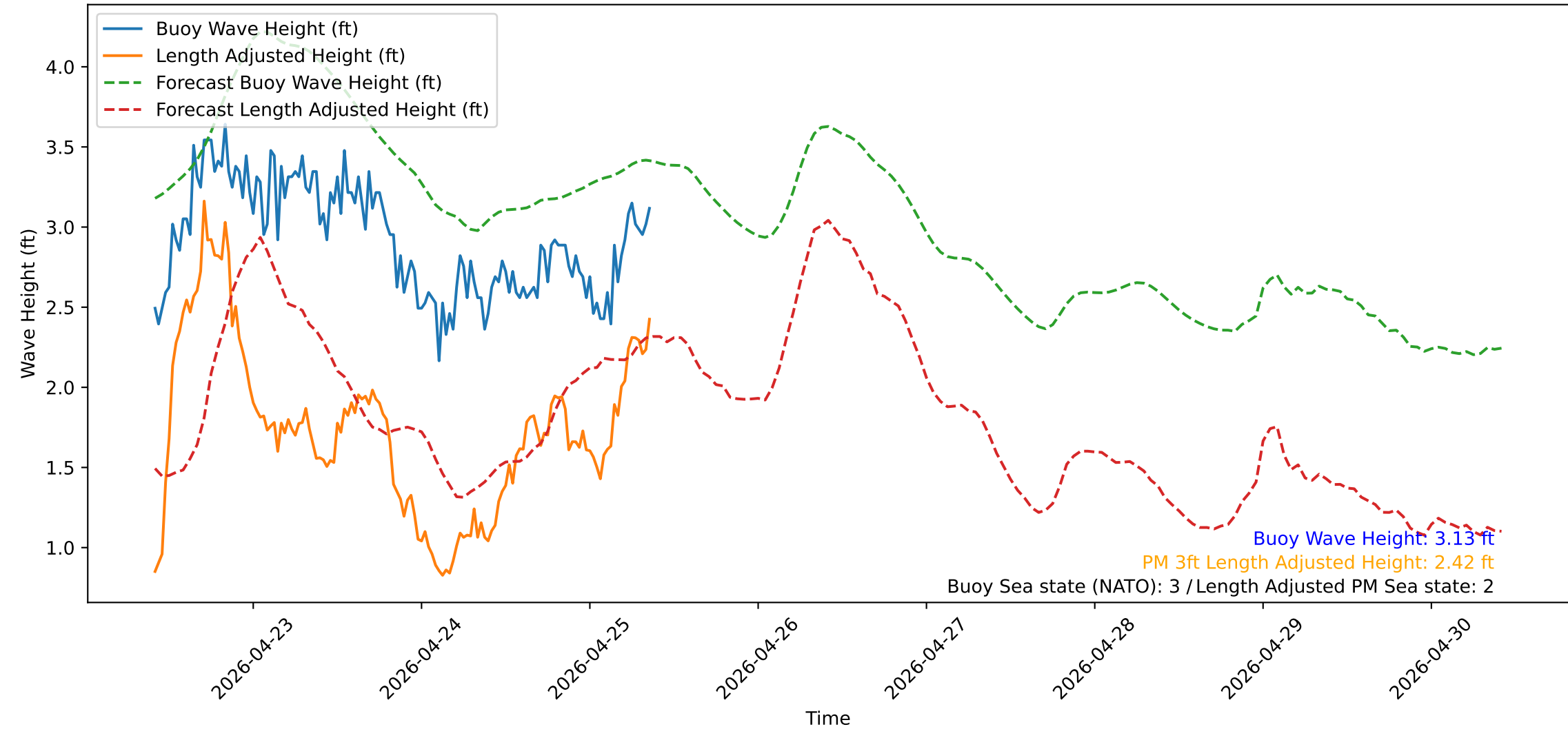
Wave Heights over Time for Red Beach at 2026-04-25 09:40:50
