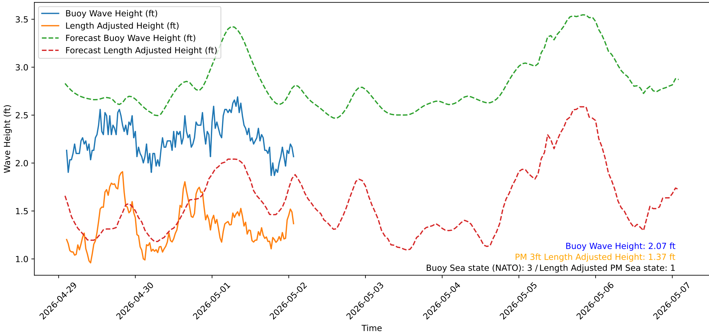
Wave Heights over Time for Oceanside Harbor at 2026-05-02 02:20:32
