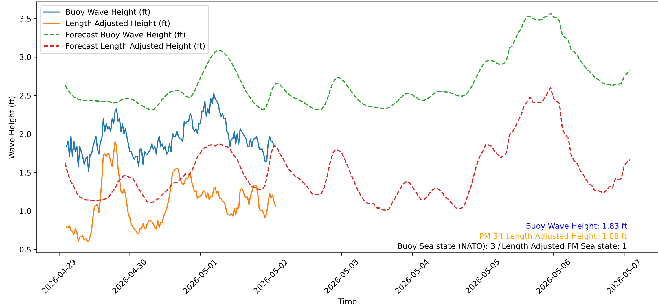
Wave Heights over Time for Red Beach at 2026-05-02 02:20:52
