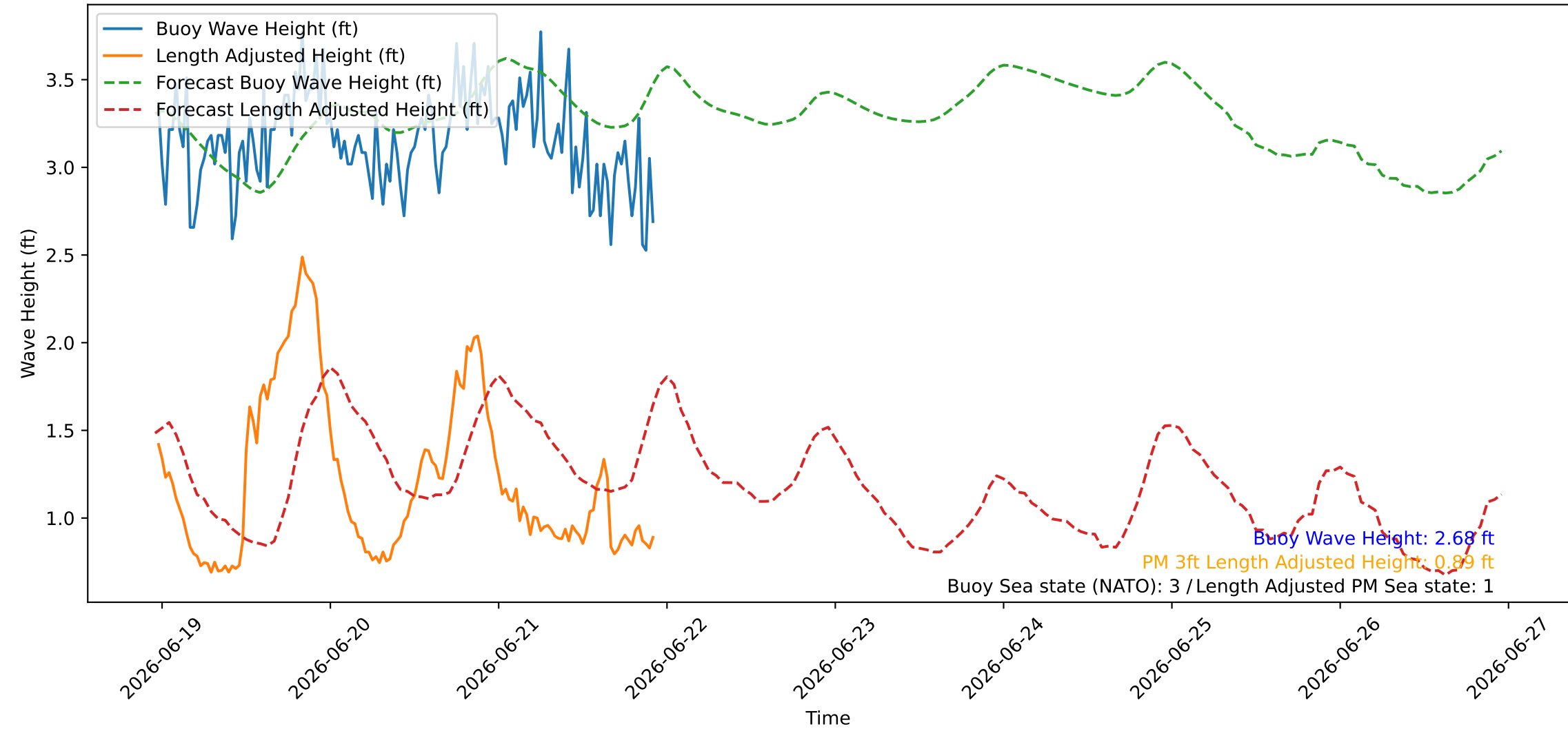
Wave Heights over Time for Red Beach at 2026-06-21 23:00:46
