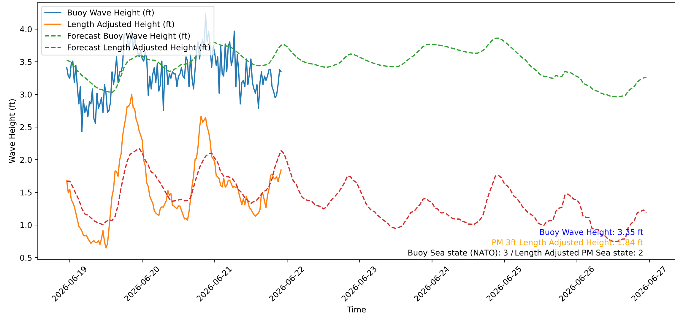
Wave Heights over Time for Green Beach at 2026-06-21 23:01:08
