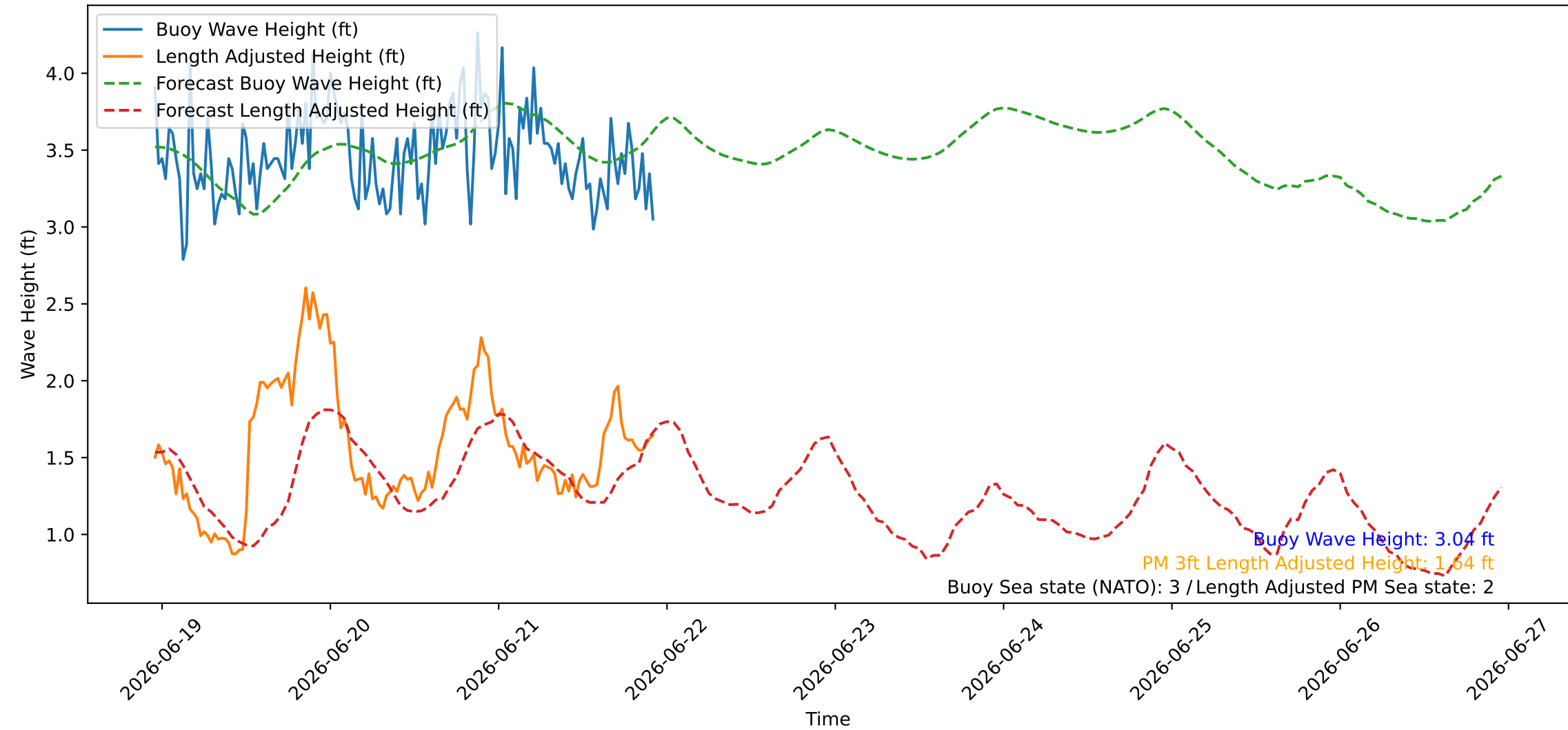
Wave Heights over Time for Oceanside Harbor at 2026-06-21 23:00:27
