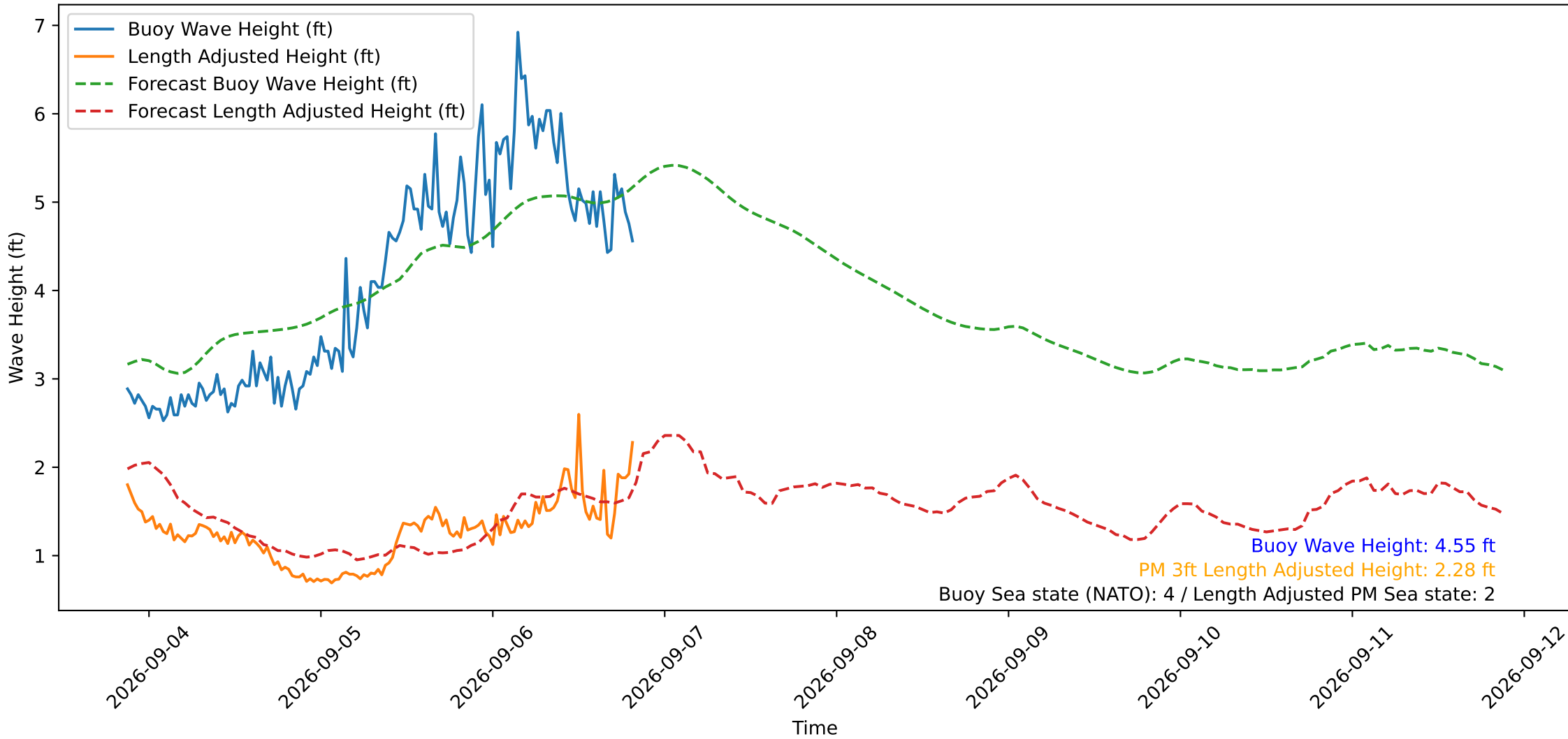
Wave Heights over Time for Red Beach at 2026-09-06 20:30:49
