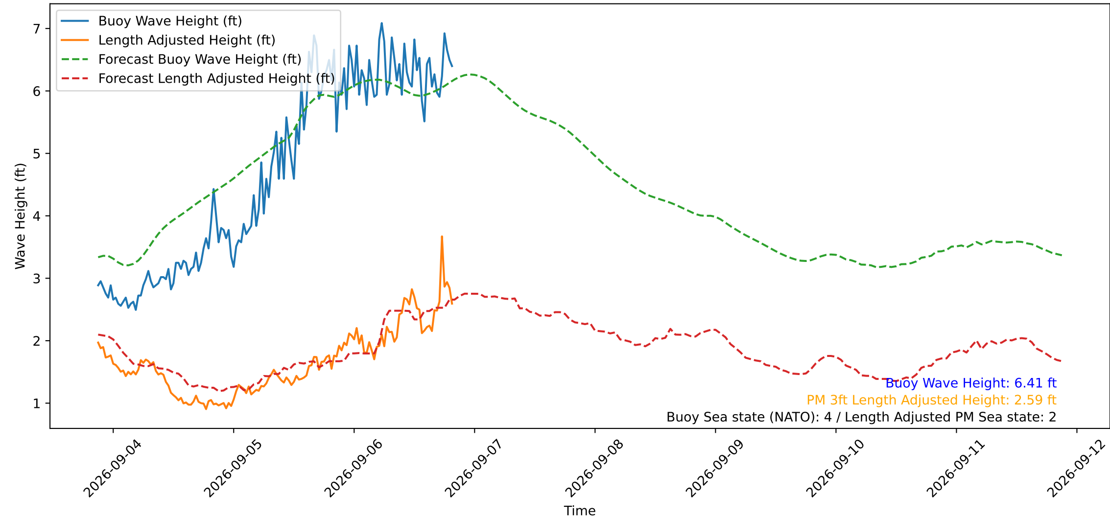
Wave Heights over Time for Green Beach at 2026-09-06 20:31:12
