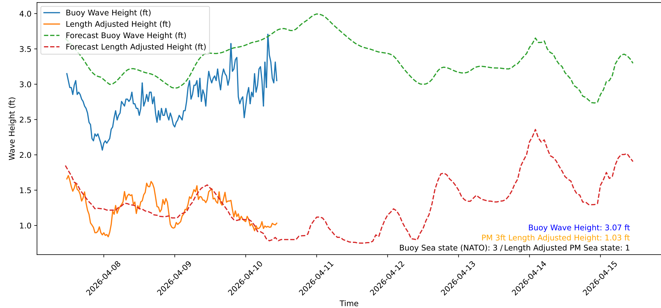
Wave Heights over Time for Red Beach at 2026-04-10 11:20:52
