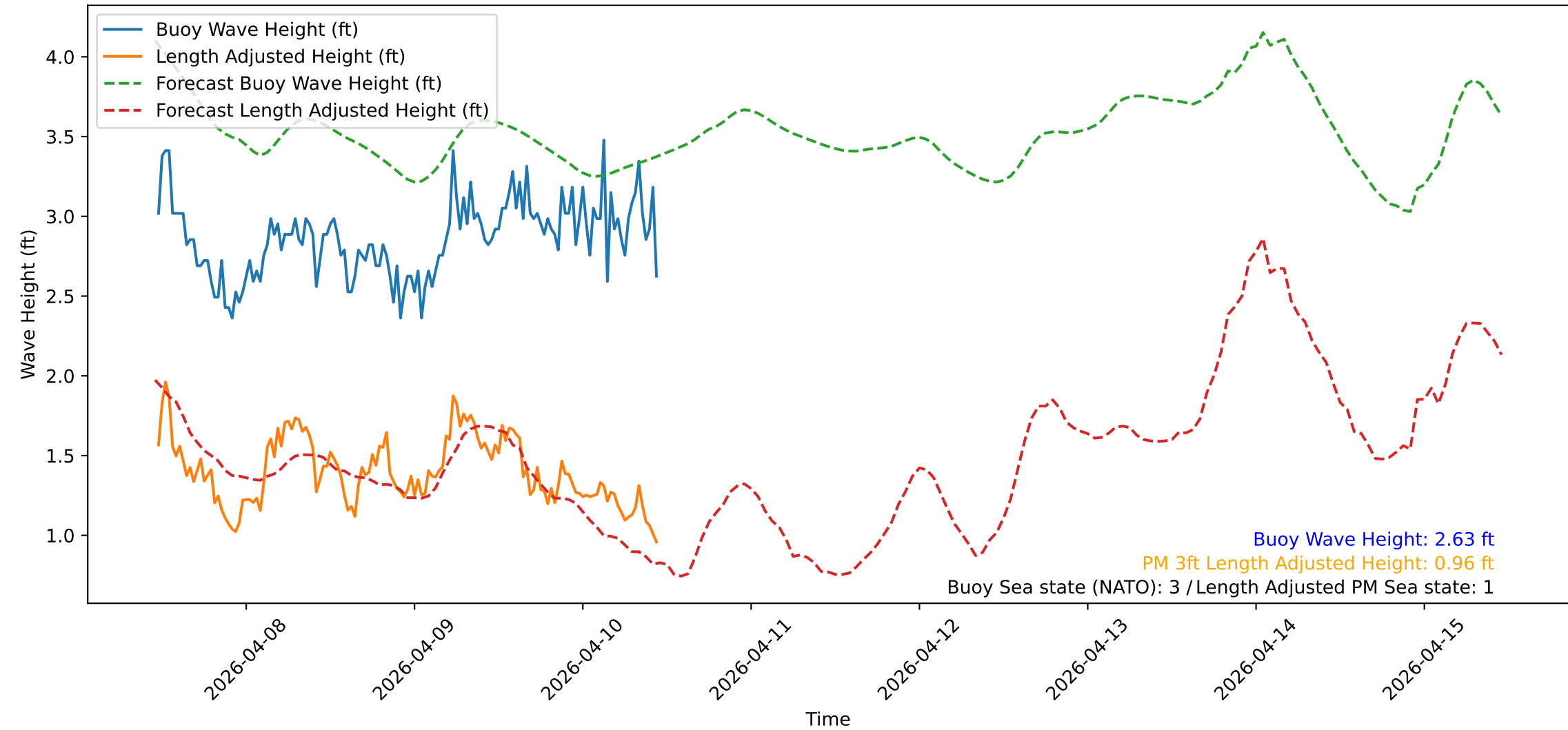
Wave Heights over Time for Green Beach at 2026-04-10 11:21:15
