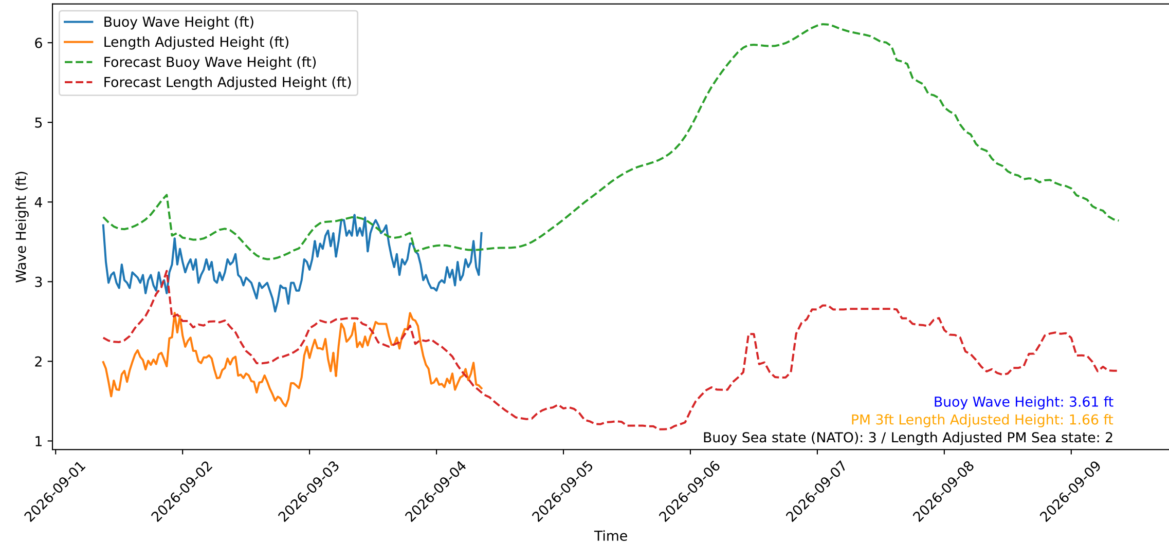
Wave Heights over Time for Oceanside Harbor at 2026-09-04 09:10:30
