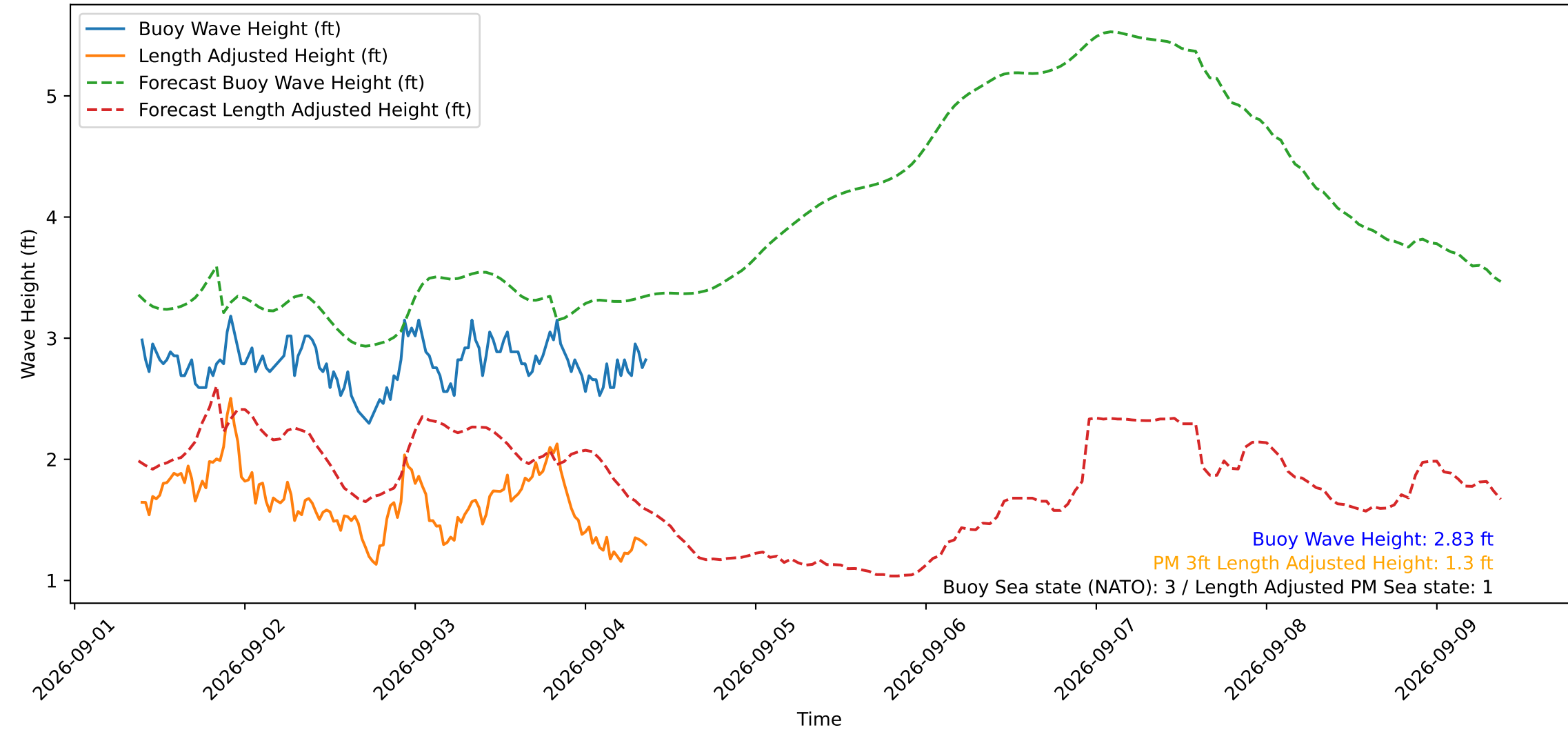
Wave Heights over Time for Red Beach at 2026-09-04 09:10:50
