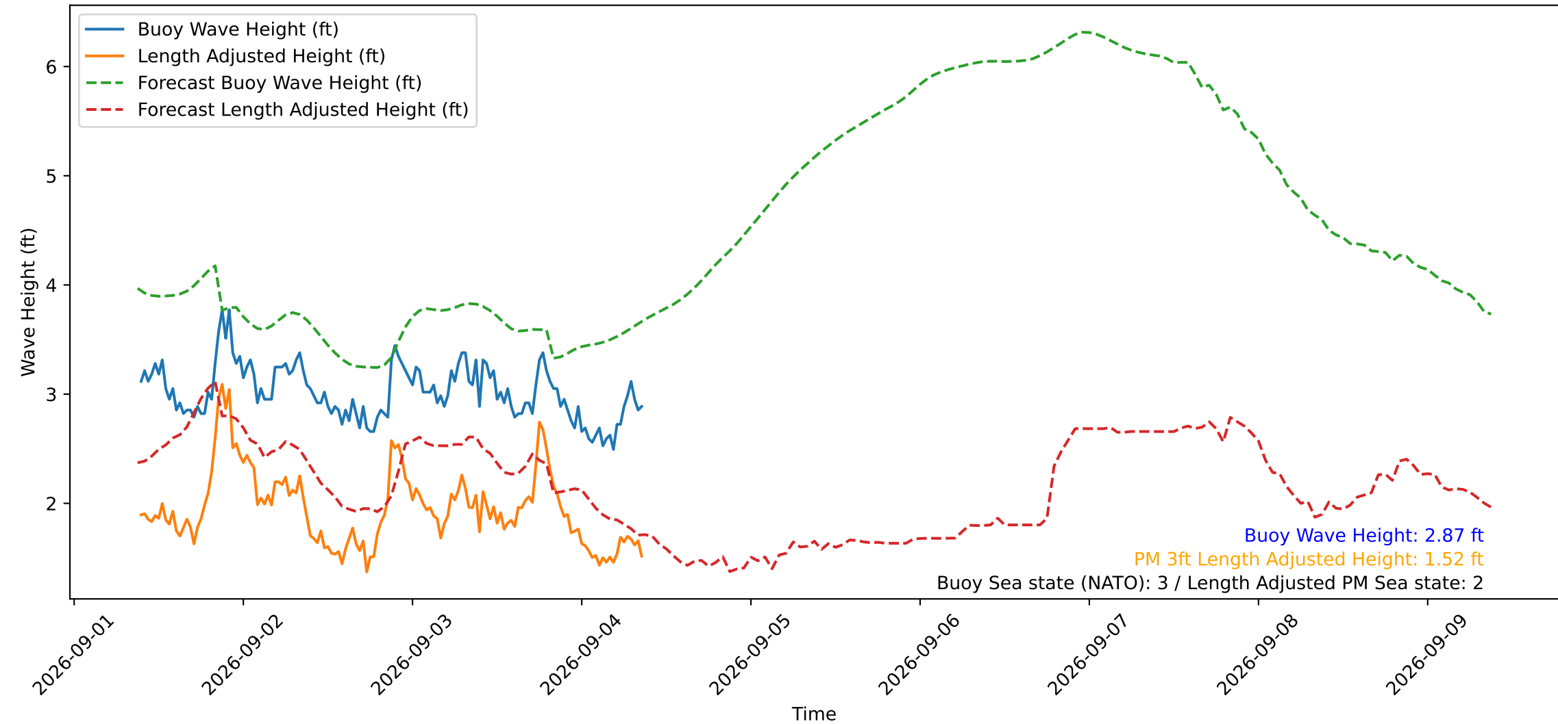
Wave Heights over Time for Green Beach at 2026-09-04 09:11:14
