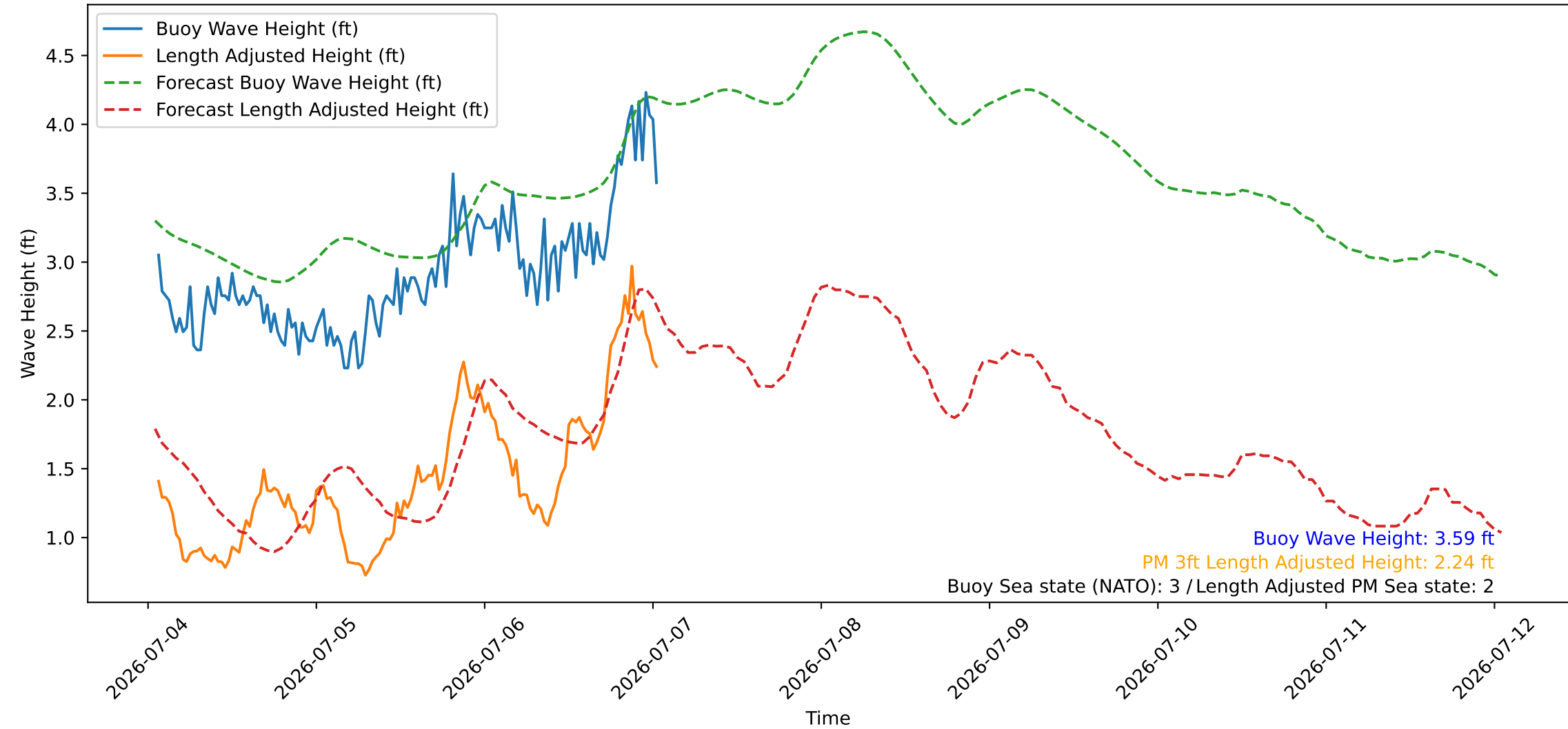
Wave Heights over Time for Red Beach at 2026-07-07 01:20:47
