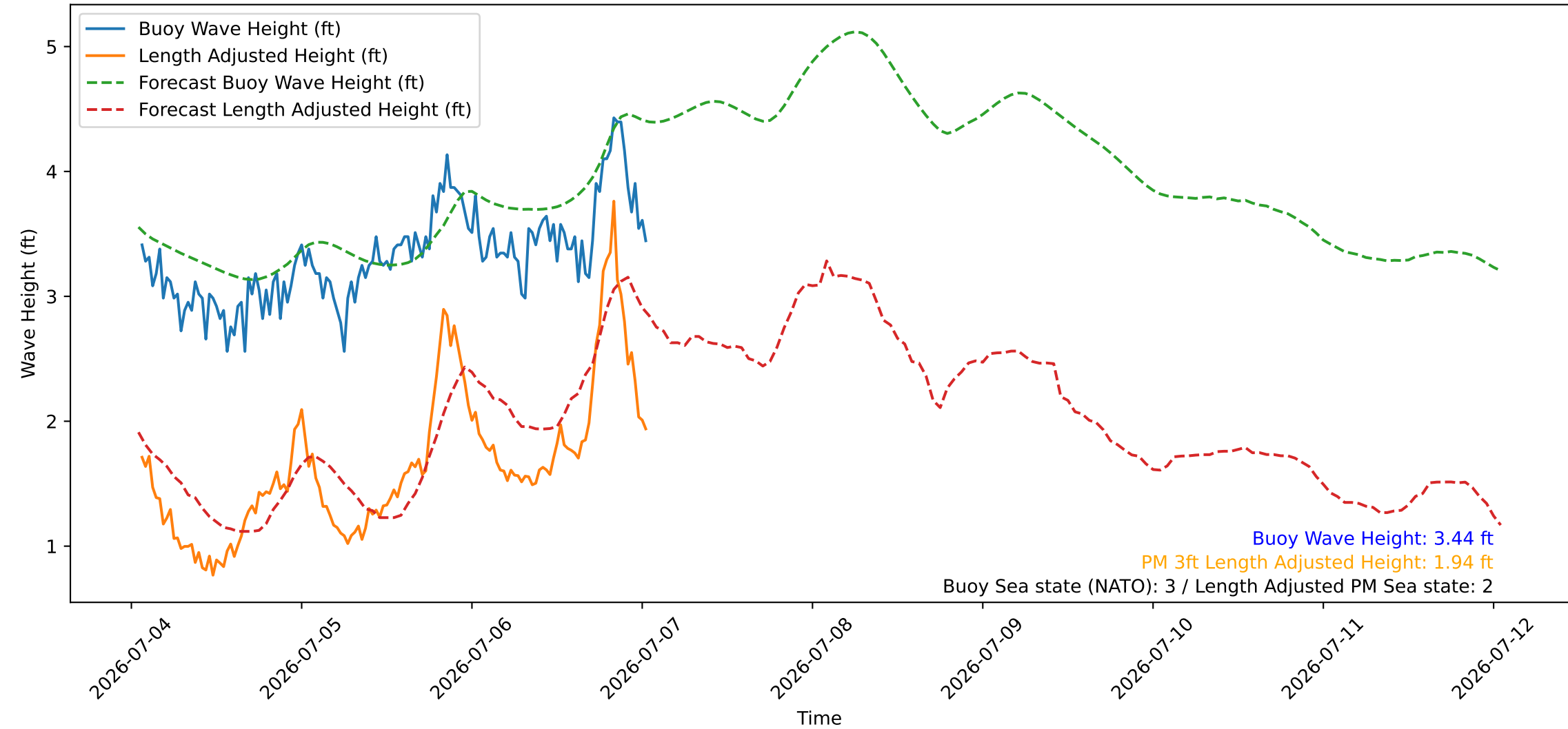
Wave Heights over Time for Green Beach at 2026-07-07 01:21:09
