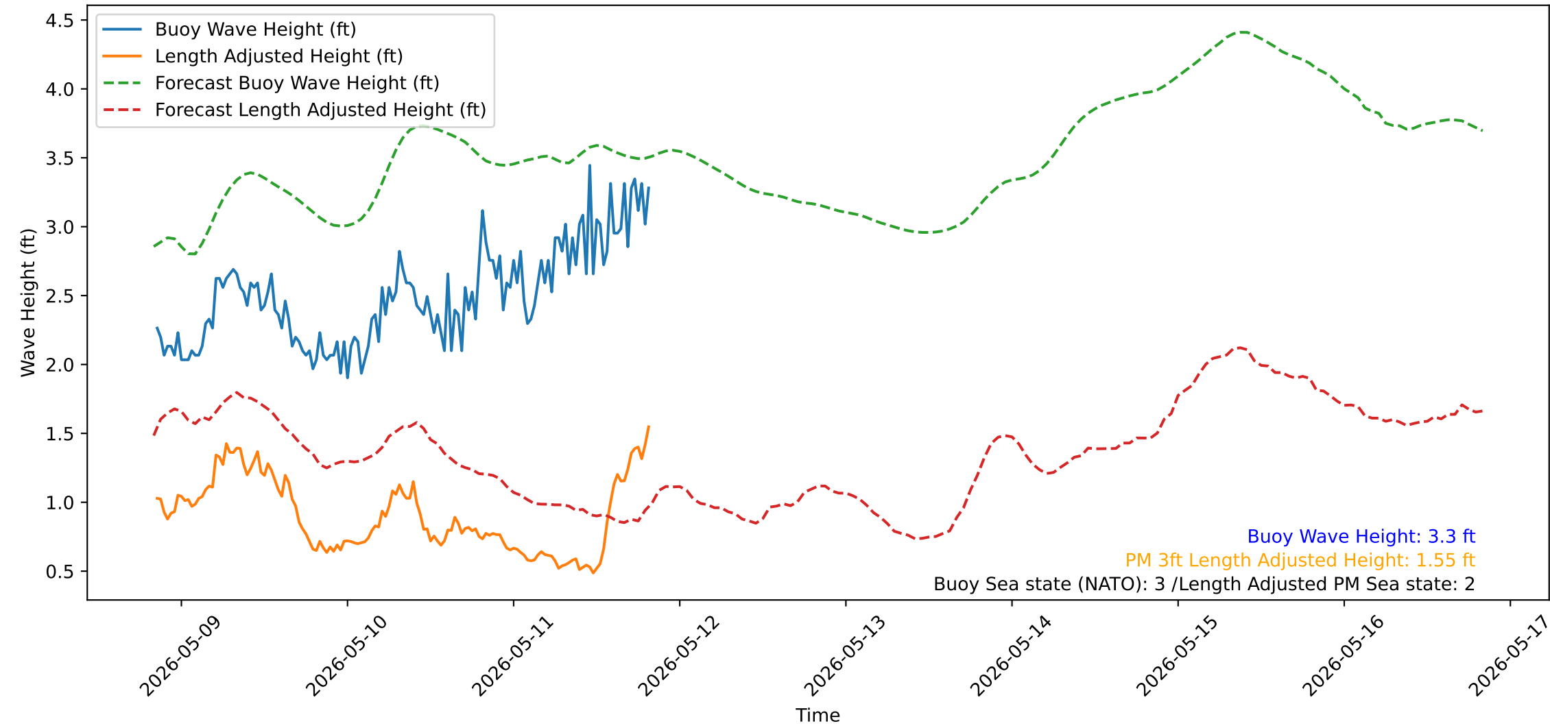
Wave Heights over Time for Green Beach at 2026-05-11 20:21:14
