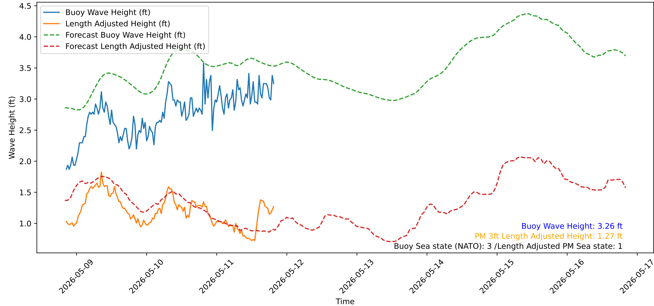
Wave Heights over Time for Oceanside Harbor at 2026-05-11 20:20:31
