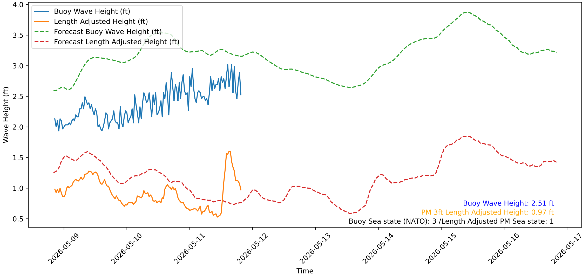
Wave Heights over Time for Red Beach at 2026-05-11 20:20:51
