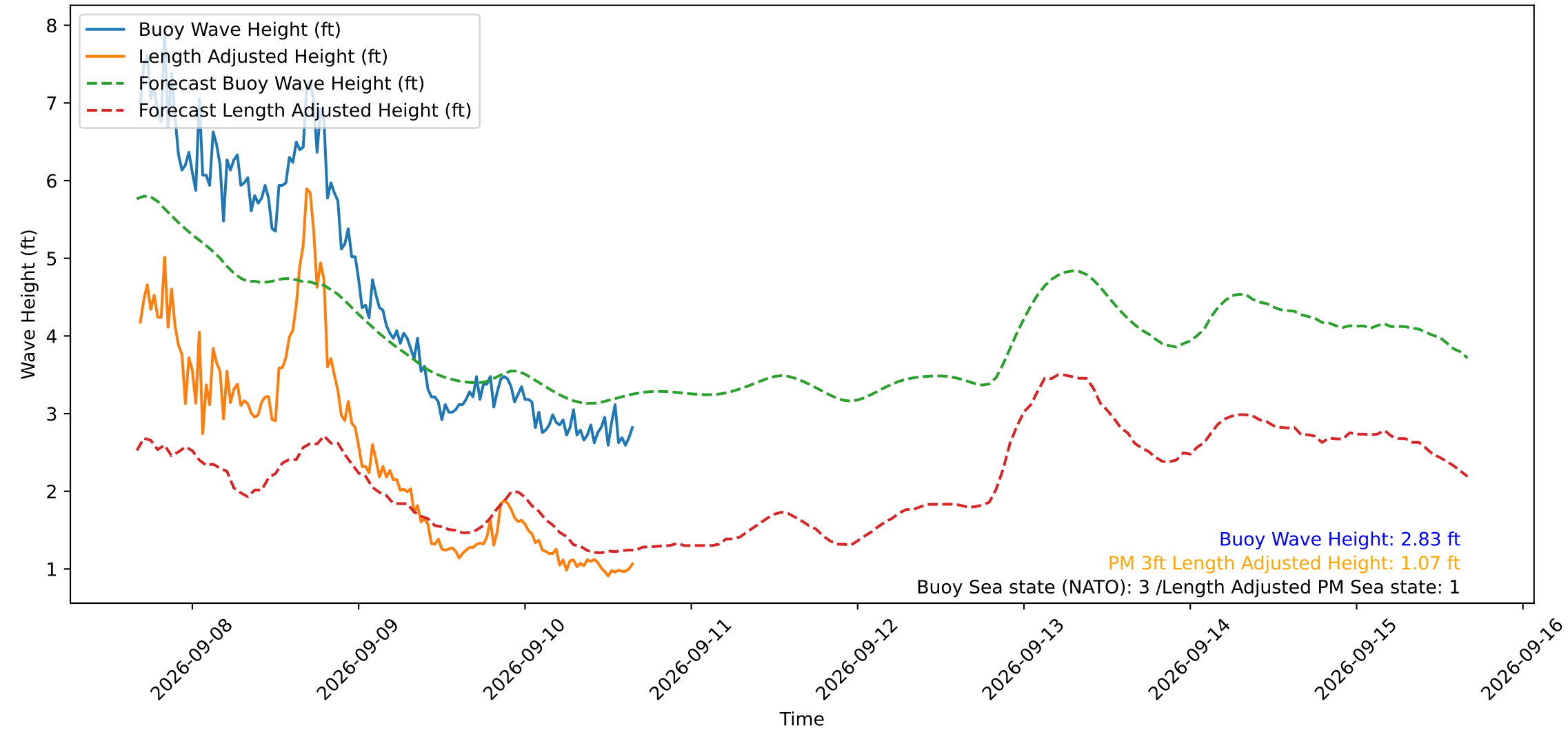
Wave Heights over Time for Green Beach at 2026-09-10 16:21:14
