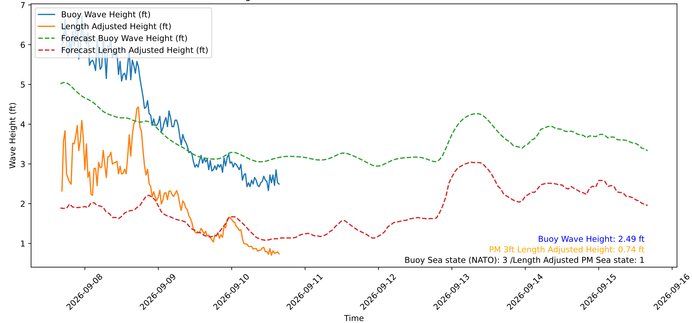
Wave Heights over Time for Red Beach at 2026-09-10 16:20:51
