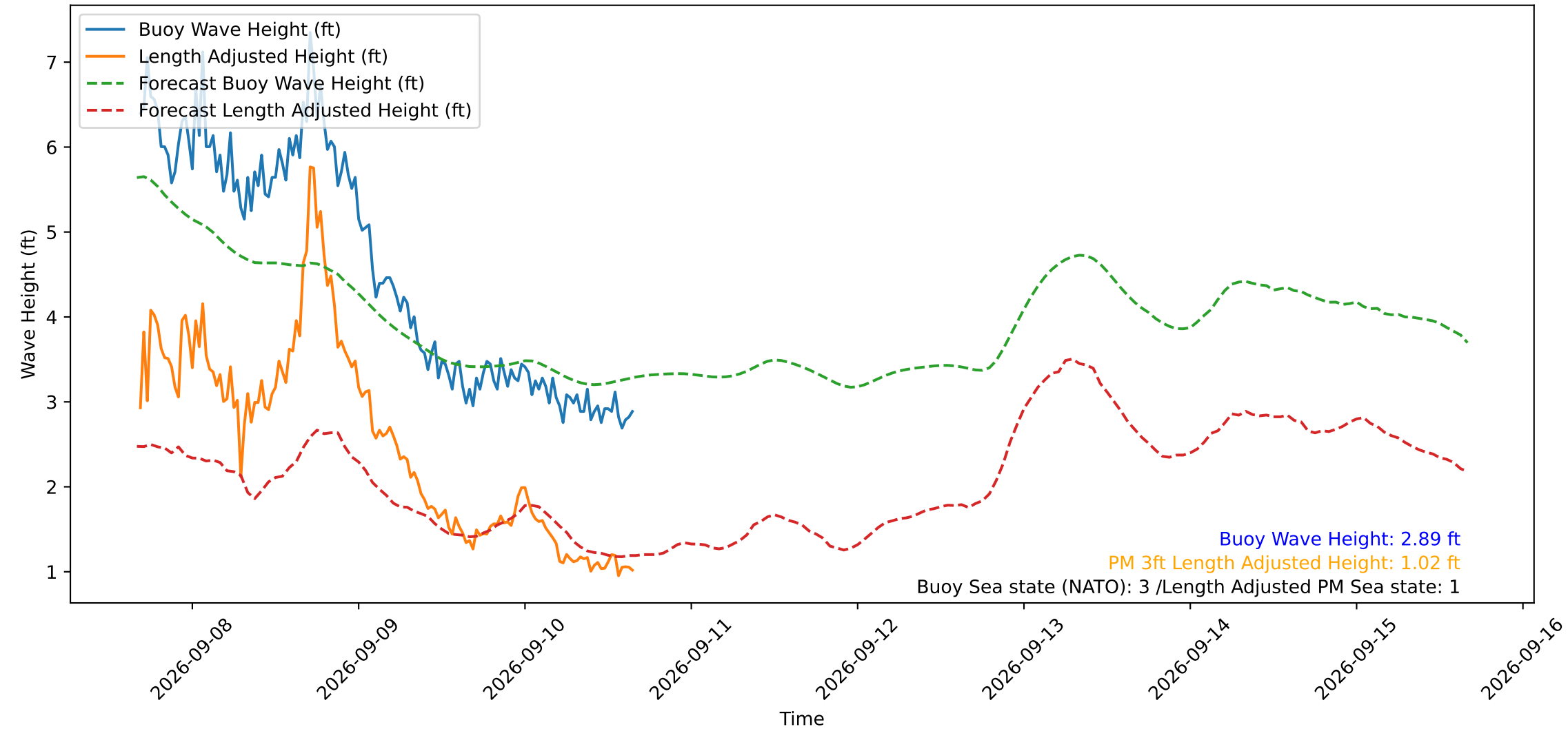
Wave Heights over Time for Oceanside Harbor at 2026-09-10 16:20:30
