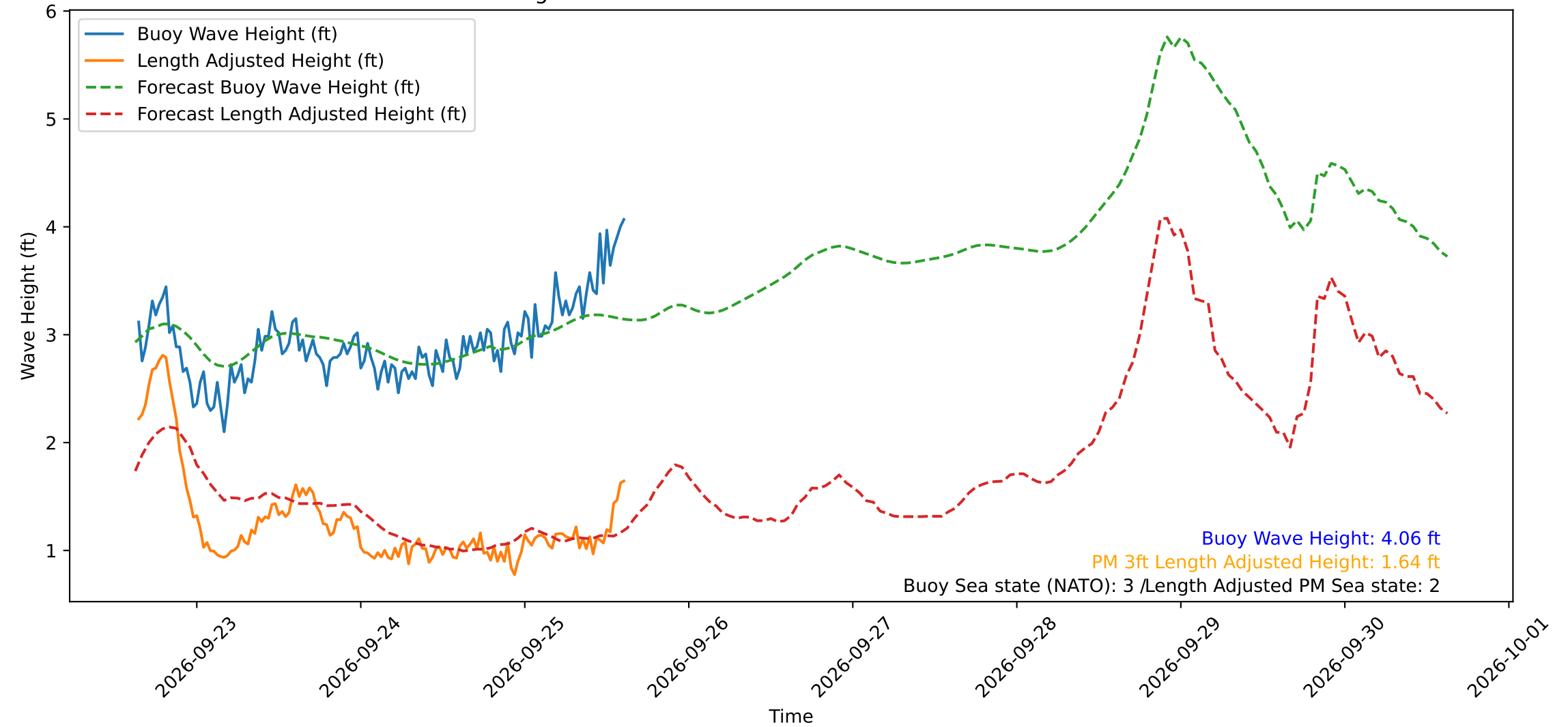
Wave Heights over Time for Green Beach at 2026-09-25 15:11:11
