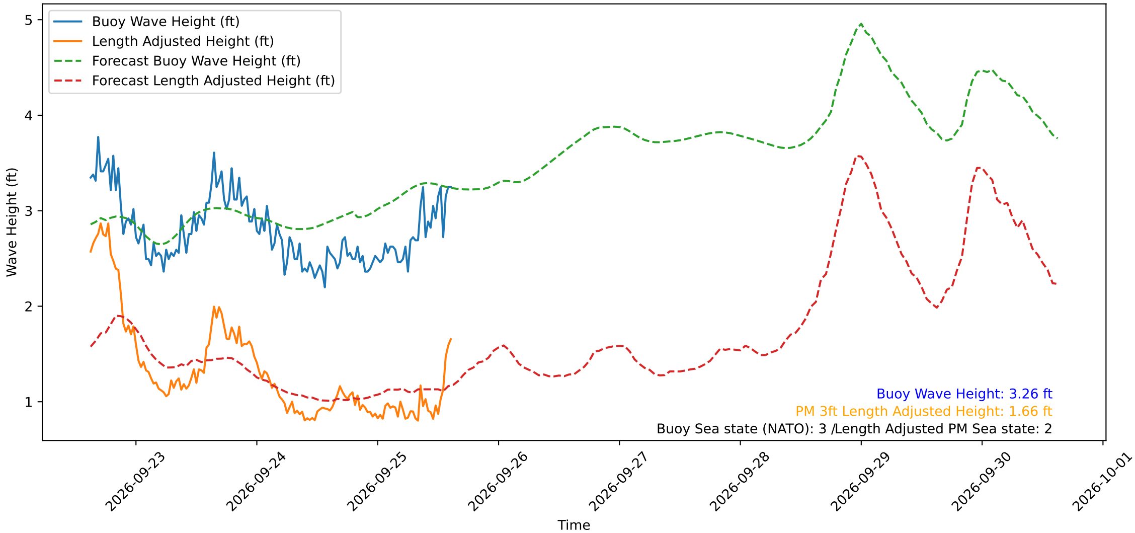
Wave Heights over Time for Oceanside Harbor at 2026-09-25 15:10:29
