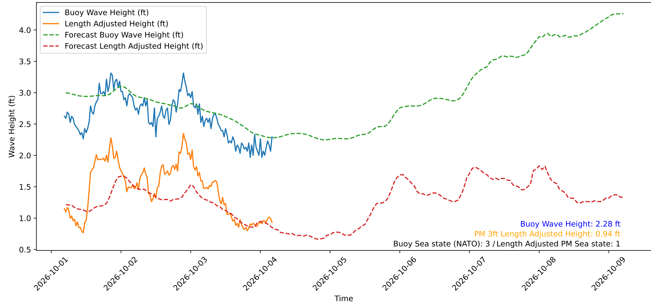
Wave Heights over Time for Oceanside Harbor at 2026-10-04 04:30:29
