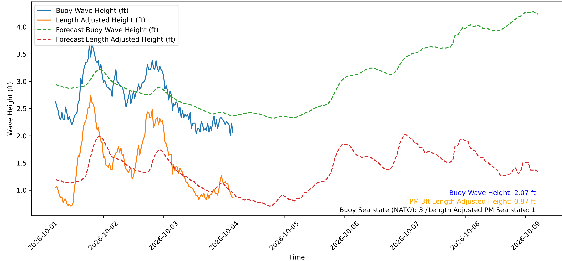
Wave Heights over Time for Green Beach at 2026-10-04 04:31:11
