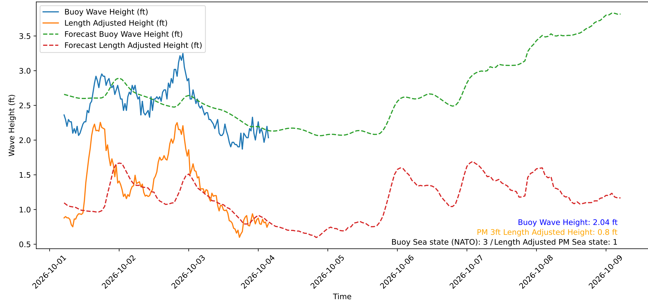
Wave Heights over Time for Red Beach at 2026-10-04 04:30:49
