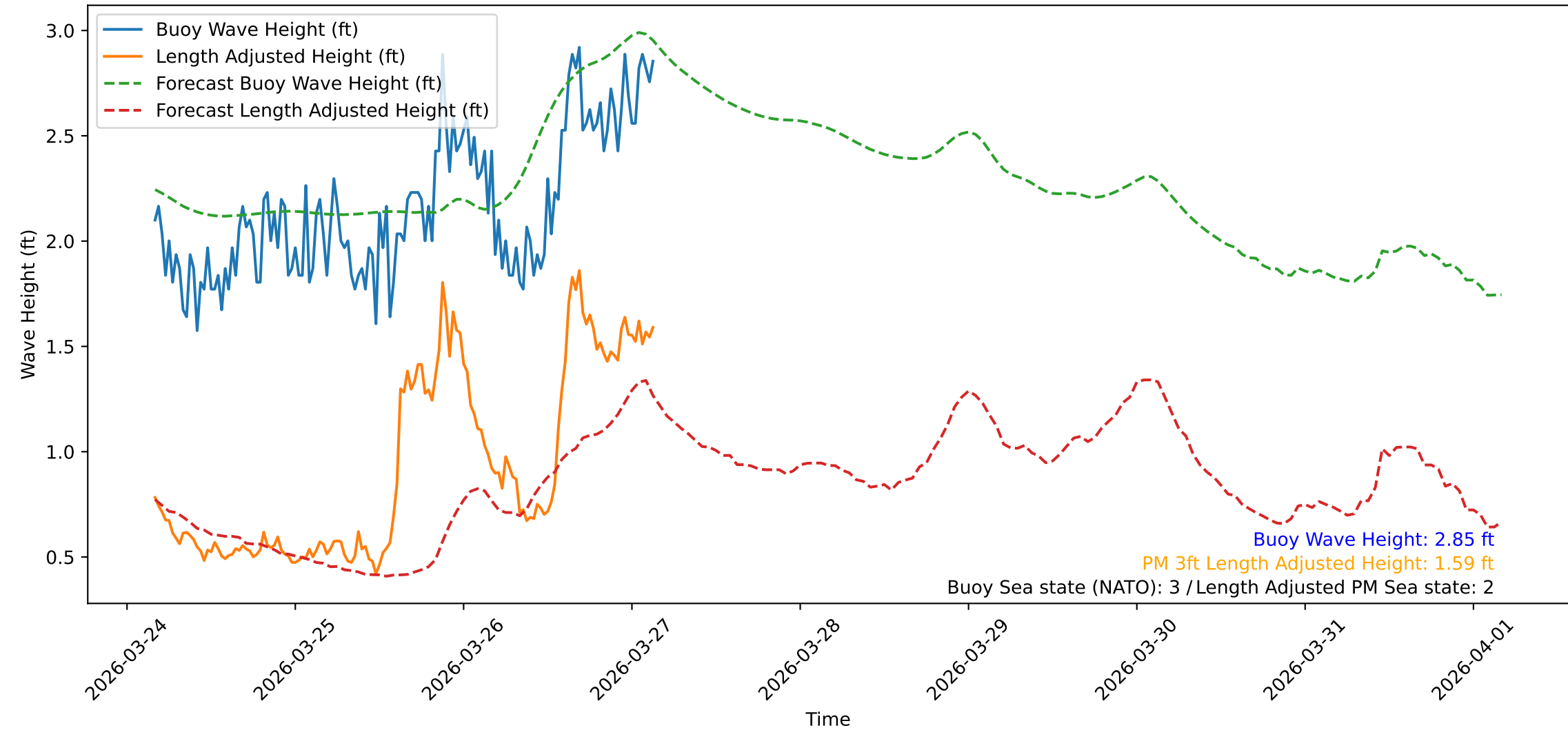
Wave Heights over Time for Oceanside Harbor at 2026-03-27 03:50:31
