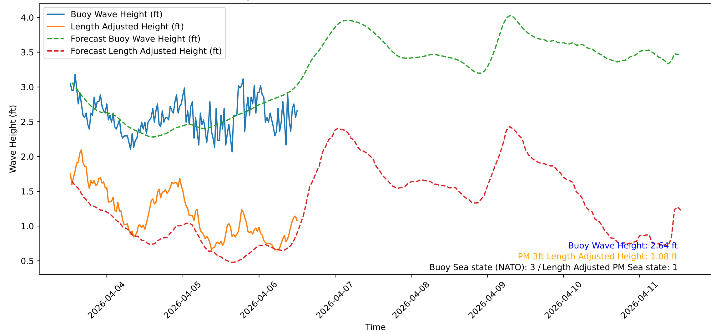
Wave Heights over Time for Oceanside Harbor at 2026-04-06 12:40:32
