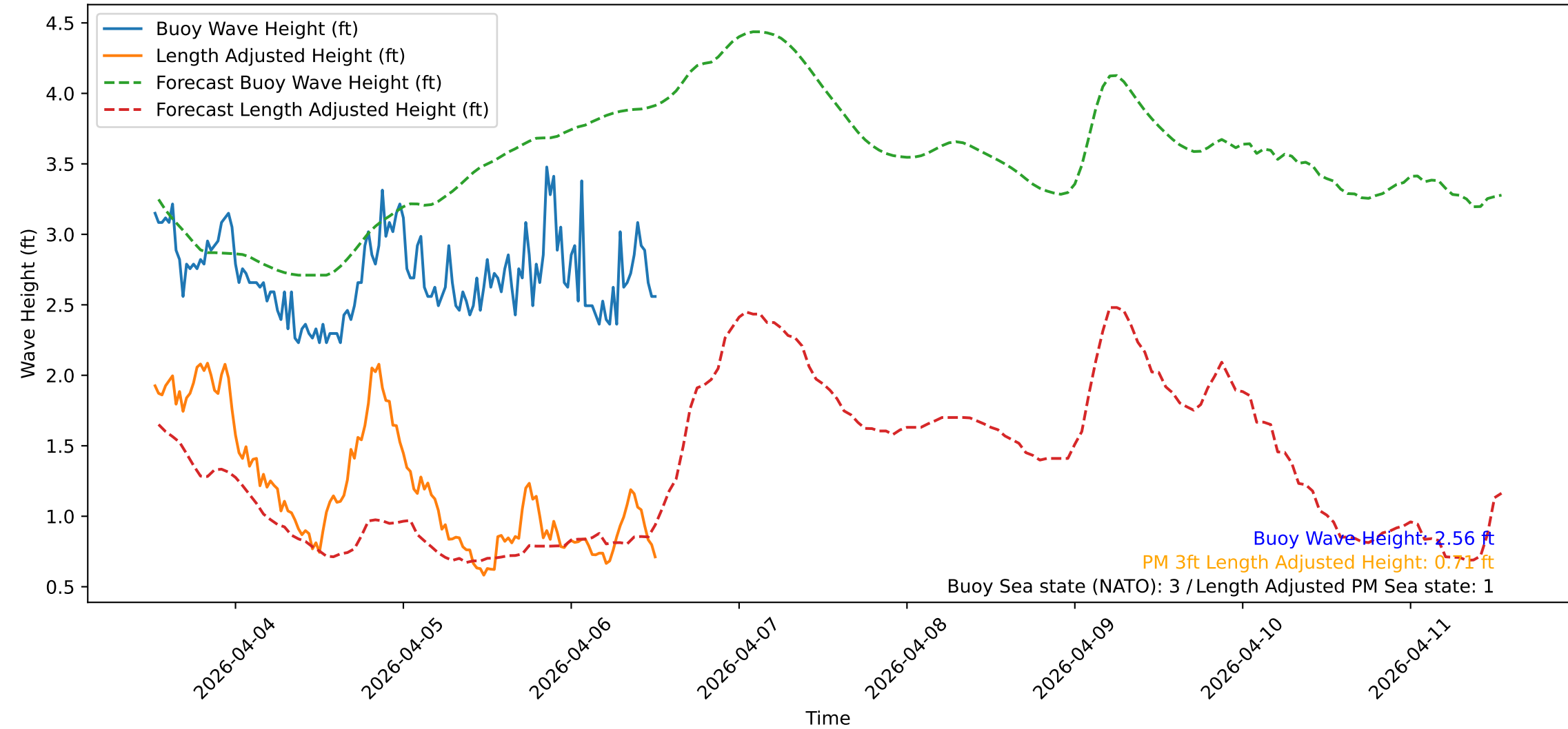
Wave Heights over Time for Green Beach at 2026-04-06 12:41:10
