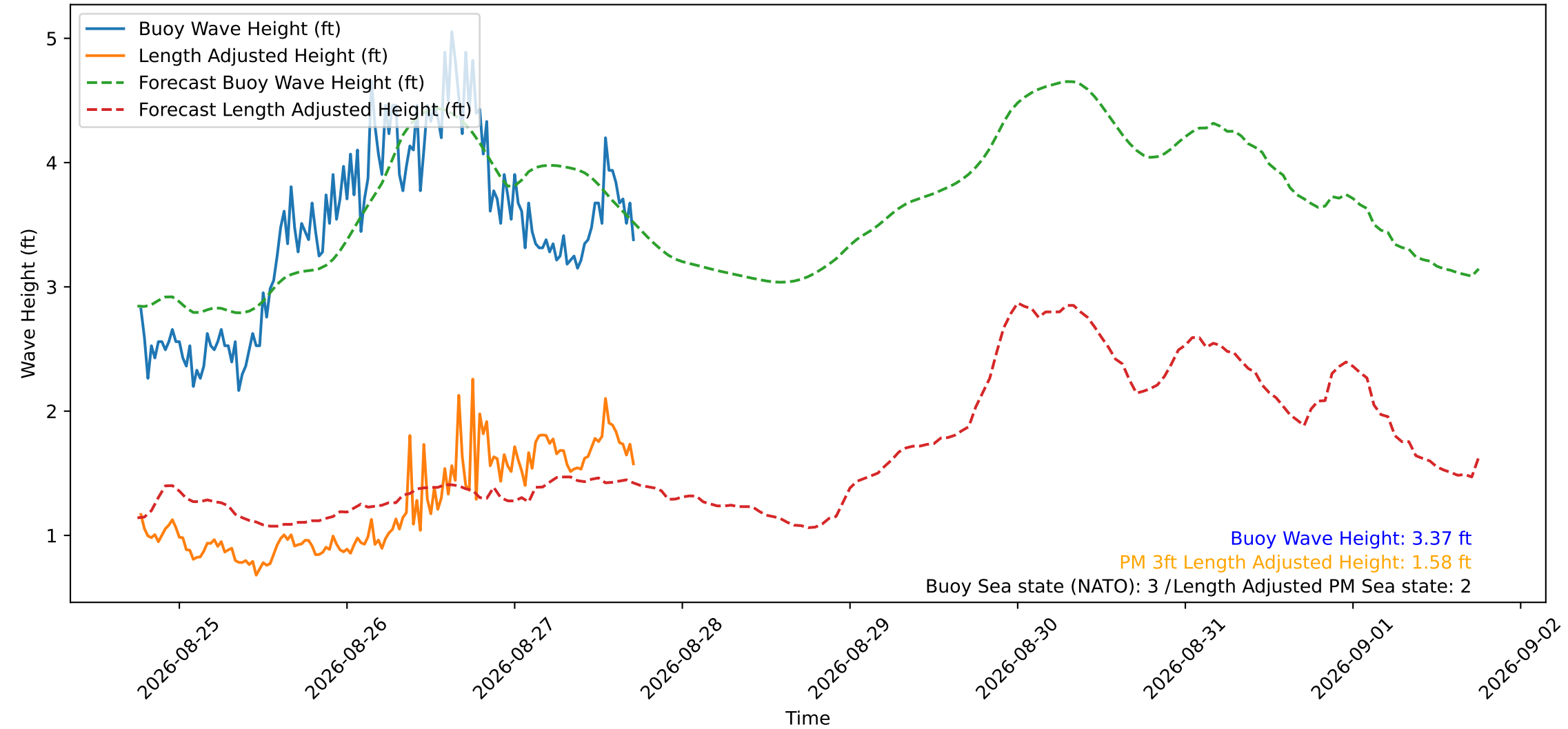
Wave Heights over Time for Red Beach at 2026-08-27 18:00:50
