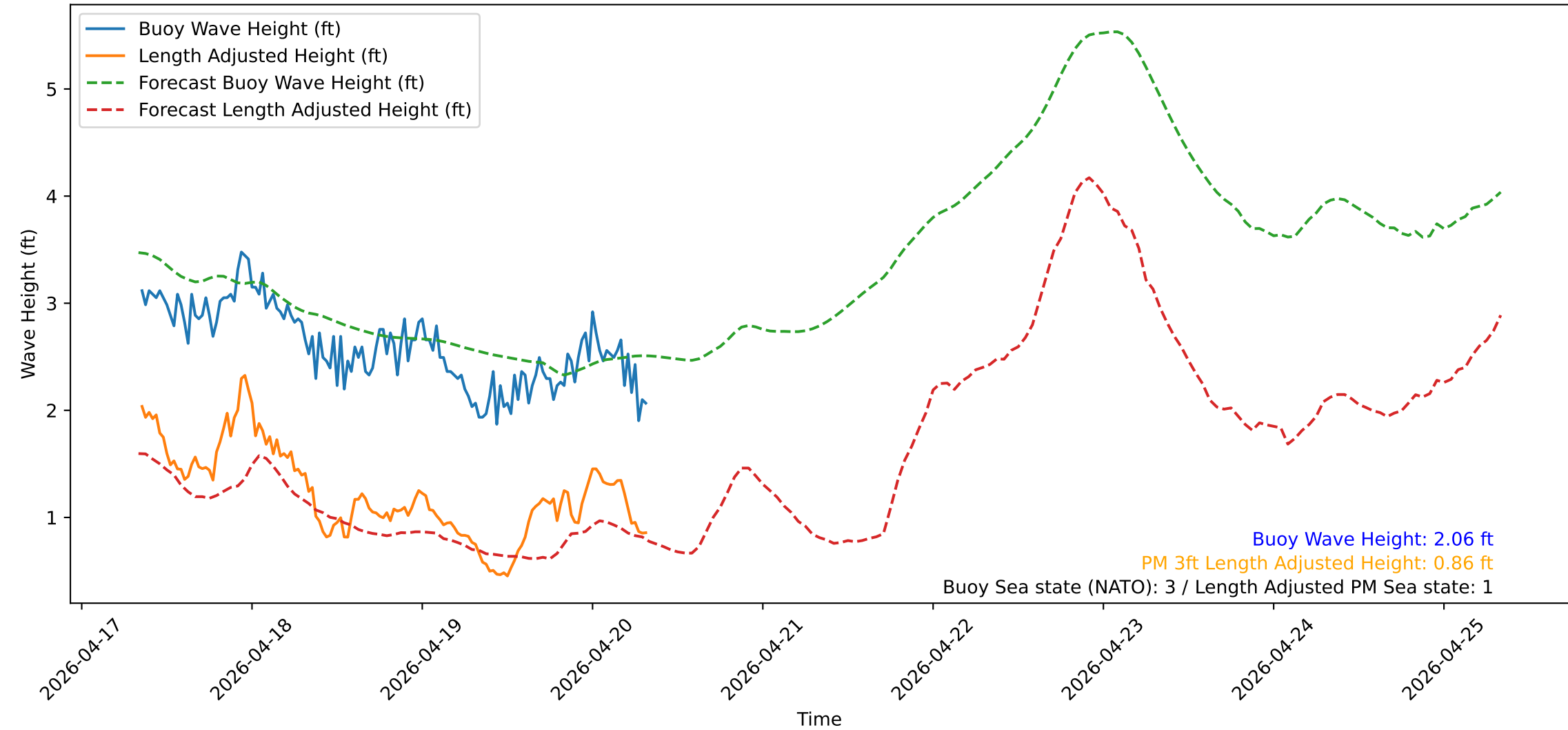
Wave Heights over Time for Green Beach at 2026-04-20 08:21:14
