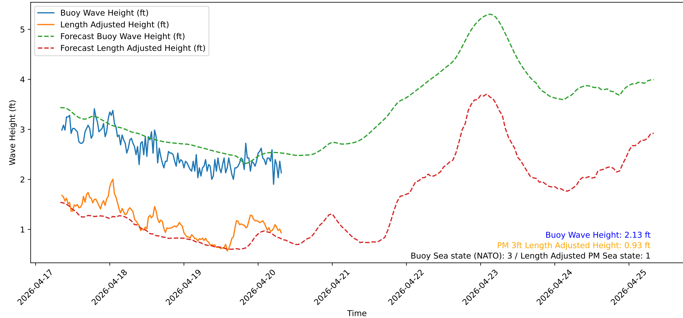
Wave Heights over Time for Oceanside Harbor at 2026-04-20 08:20:31
