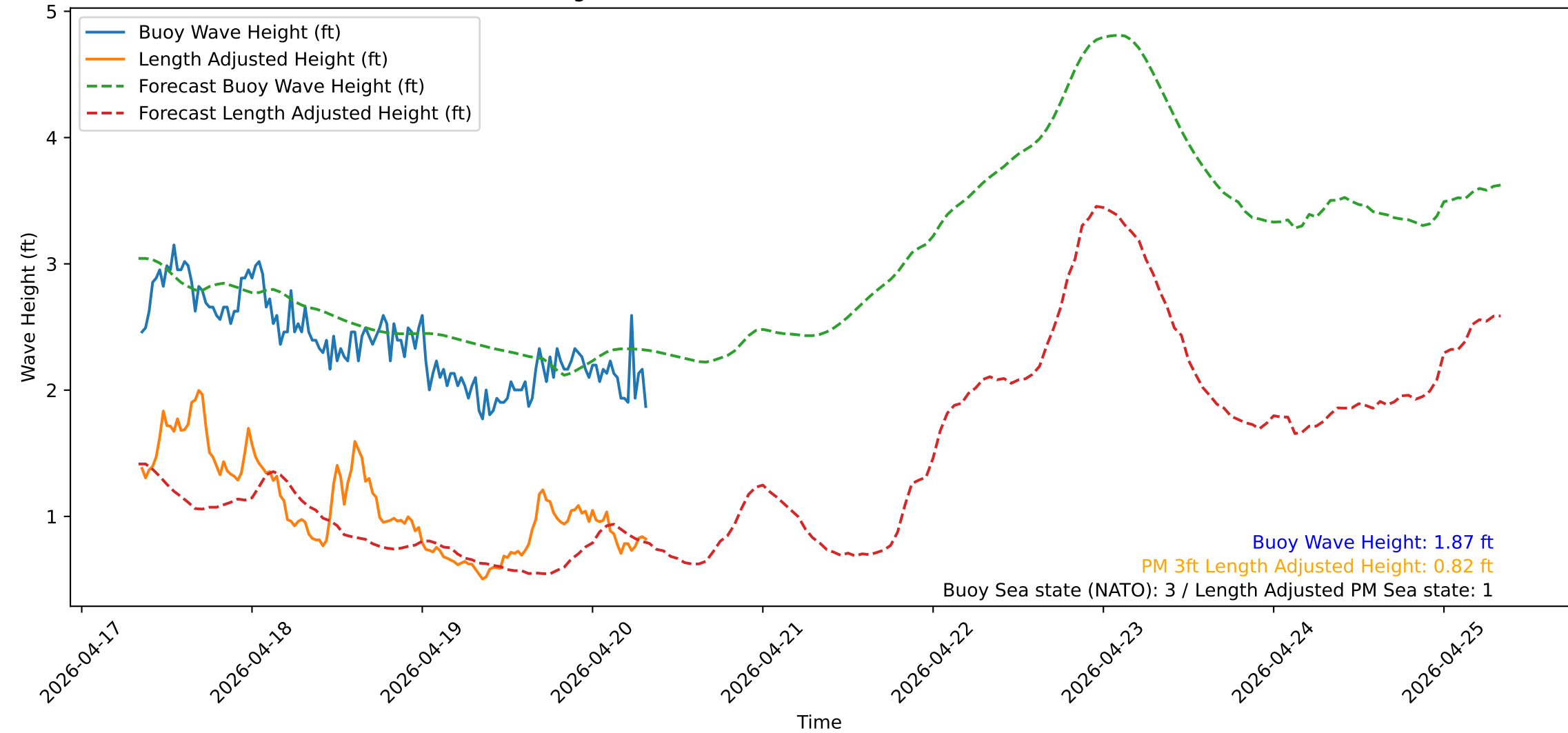
Wave Heights over Time for Red Beach at 2026-04-20 08:20:52
