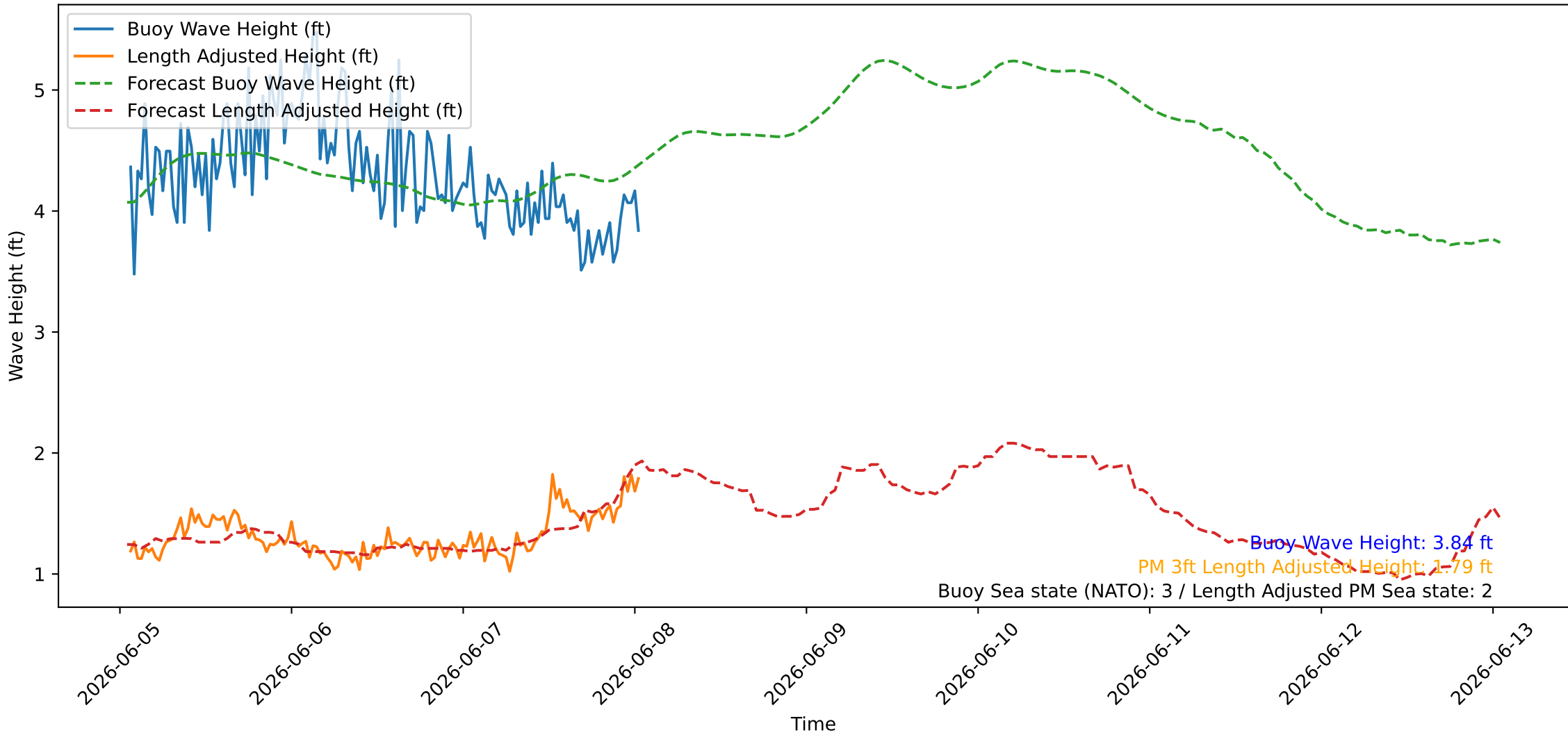
Wave Heights over Time for Oceanside Harbor at 2026-06-08 01:20:26
