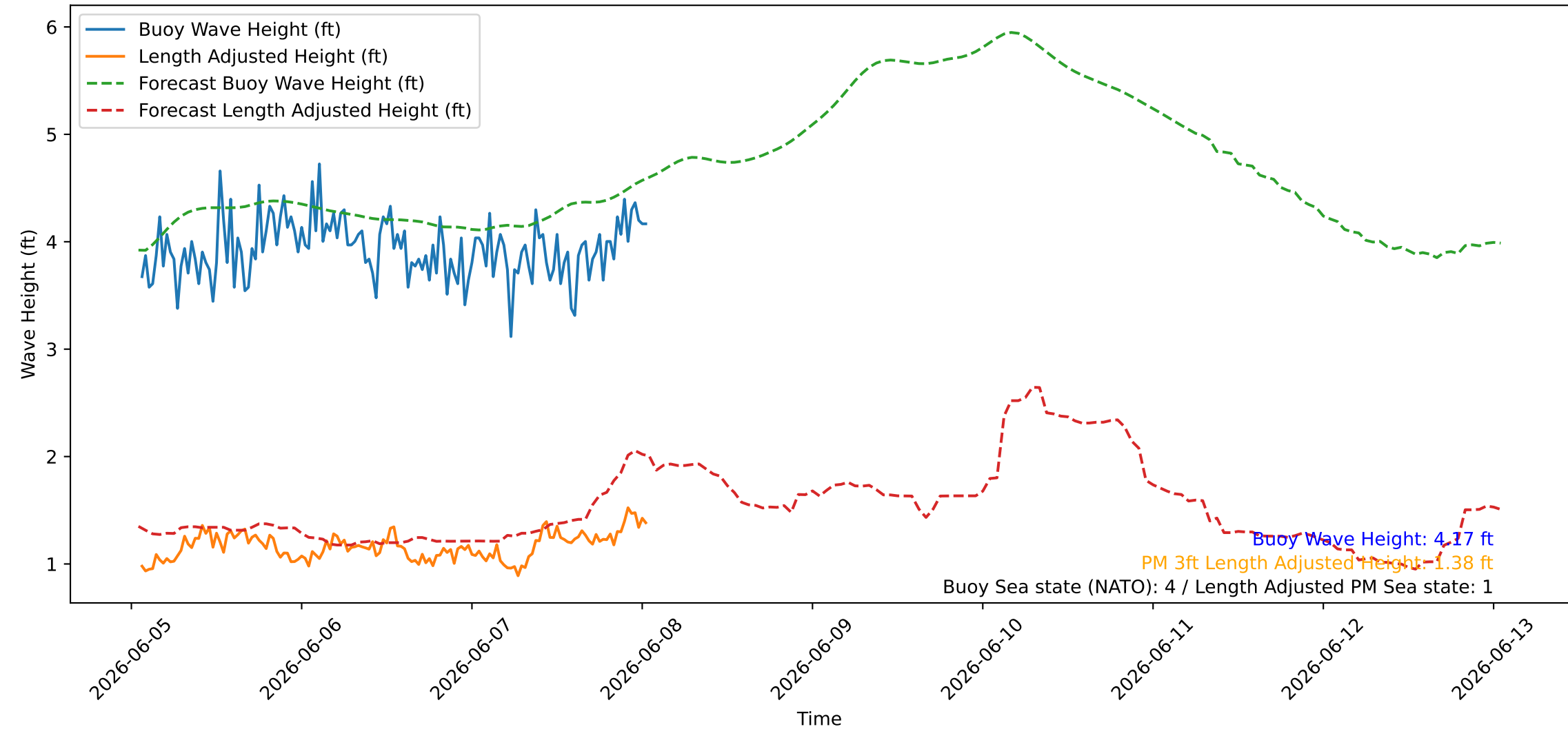
Wave Heights over Time for Green Beach at 2026-06-08 01:21:09
