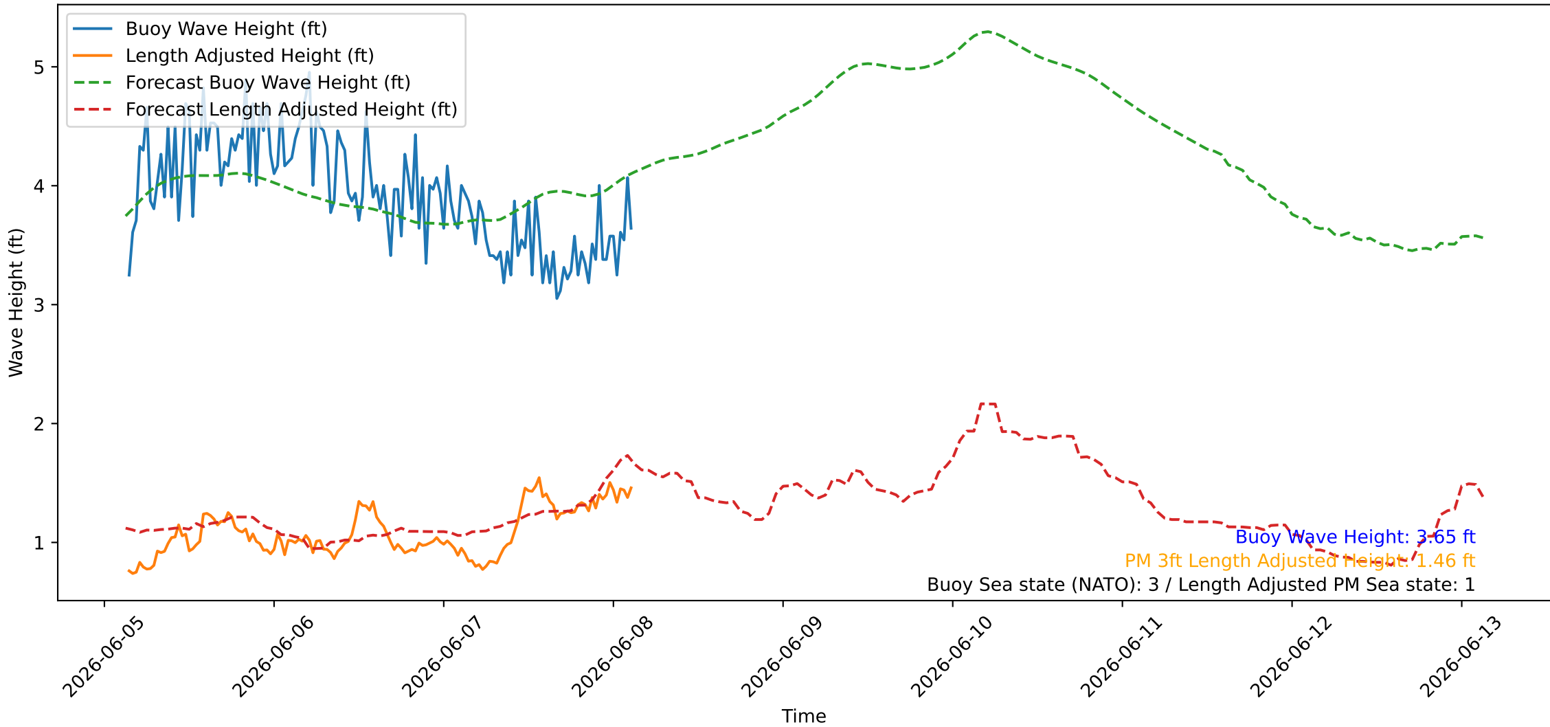
Wave Heights over Time for Red Beach at 2026-06-08 03:20:47
