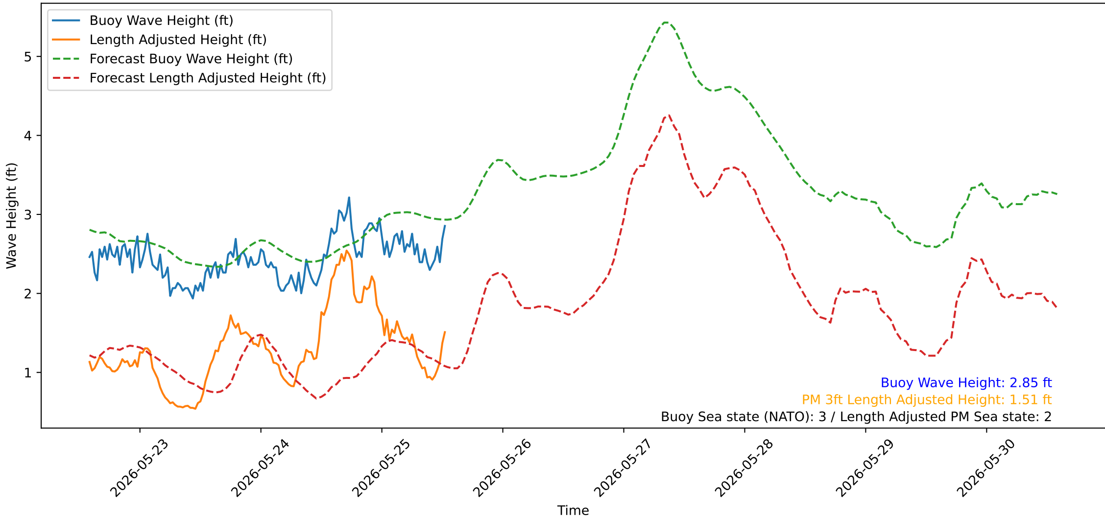
Wave Heights over Time for Red Beach at 2026-05-25 13:30:50
