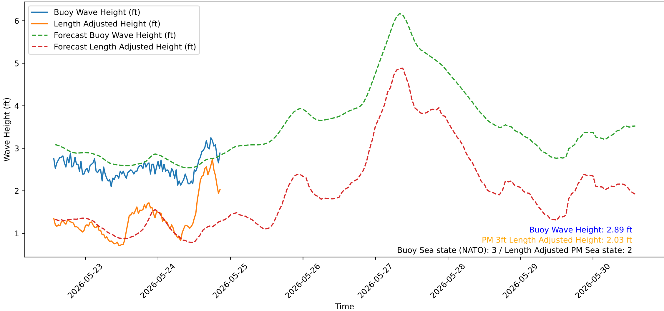
Wave Heights over Time for Oceanside Harbor at 2026-05-25 13:30:30
