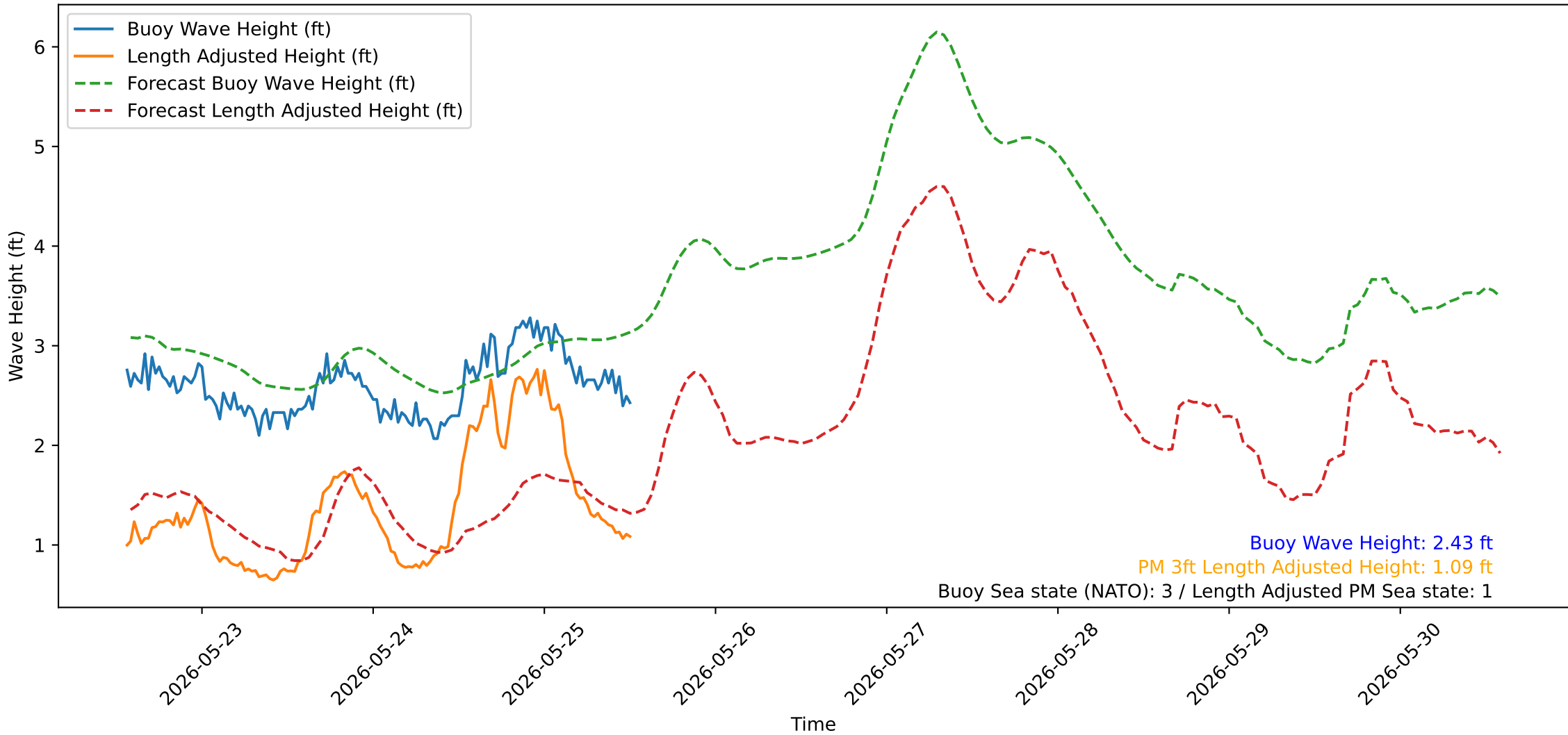
Wave Heights over Time for Green Beach at 2026-05-25 13:31:12
