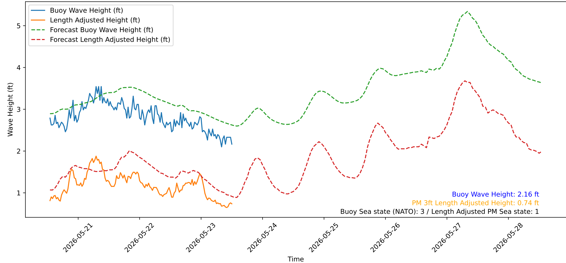
Wave Heights over Time for Green Beach at 2026-05-23 12:51:14
