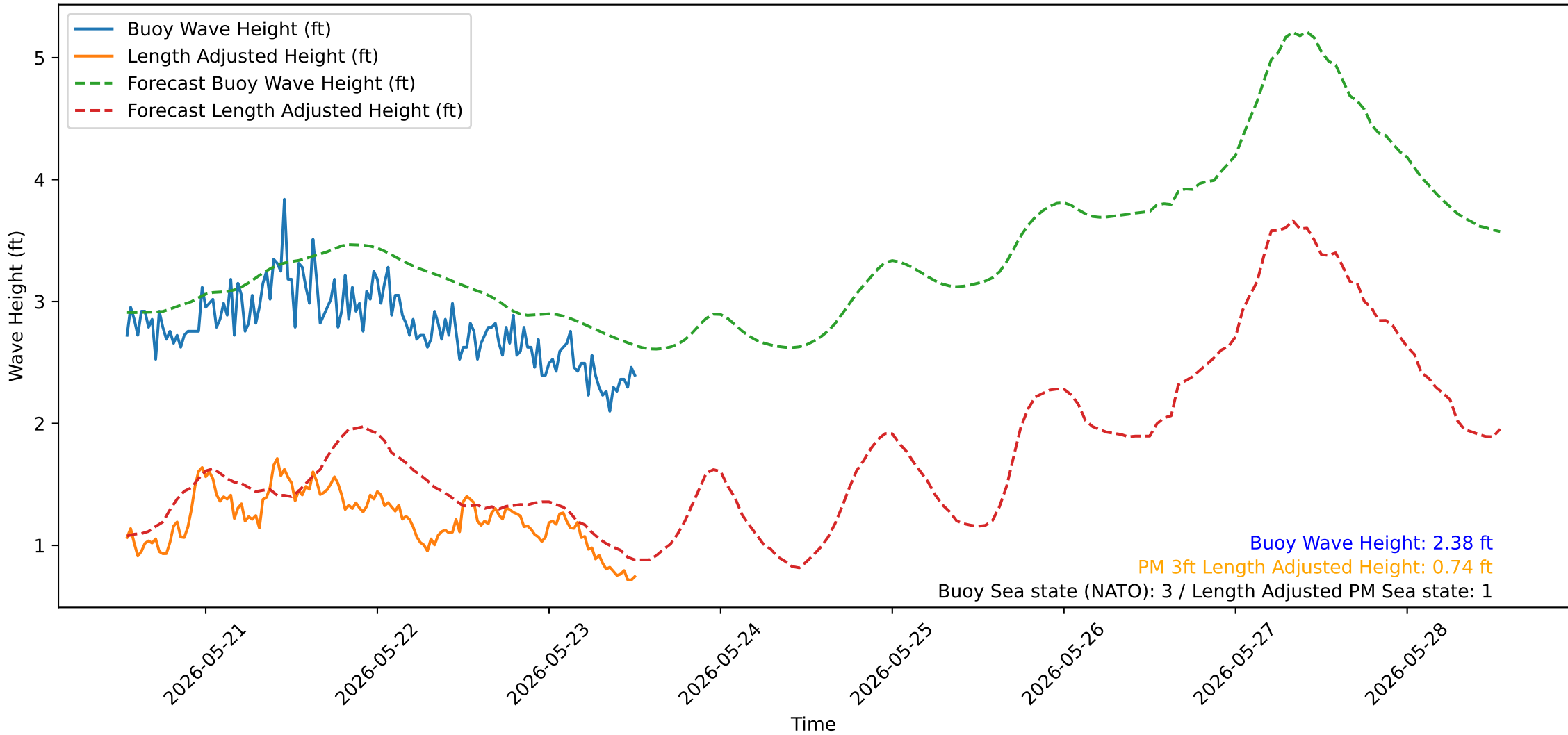
Wave Heights over Time for Oceanside Harbor at 2026-05-23 12:50:31
